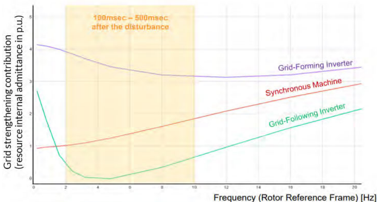
Figure 23: Resource characterization results from a series of detailed electromagnetic transient (EMT) simulations using detailed models. Image source: Telos Energy
