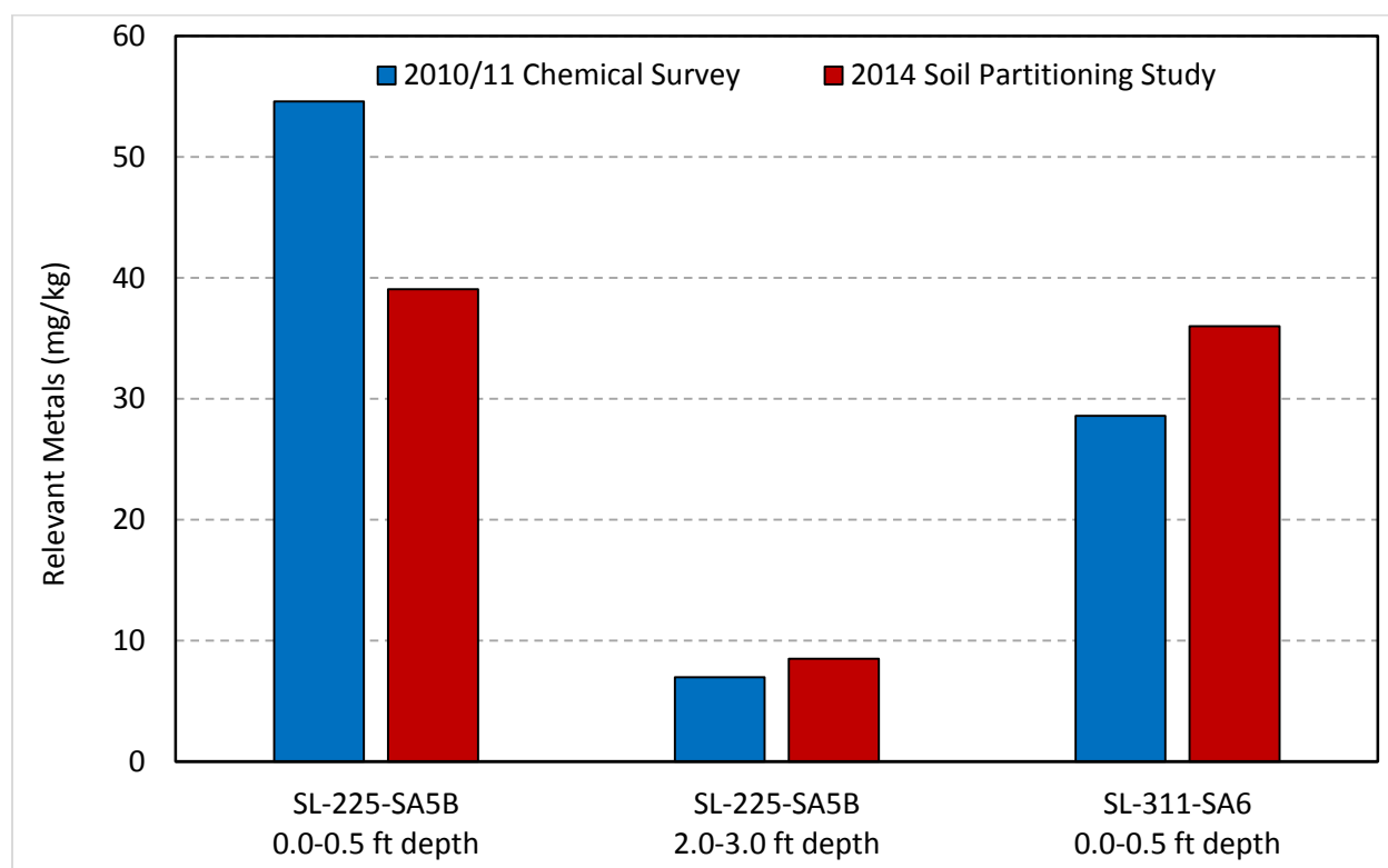
Figure 6.7 Change in Relevant Metals Concentration from 2010/2011 Soil Sampling Event to 2014 Soil Partition Study
