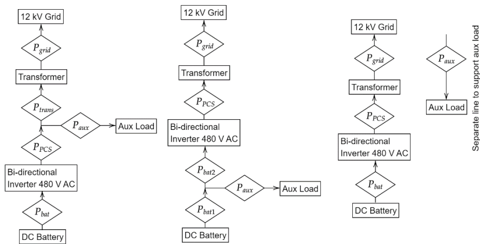
Figure 1. Example cases (1 to 3, left to right) of power meter layouts.
