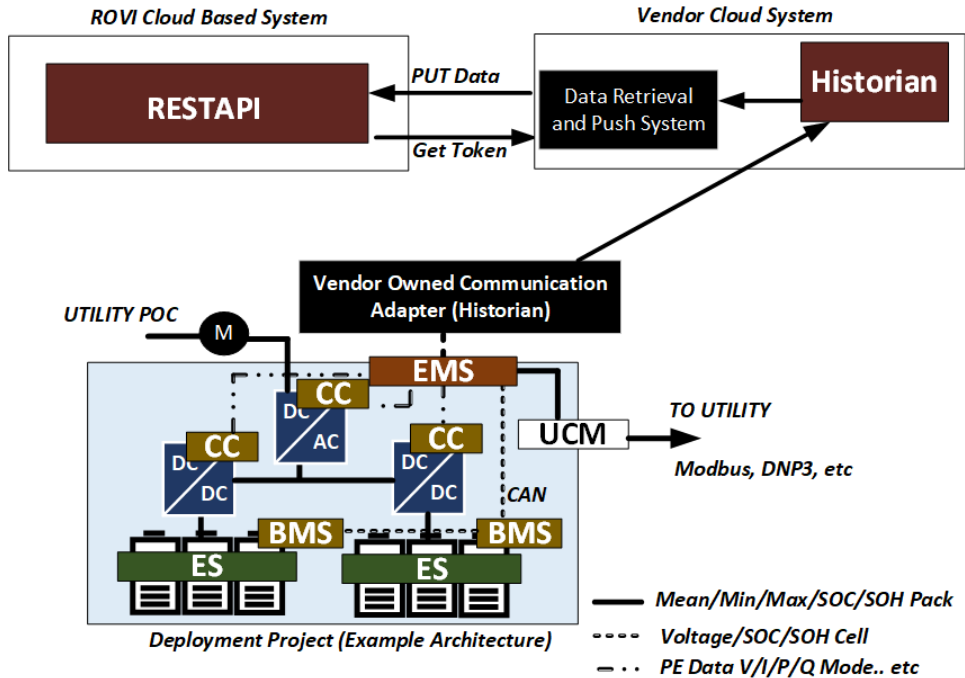
Figure 3. ROVI connects to existing vendor cloud services.
