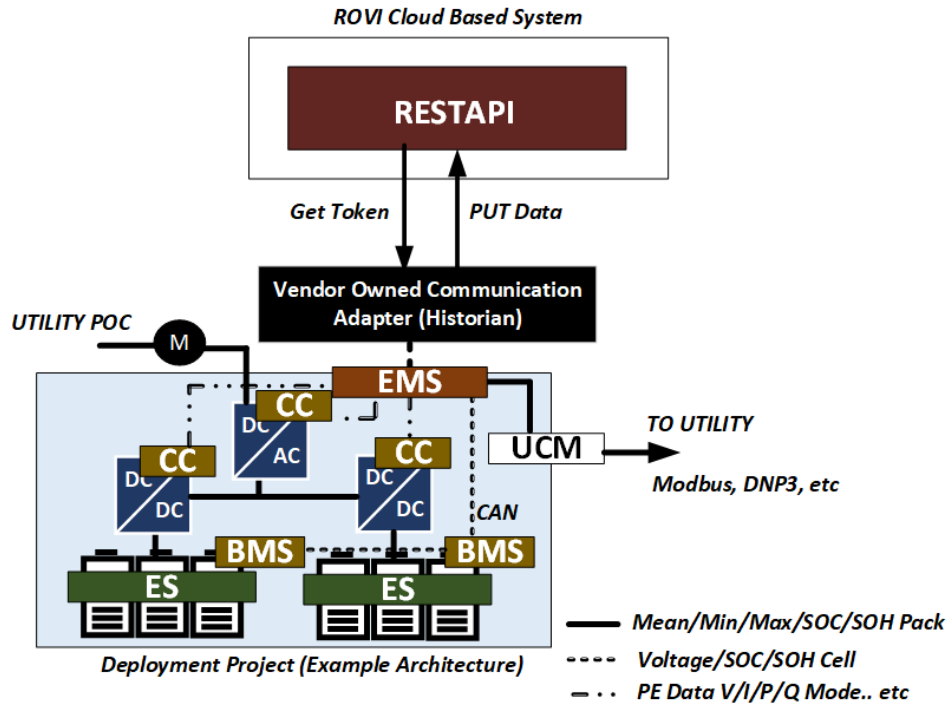
Figure 2. ROVI connects to existing vendor communication adapter.
