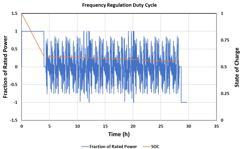
Figure 8. Protocol for frequency regulation.
