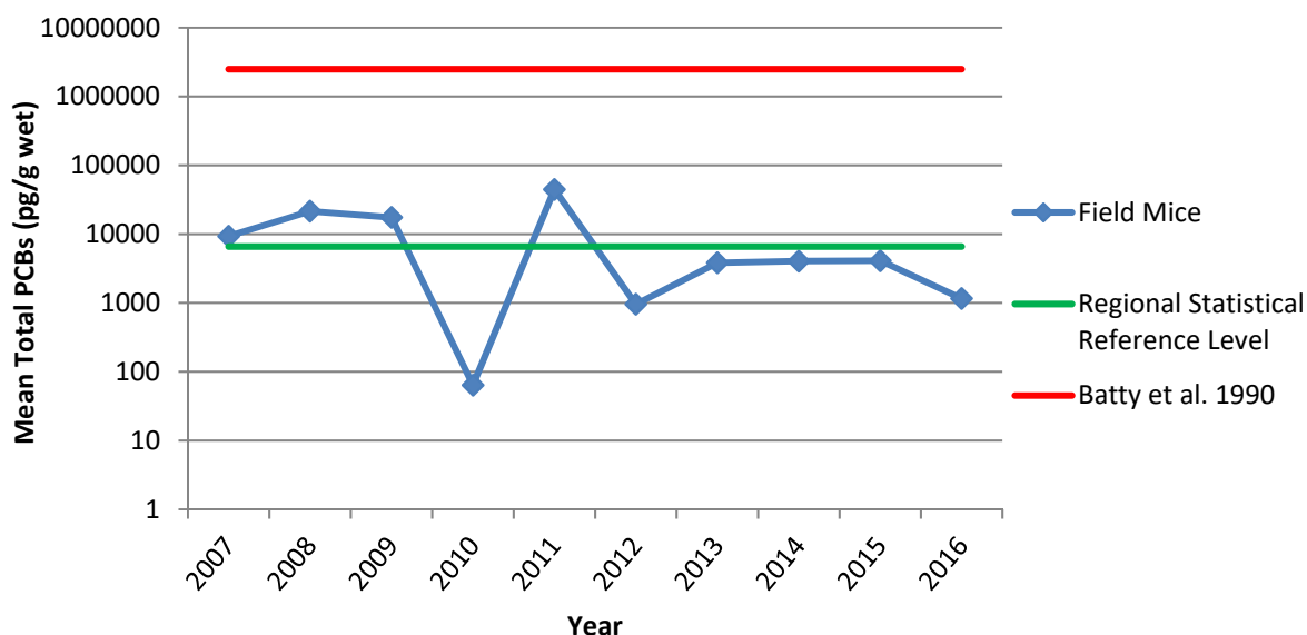
Figure 7-20 Mean total PCB concentrations in whole-body field mouse samples collected on the upstream side of the Pajarito Canyon flood-retention structure from 2007 to 2016 compared with the regional statistical reference level and the mean level of an affected population from Batty et al. (1990). Note the logarithmic scale on the vertical axis.
