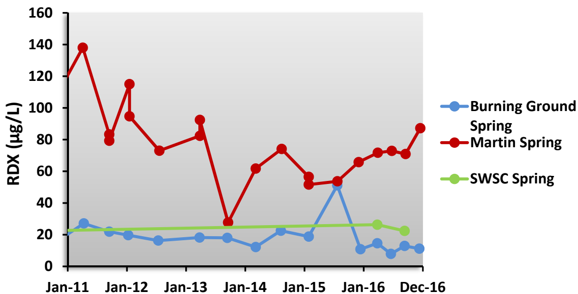
Figure 5-17 RDX concentrations in springs in Cañon de Valle and Martin Spring Canyon
