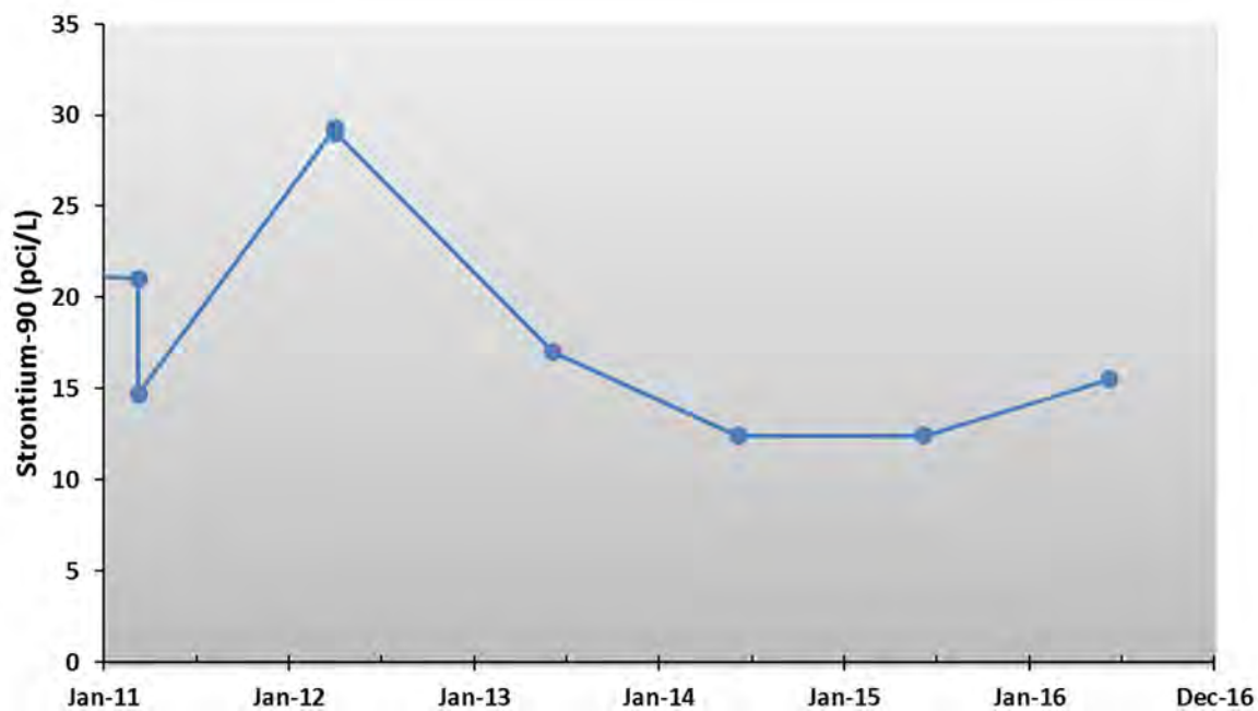
Figure 5-24 Strontium-90 activities at alluvial monitoring well LAO-3a
