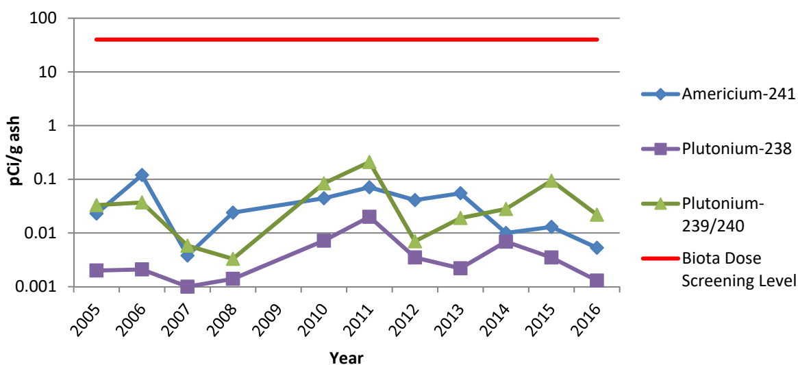
Figure 7-17 Americium-241, plutonium-238, and plutonium-239/240 activities in composite whole-body field mouse samples ( n > 5 ) collected on the upstream side (retention basin) of the Los Alamos Canyon weir from 2005 to 2016 compared with the biota dose screening level. Note the logarithmic scale on the vertical axis.
