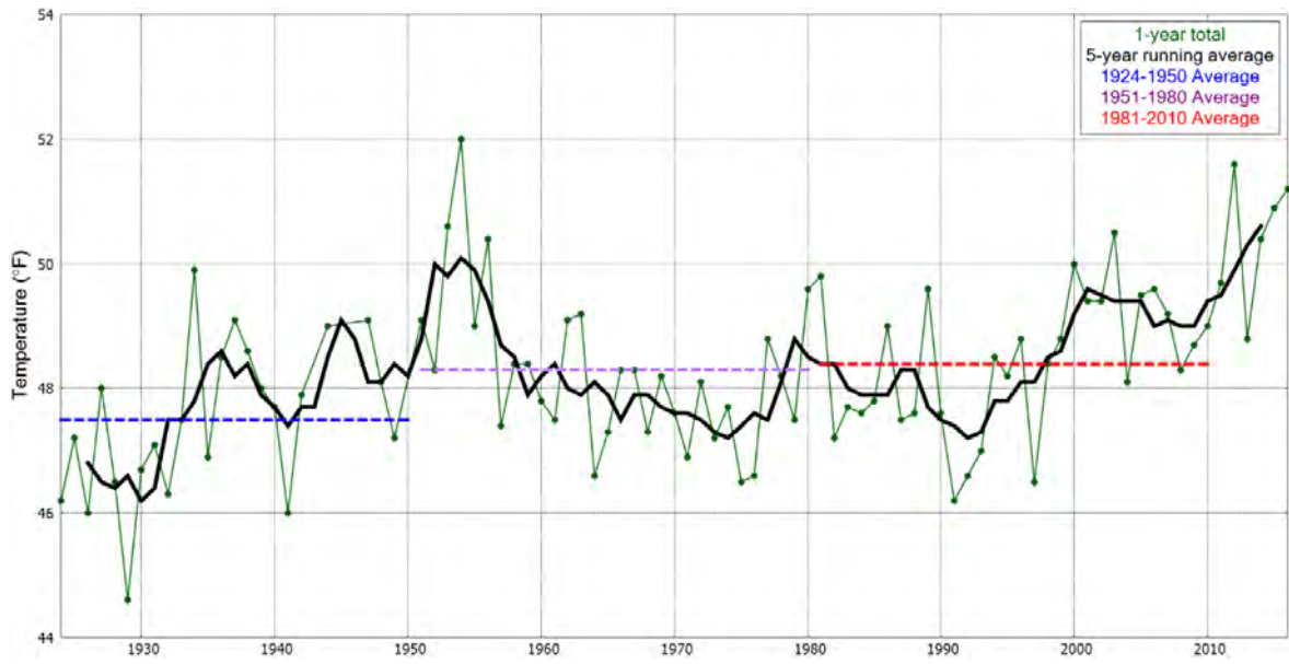
Figure 4-10 Temperature history for Los Alamos
