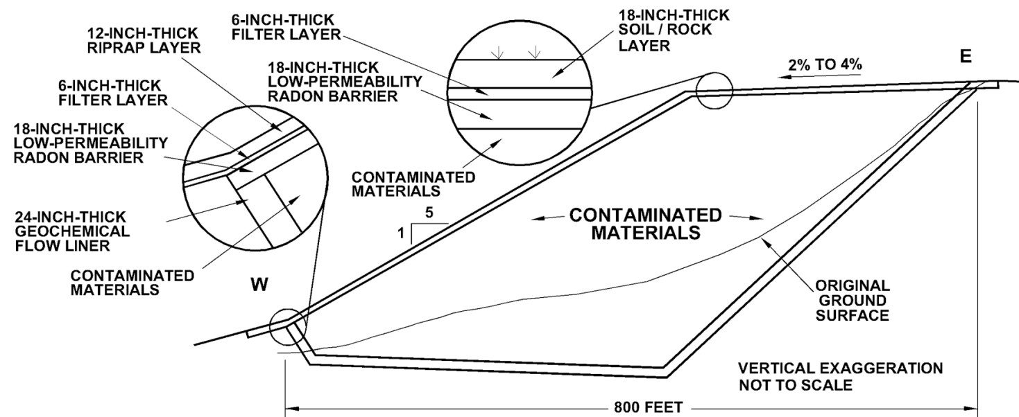
West-east cross section of the Lakeview disposal cell.
