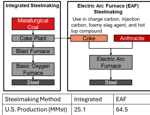
Figure 1. Coal use in integrated steelmaking and electric arc furnace steelmaking processes. 2023 production data from USGS.
