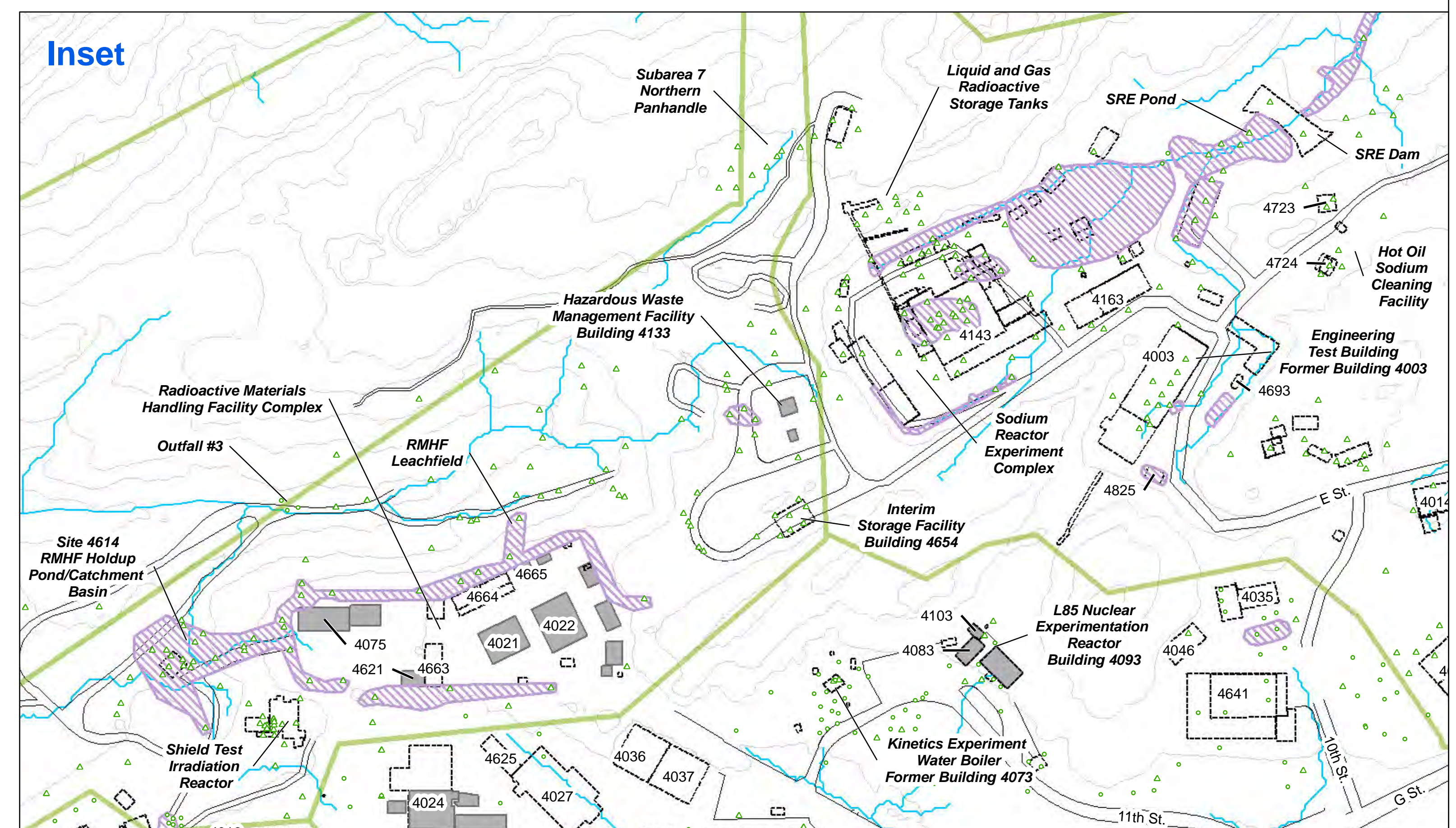
Figure 4.13 Americium-241 Round 1 and 2 Subsurface Soil and Sediment Results Santa Susana Field Laboratory Area IV and NBZ Radiological Study
