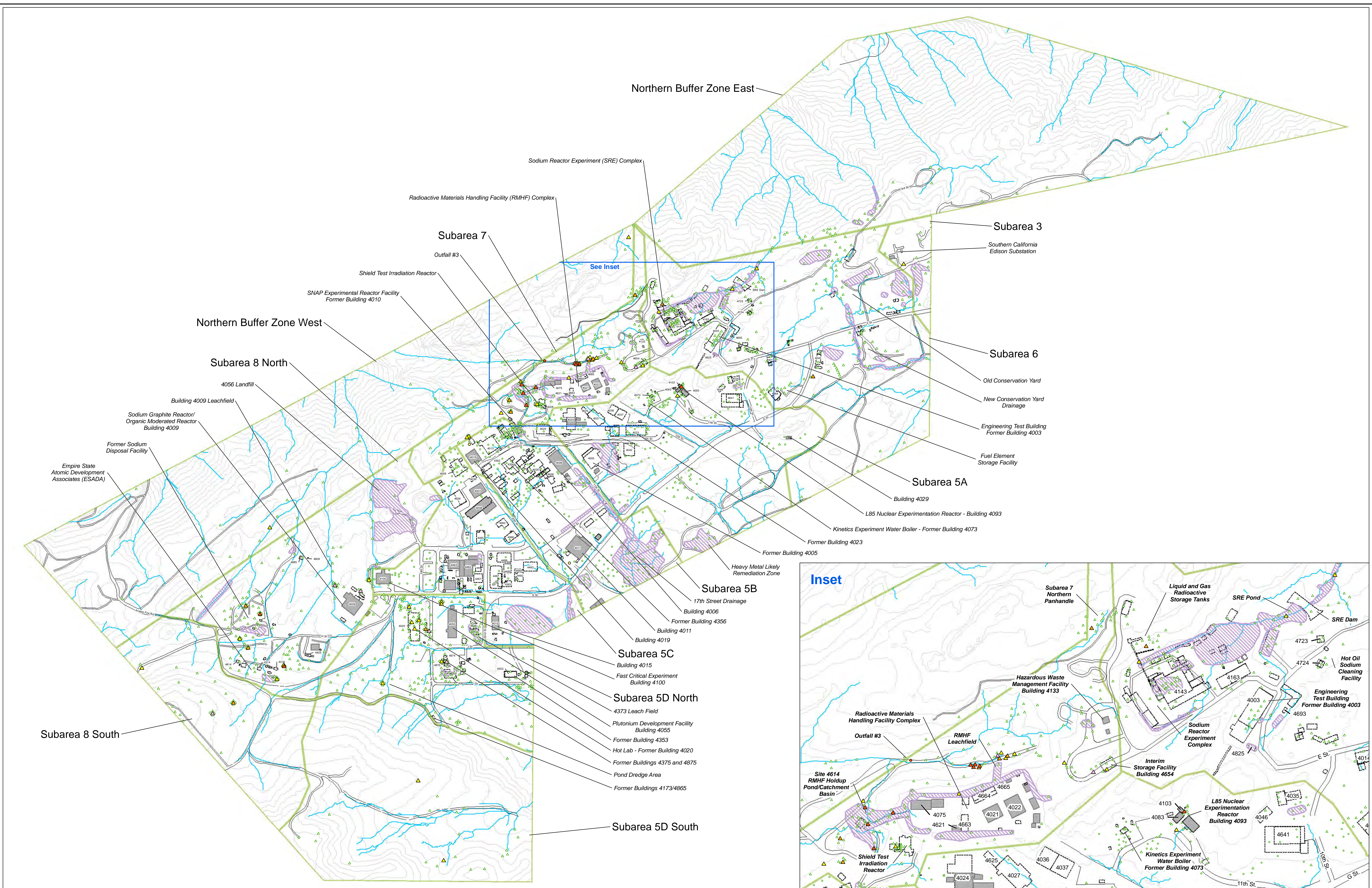
Figure 4.4 Strontium-90 Round 1 and 2 Subsurface Soil and Sediment Results Santa Susana Field Laboratory Area IV and NBZ Radiological Study
