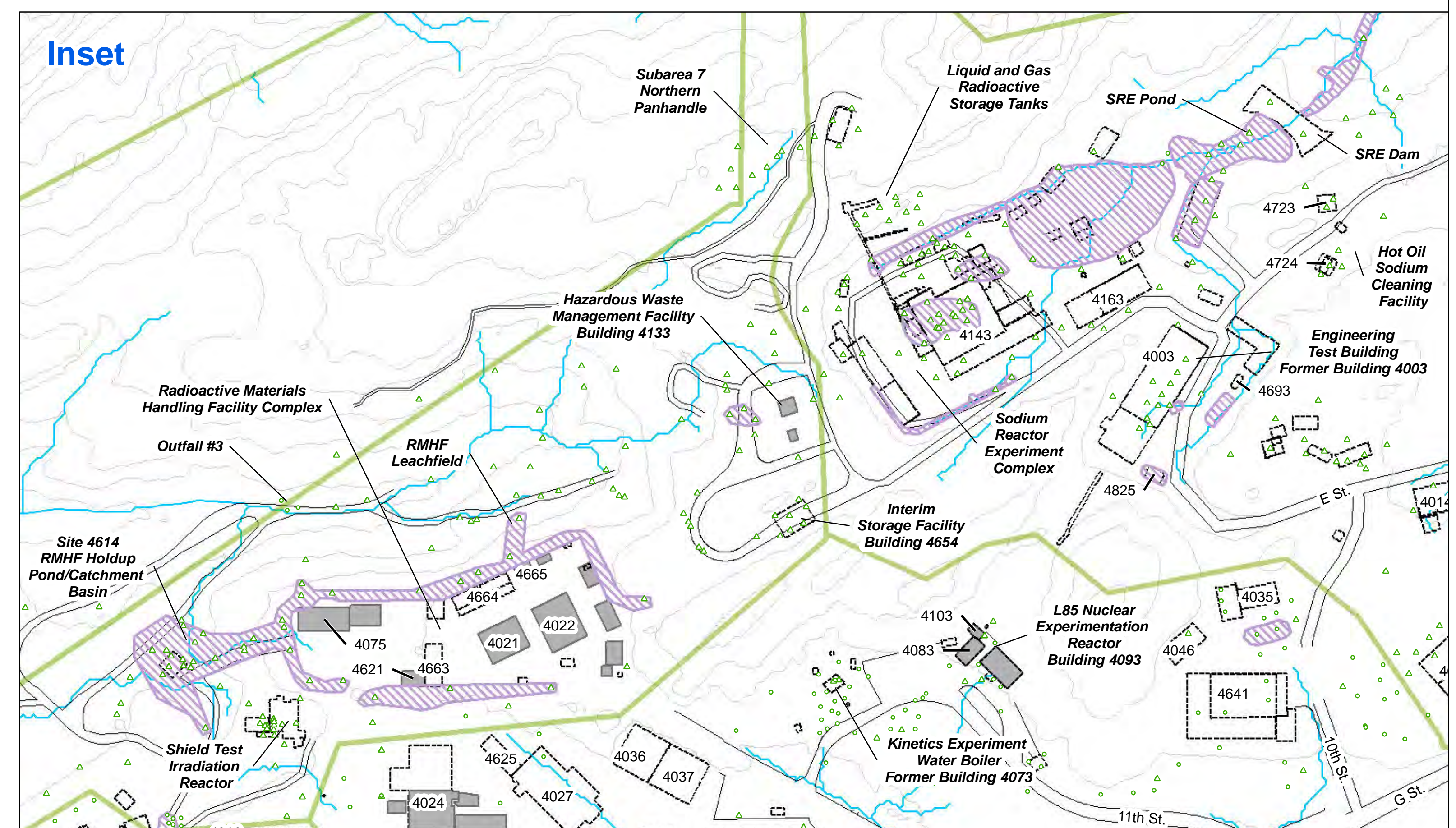
Figure 4.15 Curium-243/244 Round 1 and 2 Subsurface Soil and Sediment Results Santa Susana Field Laboratory Area IV and NBZ Radiological Study
