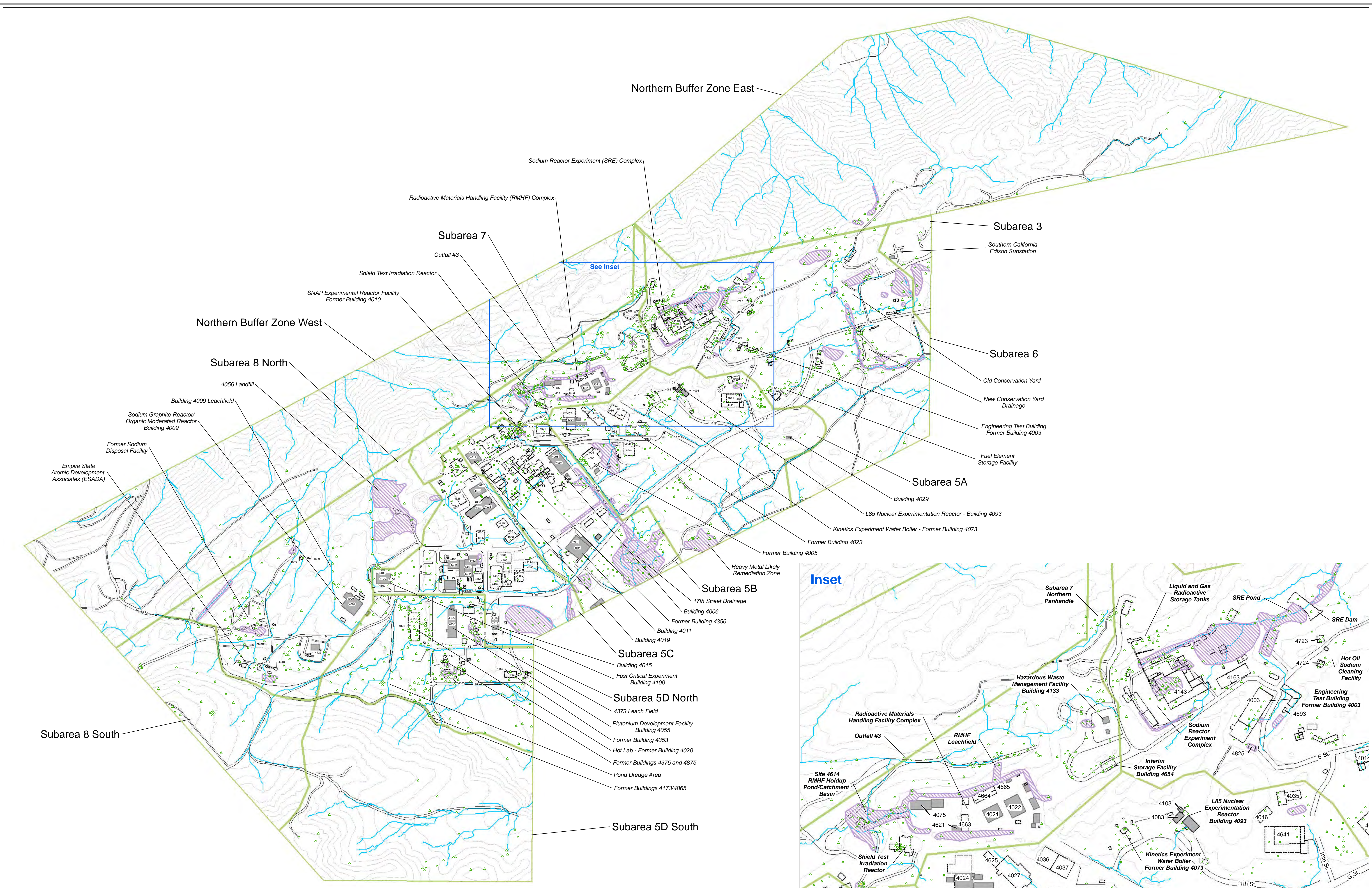
Figure 4.10 Europium-152 Round 1 and 2 Subsurface Soil and Sediment Results Santa Susana Field Laboratory Area IV and NBZ Radiological Study
