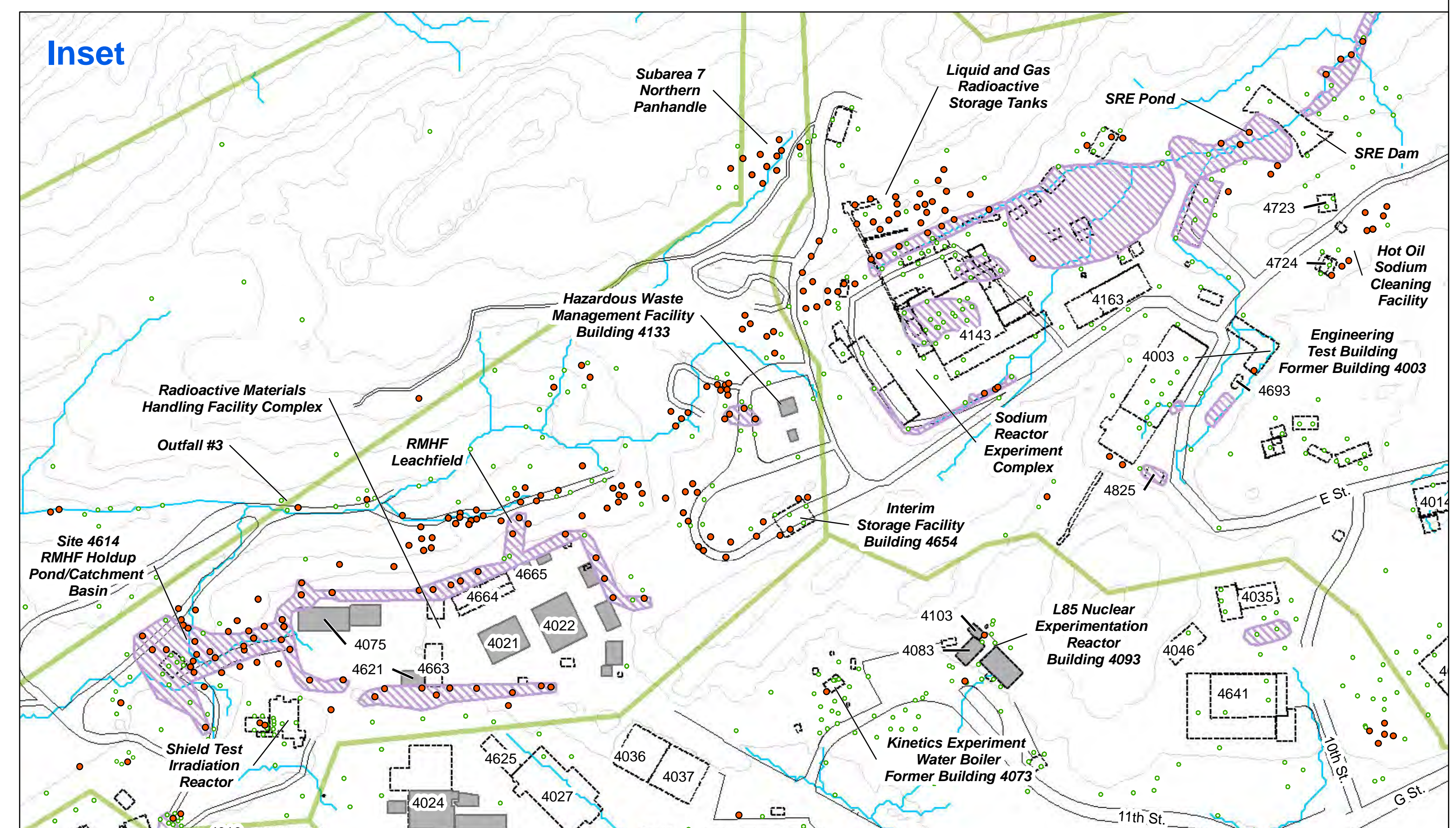
Figure 5.1 Select Radionuclides of Concern Round 1 and 2 Surface and Subsurface Soil and Sediment Results Santa Susana Field Laboratory Area IV and NBZ Radiological Study
