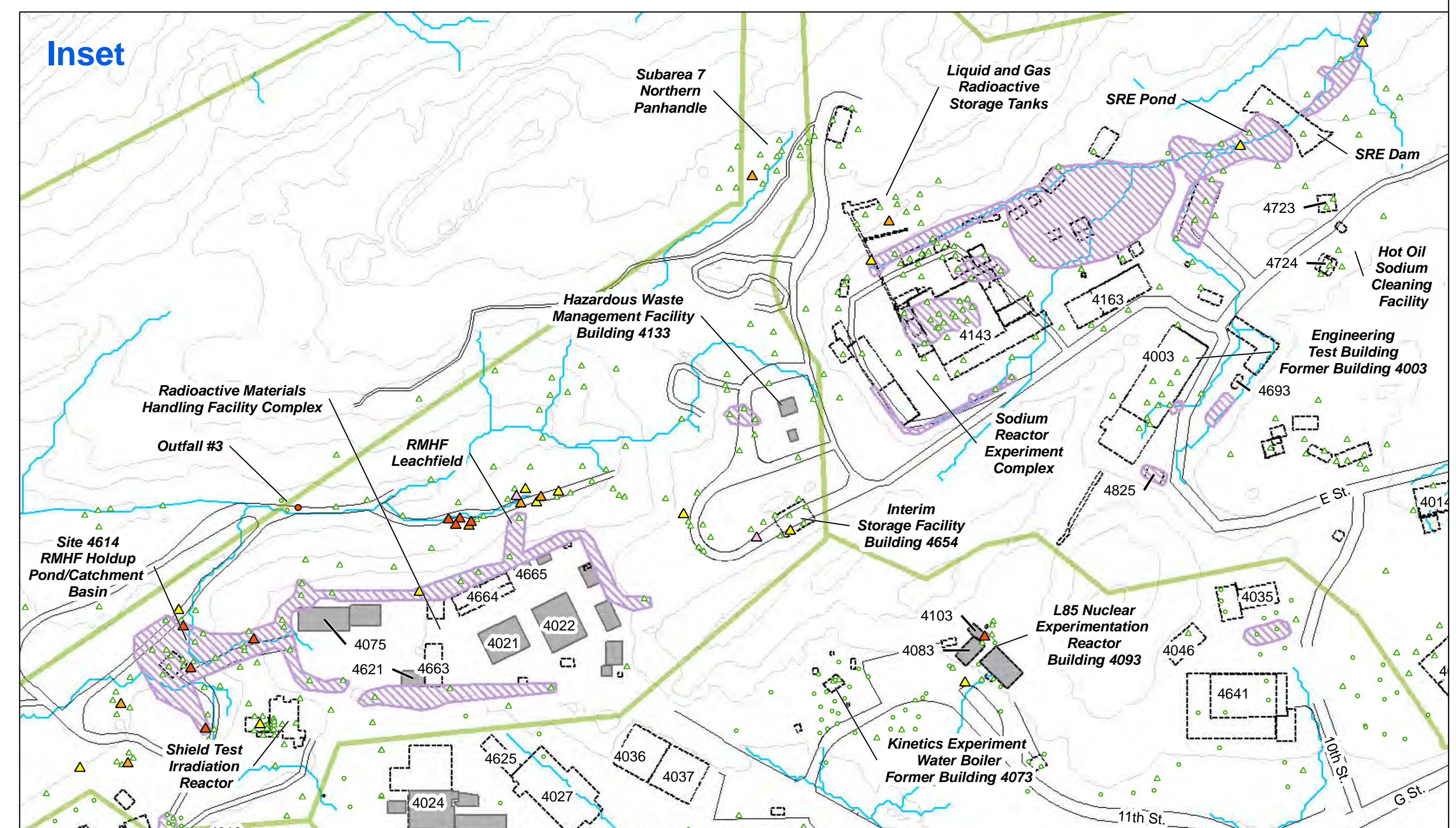
Figure 4.4 Strontium-90 Round 1 and 2 Subsurface Soil and Sediment Results Santa Susana Field Laboratory Area IV and NBZ Radiological Study
