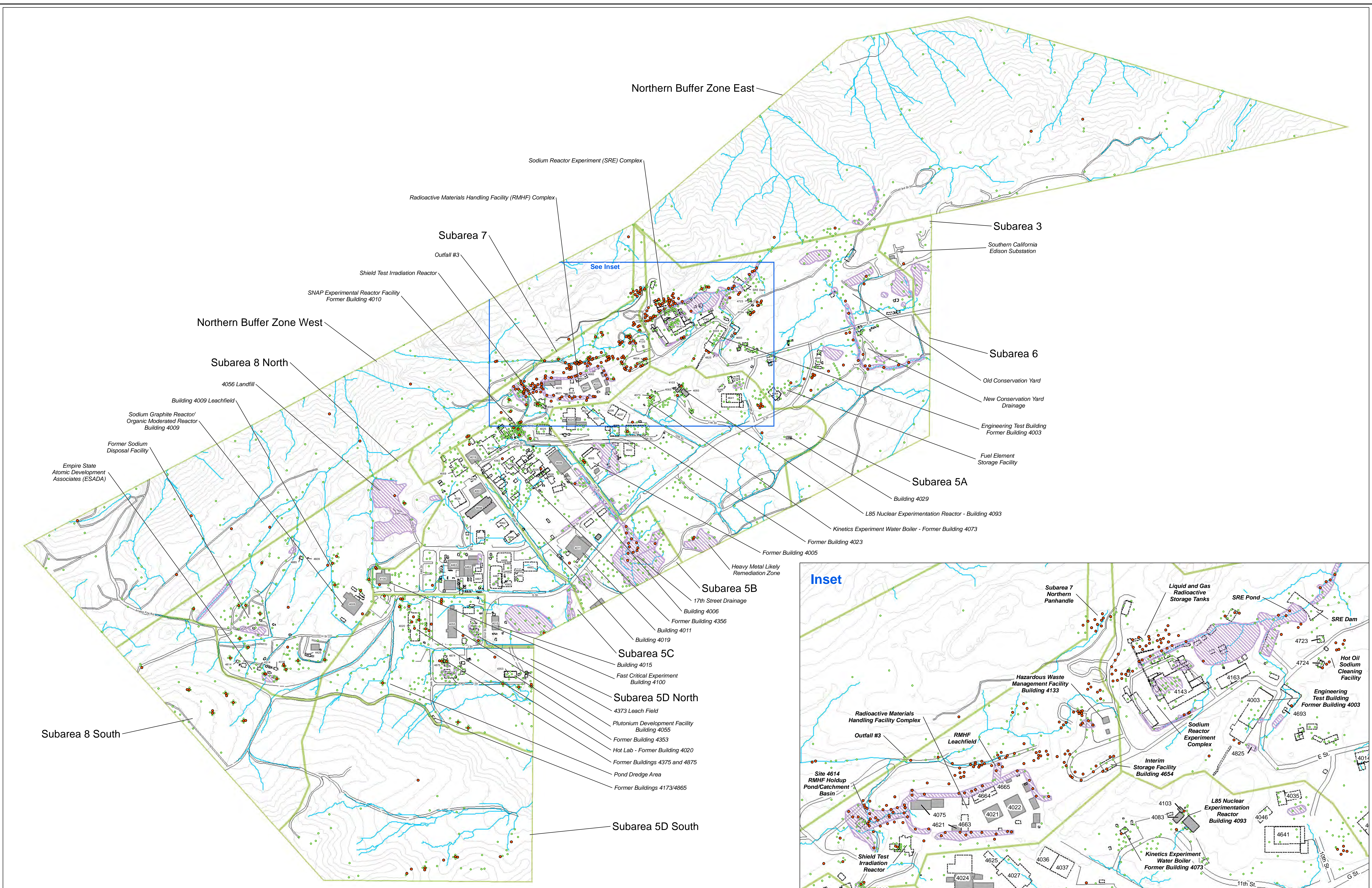
Figure 5.1 Select Radionuclides of Concern Round 1 and 2 Surface and Subsurface Soil and Sediment Results Santa Susana Field Laboratory Area IV and NBZ Radiological Study
