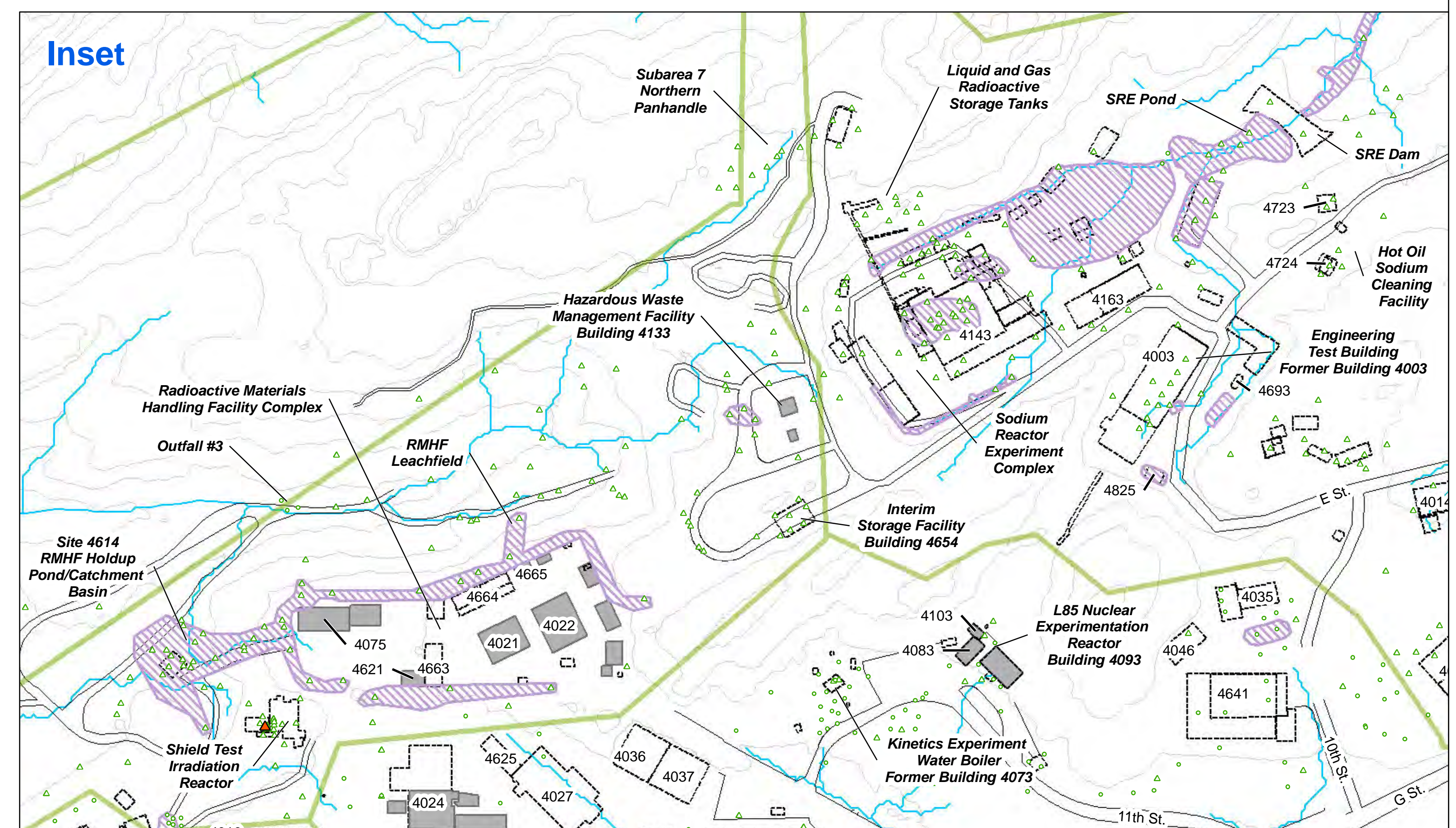
Figure 4.6 Plutonium-239/240 Round 1 and 2 Subsurface Soil and Sediment Results Santa Susana Field Laboratory Area IV and NBZ Radiological Study
