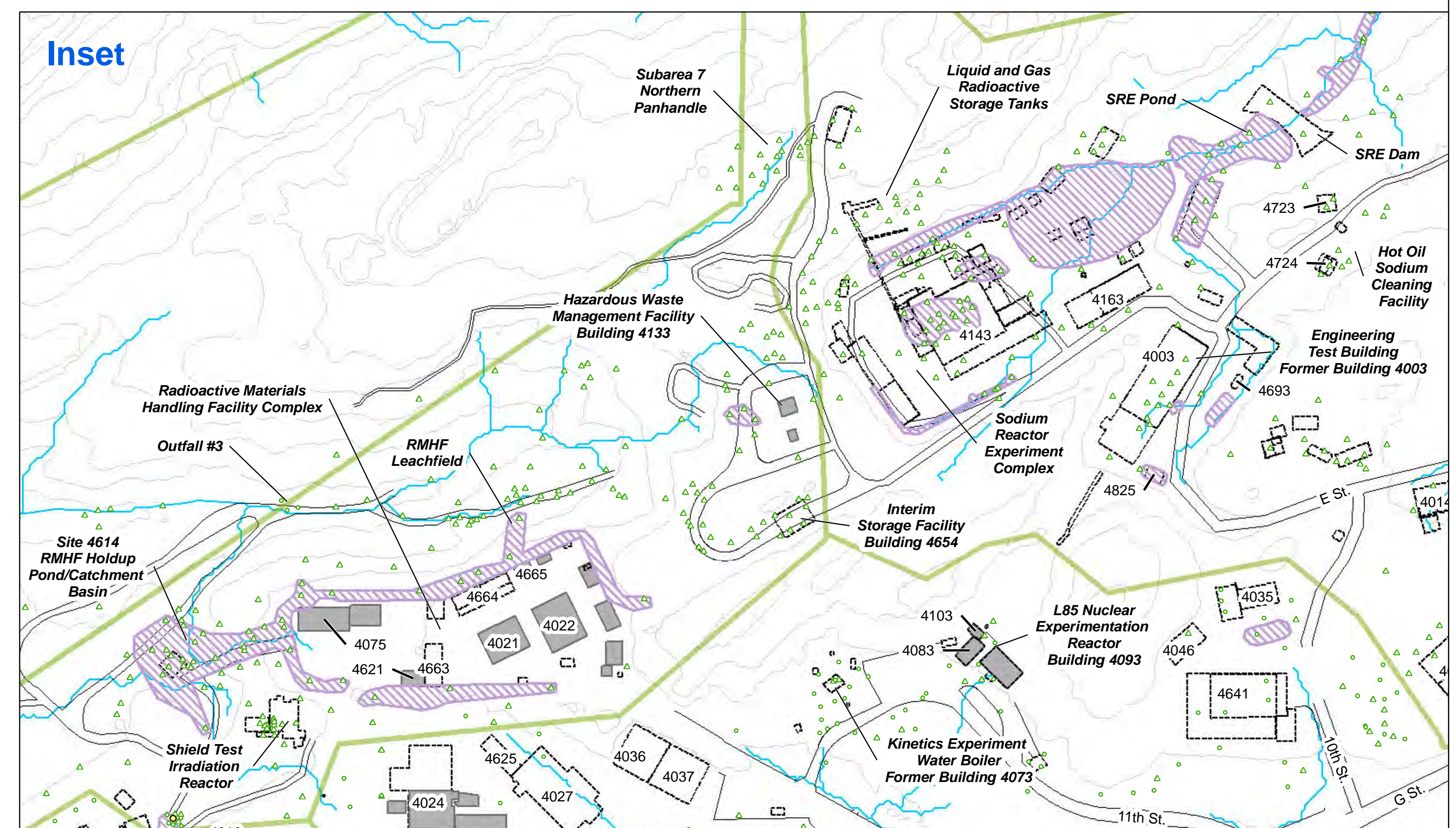
Figure 4.10 Europium-152 Round 1 and 2 Subsurface Soil and Sediment Results Santa Susana Field Laboratory Area IV and NBZ Radiological Study
