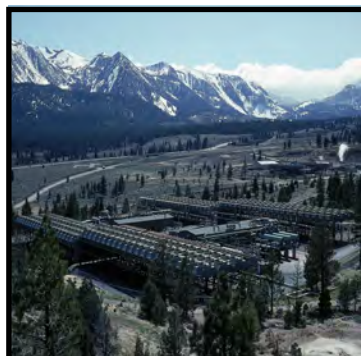
The Mammoth-Pacific geothermal power plants, in Mono County, California, draw on the natural geothermal resource close to the surface. Early DOE investments helped to harness this energy. Source: NREL
