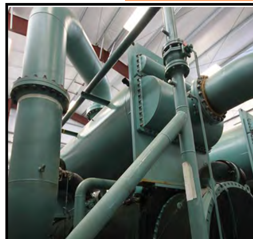
Energy Department industry partner Johnson Controls Inc. commissioned another 1.75 MW of geothermal energy at Oregon Institute of Technology in 2014. Source: Bill Goloski
