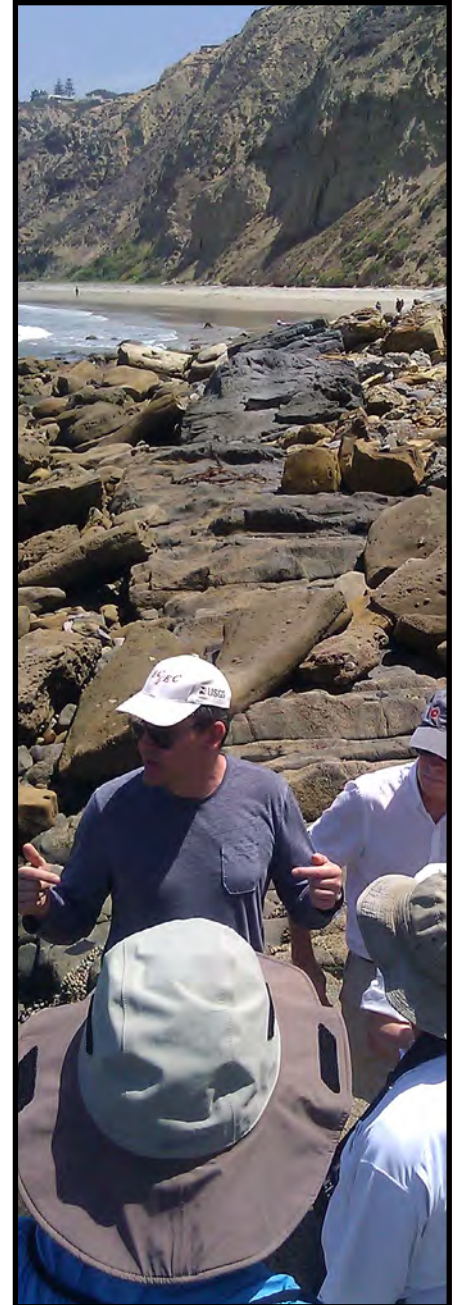
JASON study members stand on a basaltic dike exposure below the La Jolla cliffs while Professor Yuri Fialko of the Scripps Institution of Oceanography describes how its orientation is controlled by the stress field at the time of emplacement. Source: Benjamin Phillips
