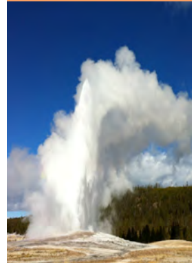
Old Faithful Geyser, Yellowstone. SOURCE: Laura Garchar
