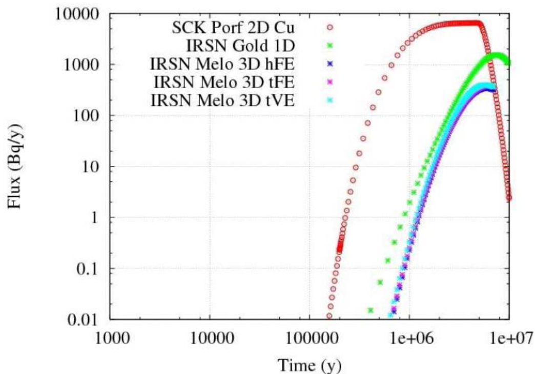
Figure 3.3-20. Np Activity Flux to Upper Aquifer–PAMINA Benchmark
