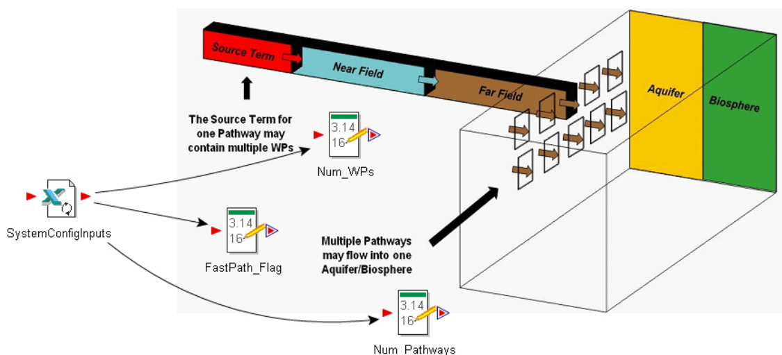
Figure 4-18. GoldSim GPAM System-Level Input Elements
