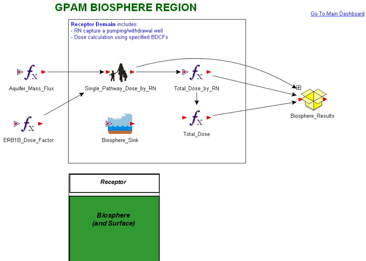
Figure 4-16. GoldSim GPAM Biosphere Region
