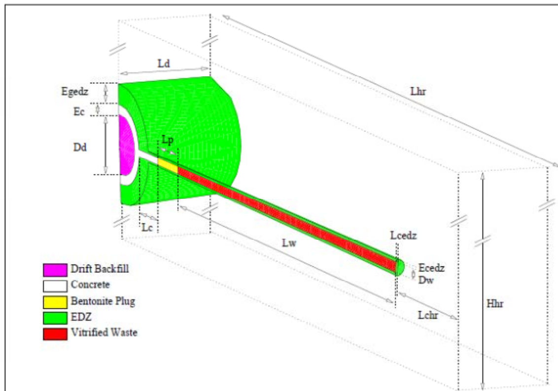
Figure 3.3-15. PAMINA Benchmark Configuration
