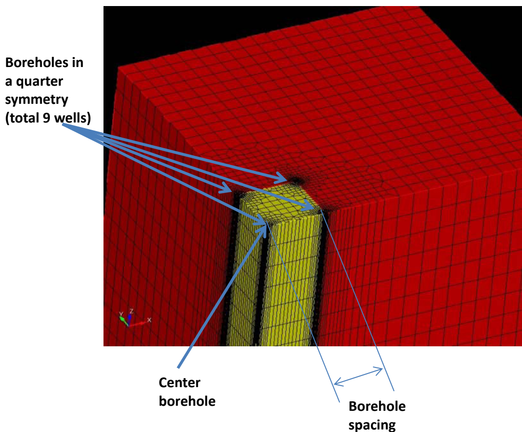
Figure 3.4-2. Mesh Used for Thermal-Hydrologic Simulations
