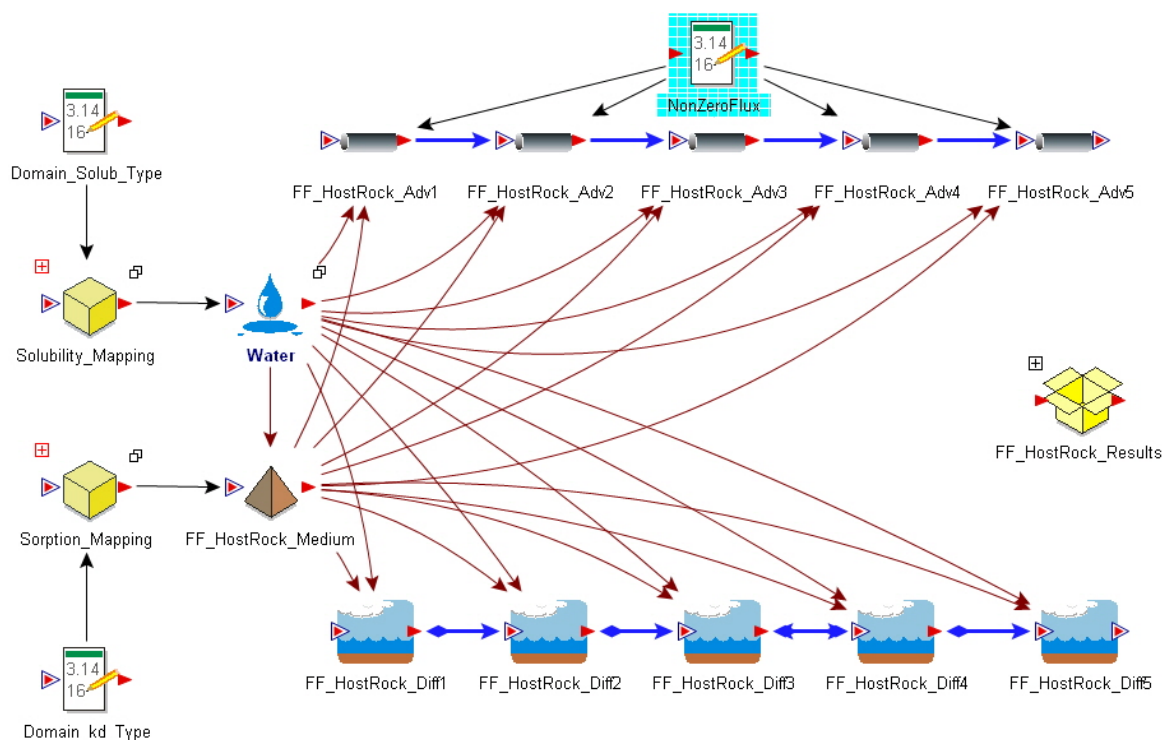
Figure 4-14. GoldSim GPAM Far-Field Host Rock Domain Elements
