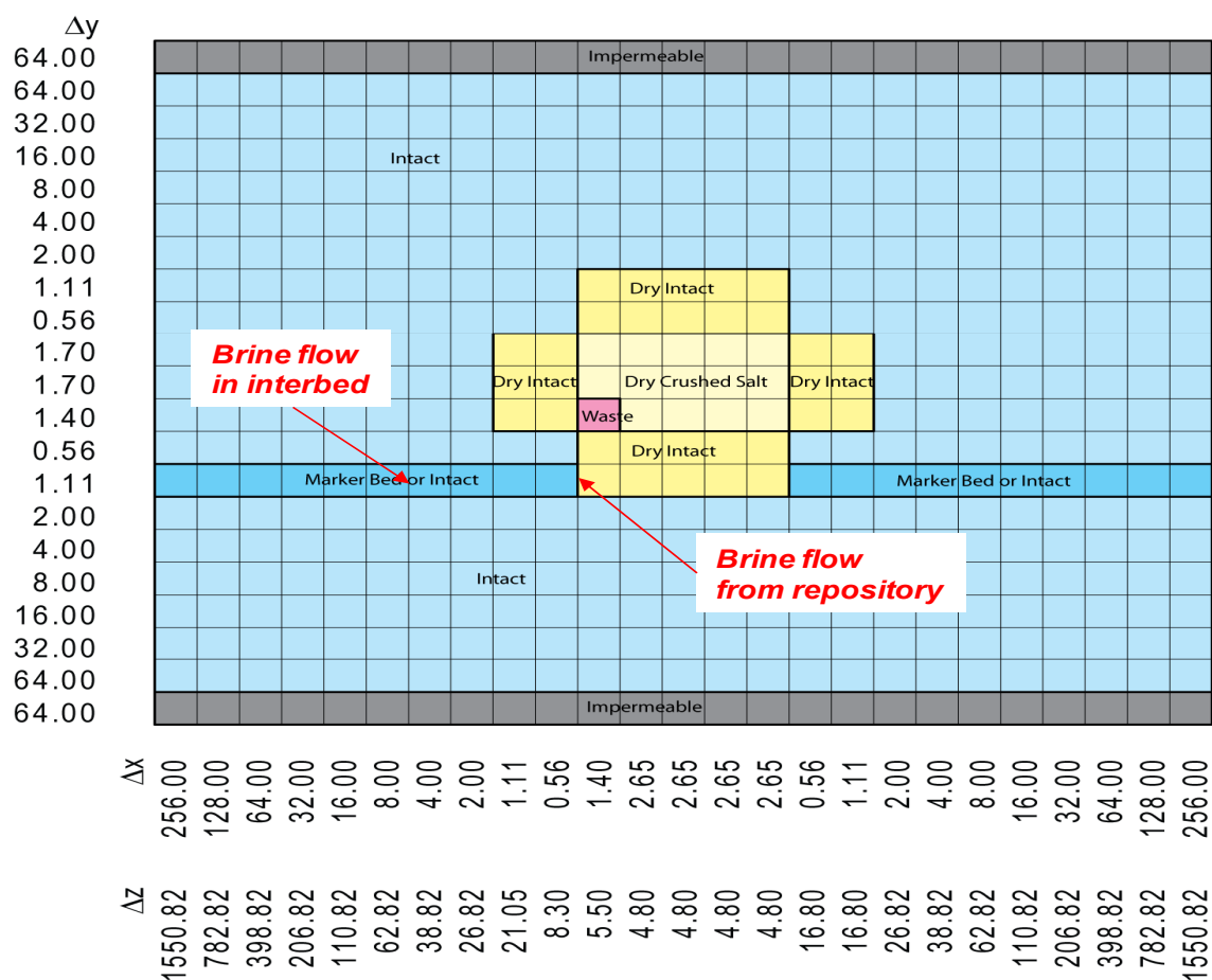
Figure 3.1-3. Long-term Brine Flow Grid Used in Analysis
