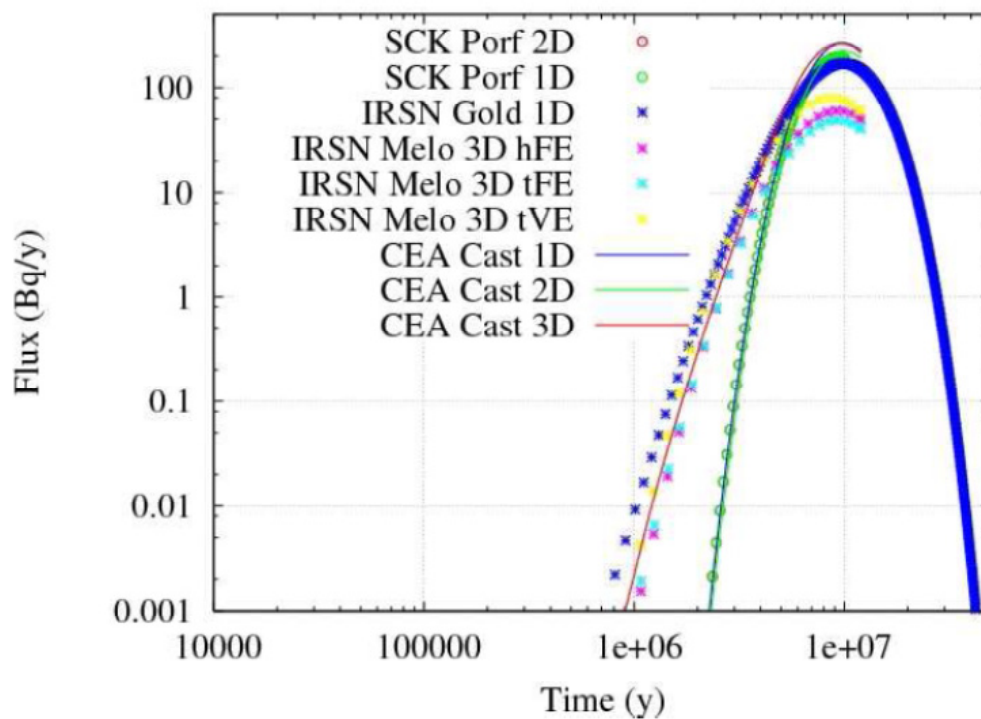
Figure 3.3-18. Cs Activity Flux to Upper Aquifer—PAMINA Benchmark
