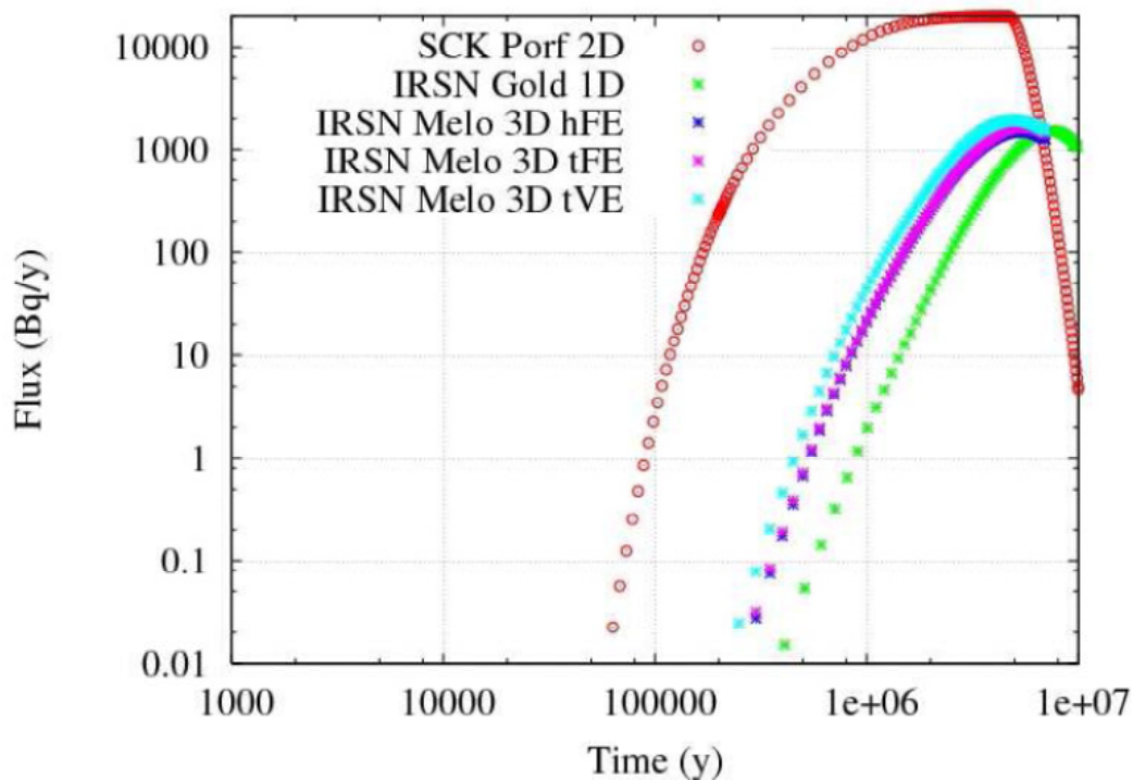
Figure 3.3-21. U Activity Flux to Upper Aquifer – PAMINA Benchmark
