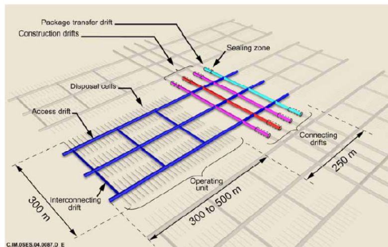
Figure 3.3-23. Andra Benchmark Configuration
