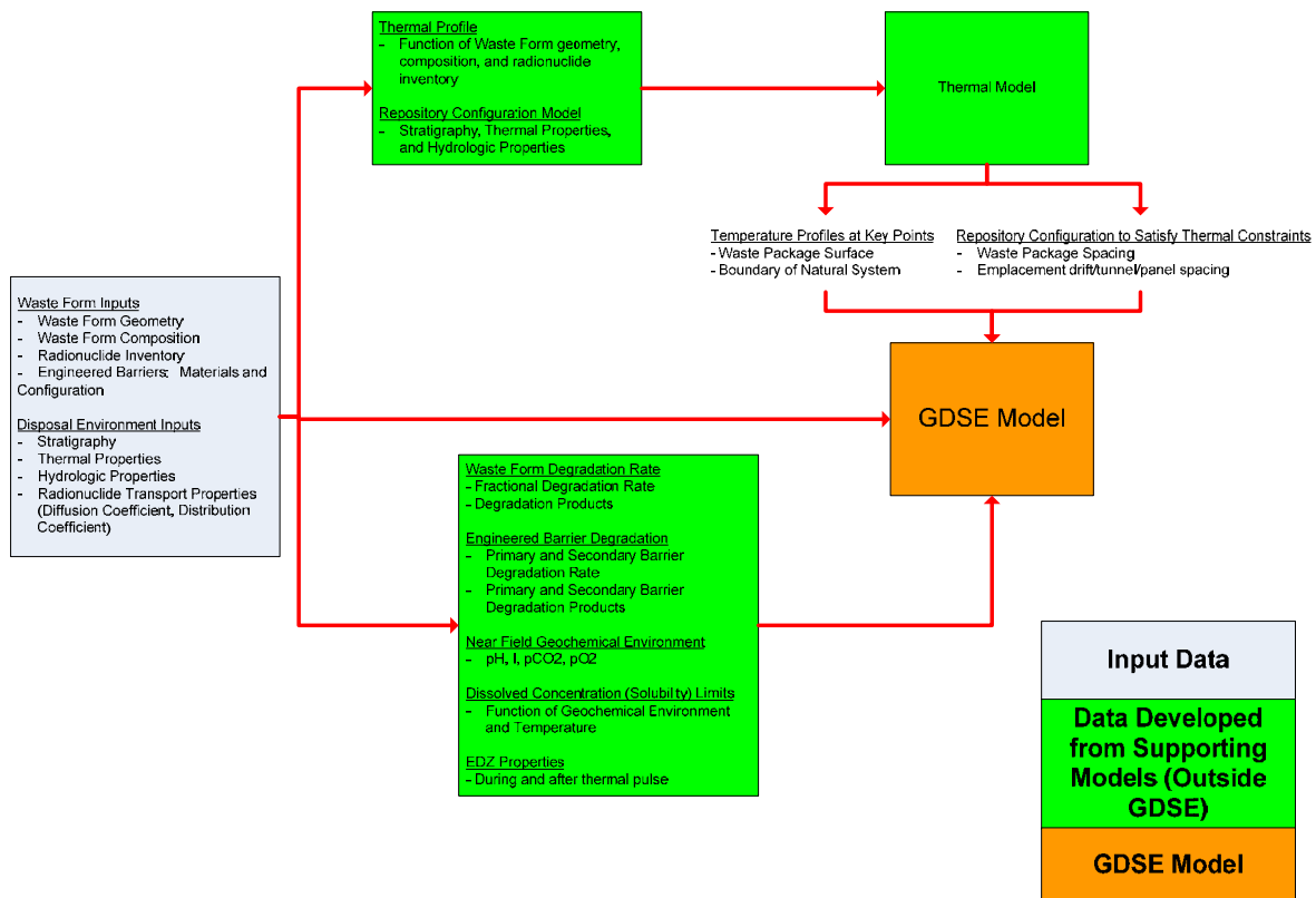
Figure 3.3-1. Clay GDS Model Structure
