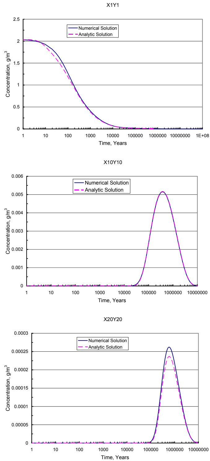
Figure 3.3-14. Time-Dependent Solutions for a = 20 m b = 150 m
