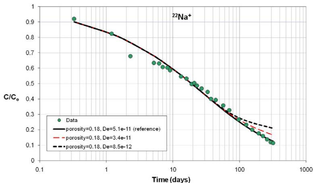
Figure A-7. Measured and Computed Na Concentration with Several Effective Diffusion Coefficients ( \text{m}^2/\text{s} )
