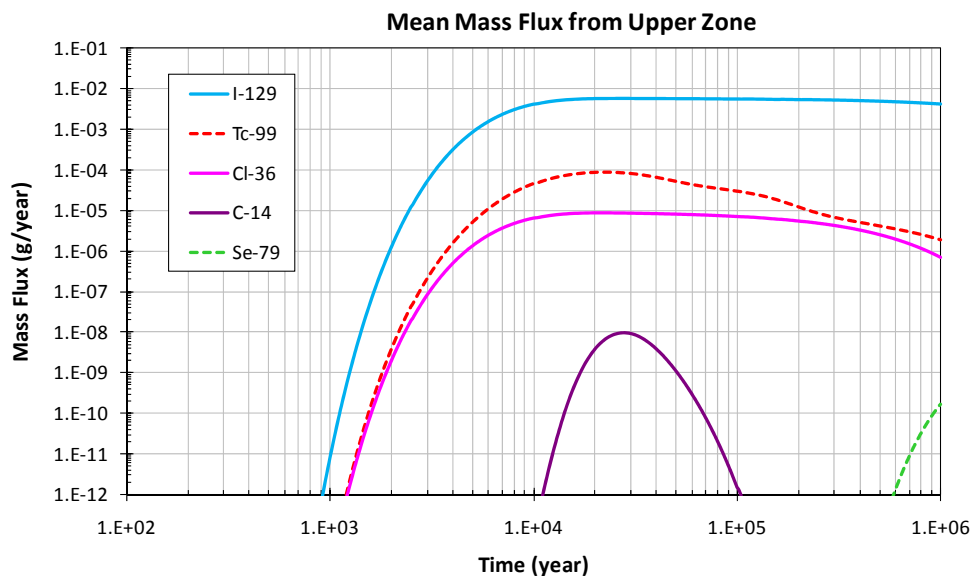
Figure 3.4-18. Commercial UNF Model Results for the High Permeability Case: Mean Mass Release Rate from Upper Zone
