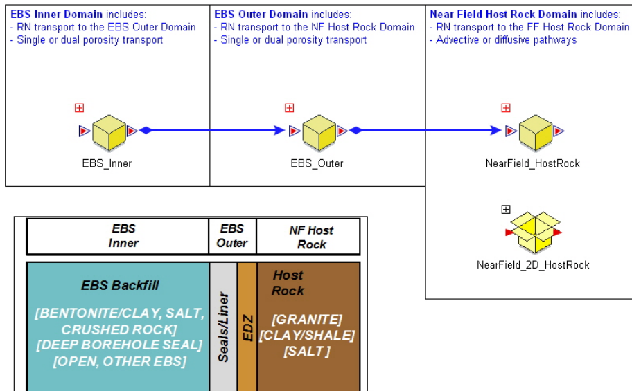
Figure 4-6. GoldSim GPAM Near Field Region
