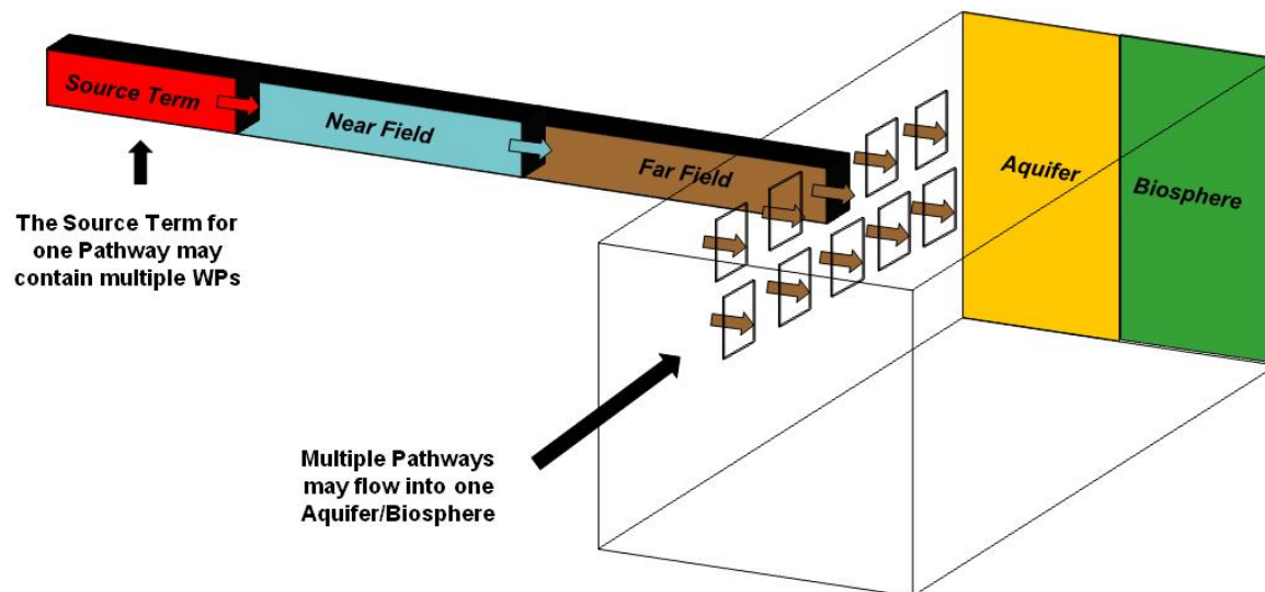
Figure 4-8. Schematic Representation of a GPAM Transport Pathway
