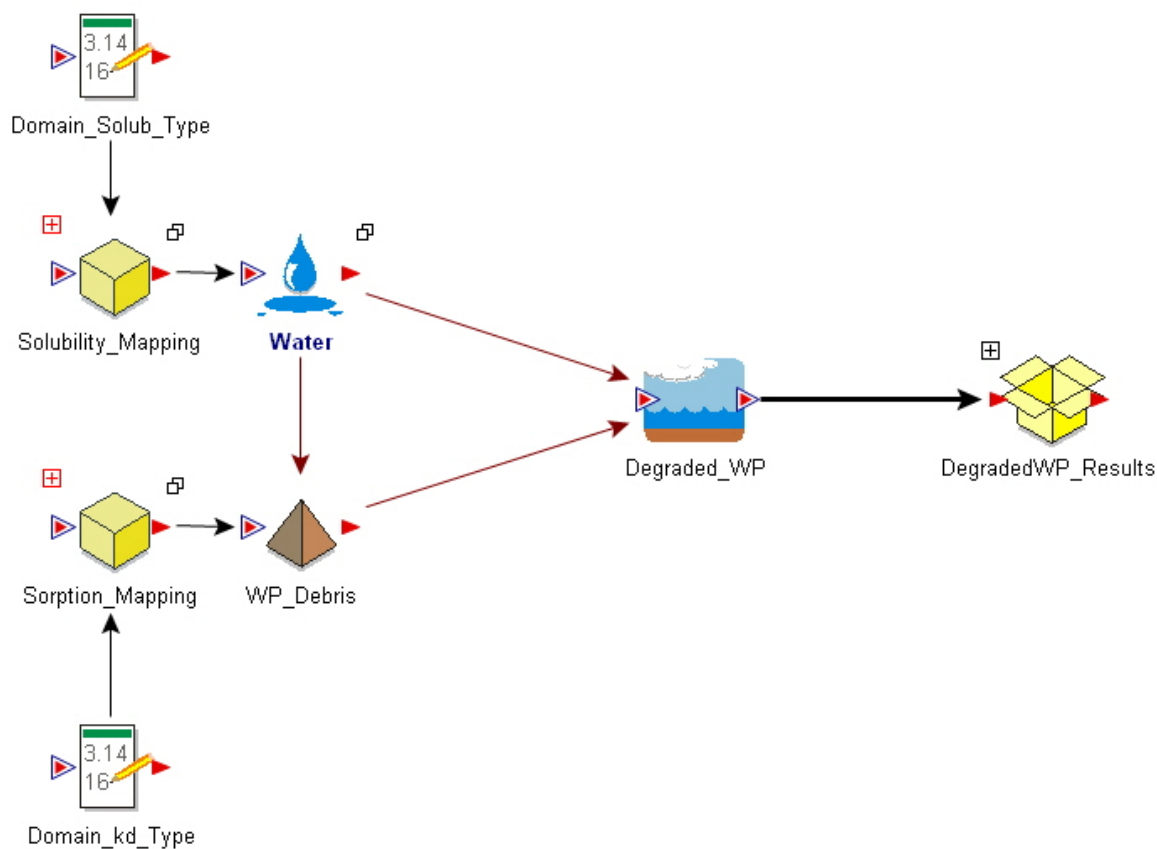
Figure 4-10. GoldSim GPAM Degraded Waste Package Domain Element
