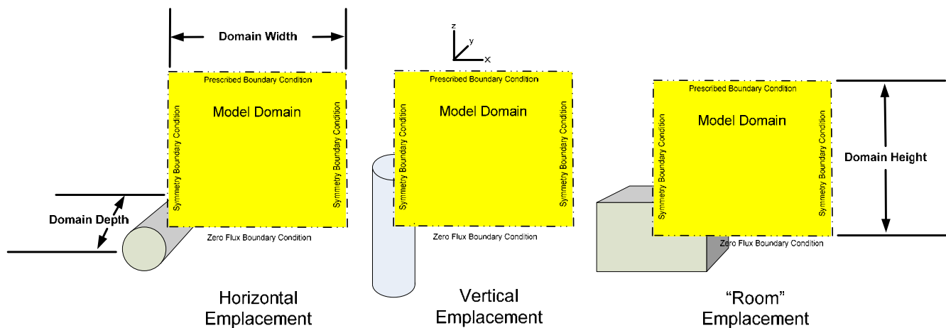
Figure 3.3-3. Conceptual Framework for Clay GDS Models
