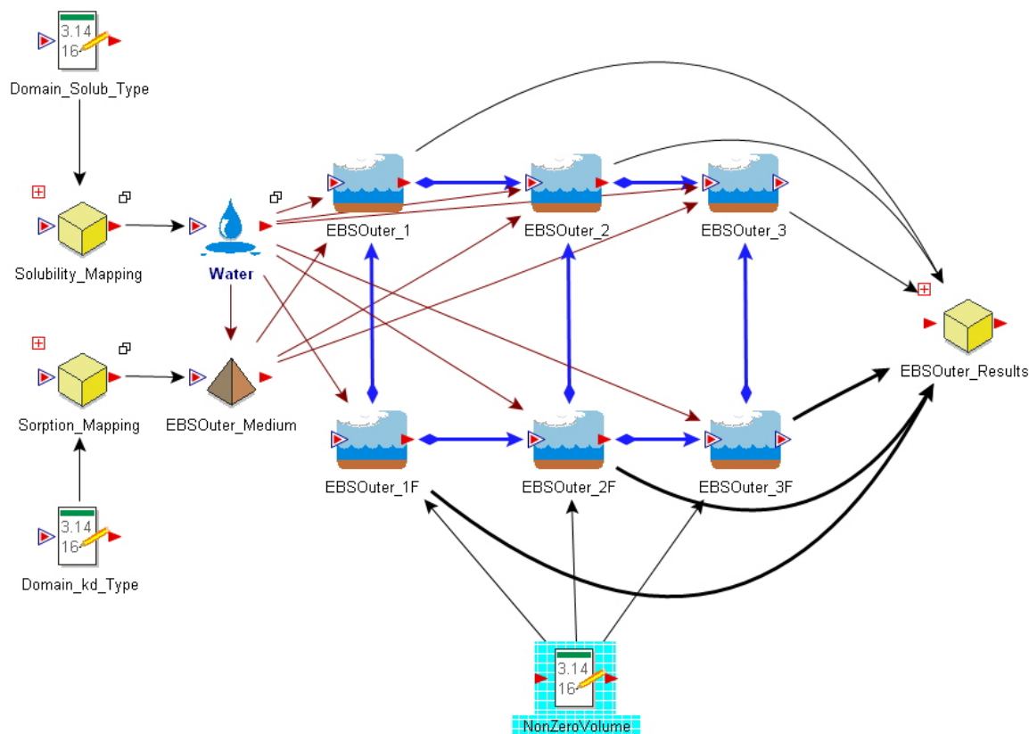
Figure 4-12. GoldSim GPAM EBS Outer Domain Elements
