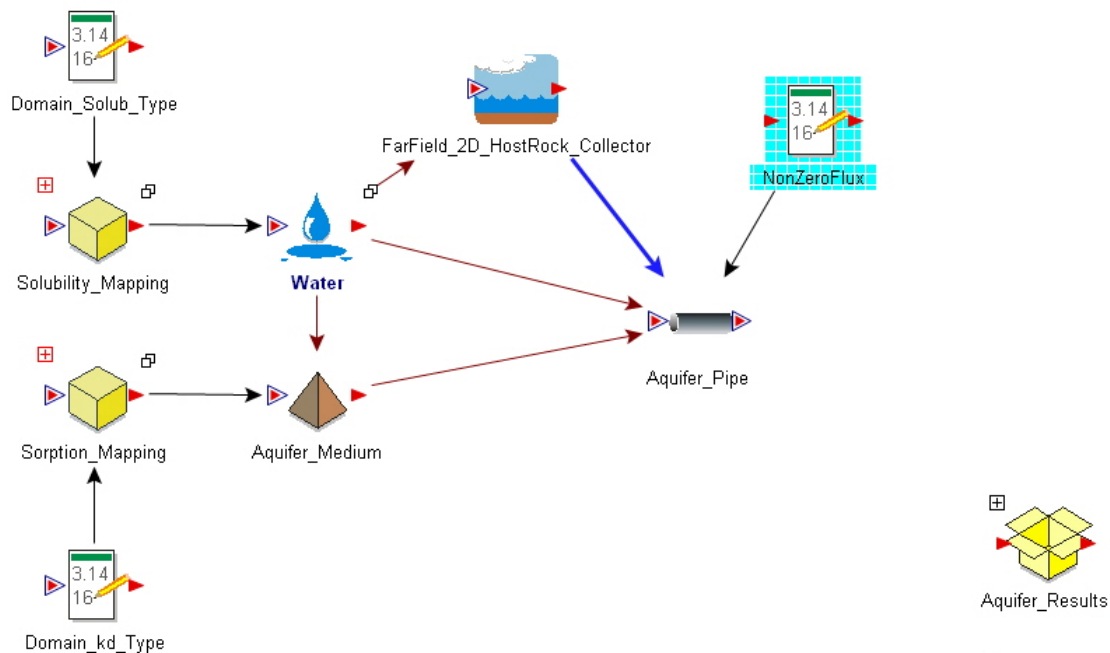
Figure 4-15. GoldSim GPAM Aquifer Domain Elements
