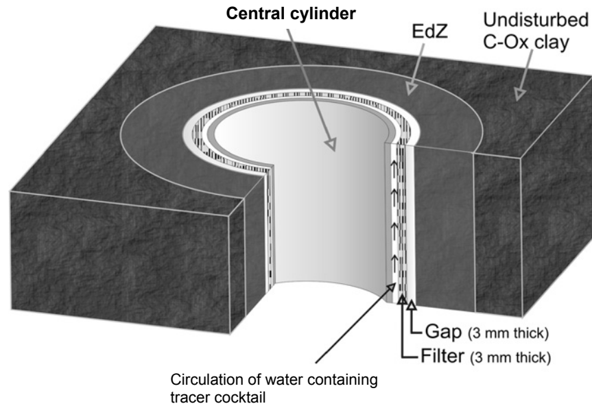
Figure A-5. Sketch of Borehole Geometry for DIR Experiments
