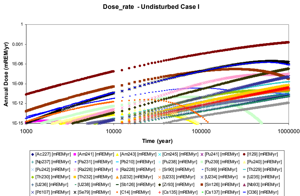
Figure 3.2-6. Undisturbed Scenario: Mean Annual Dose of 100 Realizations for 36 Individual Radionuclide Species
