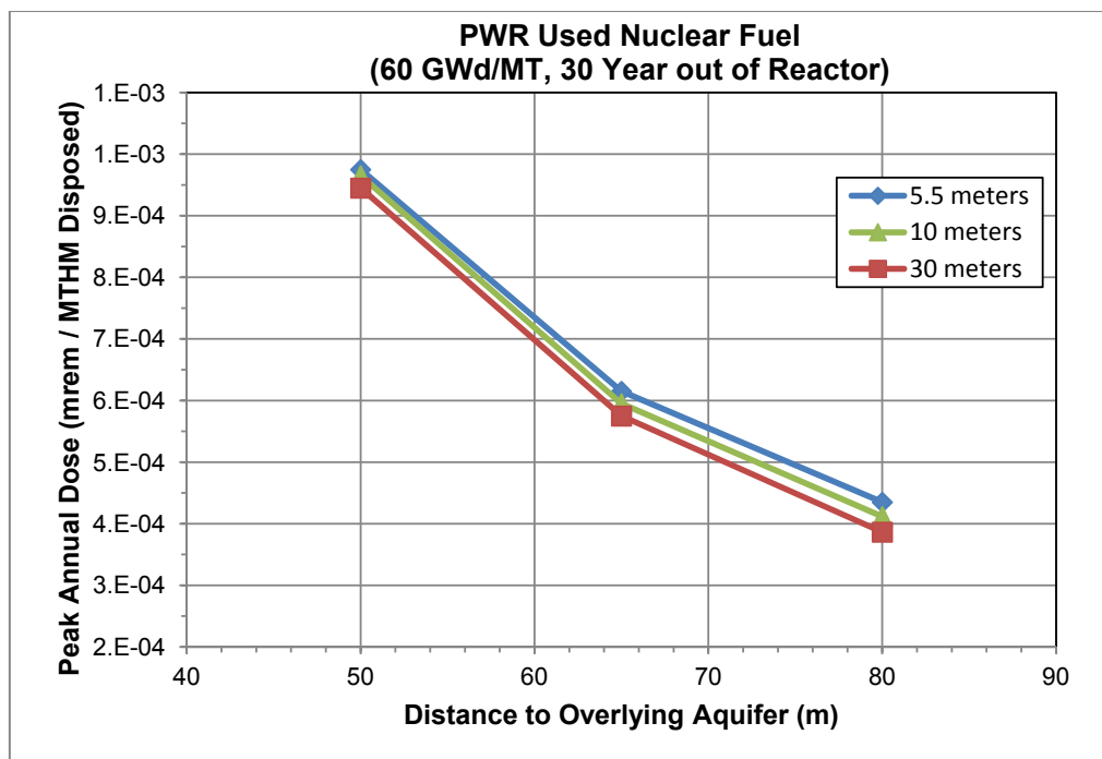
Figure 3.3-31. Clay GDS Model Sensitivity Analysis – Effect of Disposal System Configuration
