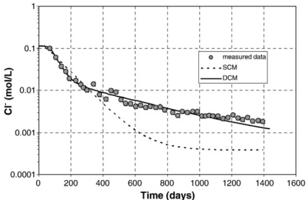
Figure A-2. Measured and Computed Breakthrough Curves of Chloride with Single-Continuum Model and Dual-Continuum Model
