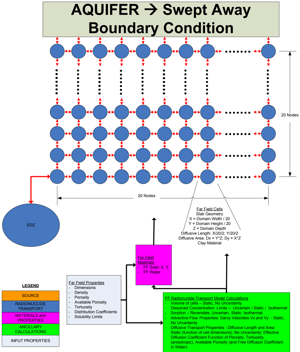
Figure 3.3-9. Schematic of Far-Field Representation
