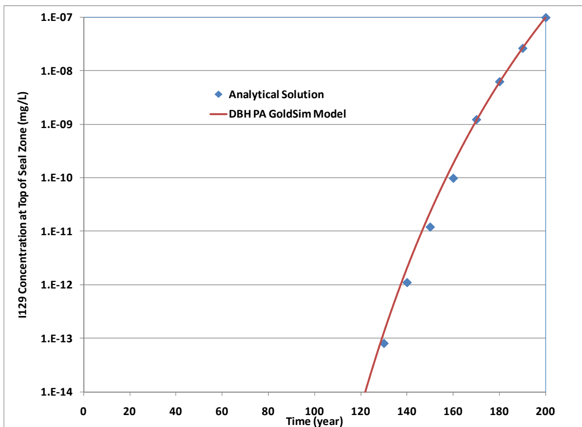
Figure 3.4-4. Comparison of I^{129} Concentration Predictions at Top of Seal Zone for the Analytical Solution and Deep Borehole GDS Model
