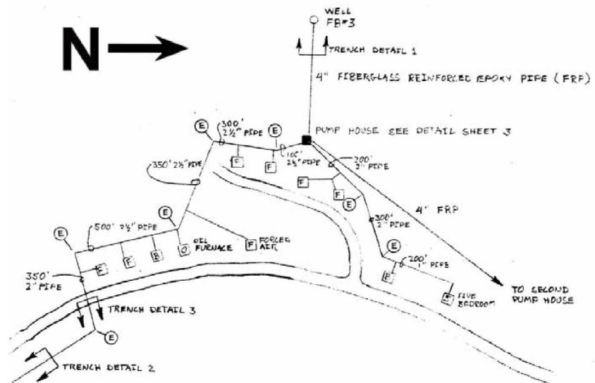
Figure 3 – Partial Chitwood Pipe Distribution Layout
