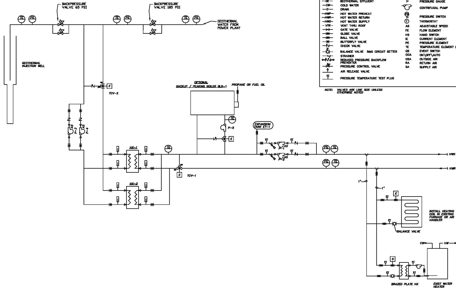
SYSTEM SCHEMATIC NTS
