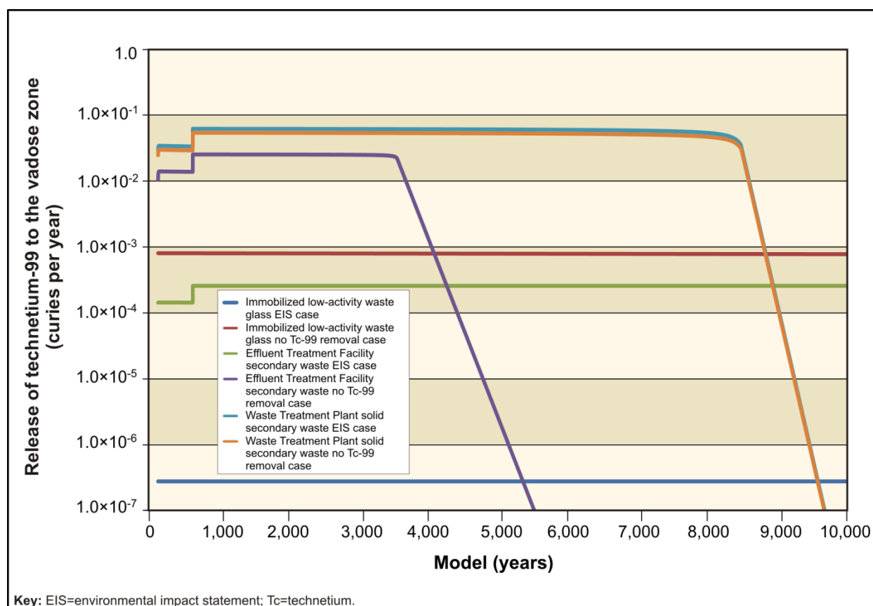
Figure M-140. Release of Technetium-99 to the Vadose Zone, TC & WM EIS and No-Technetium-99-Removal Sensitivity Cases
