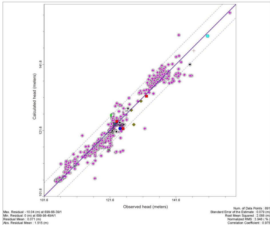
Figure L–67. 100th Percentile Flow Model Residuals, Calendar Year 2010
