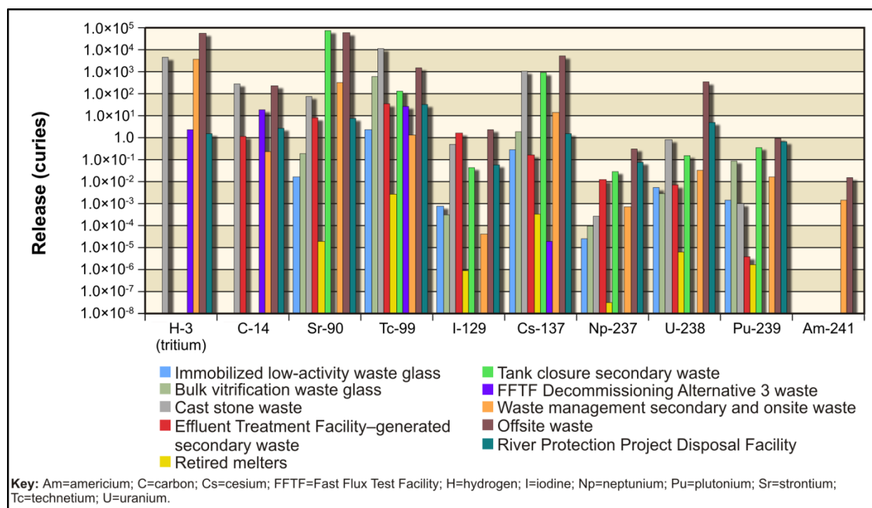
Figure M-72. Waste Management Alternative 2, Disposal Group 1, Subgroup 1-E, Radionuclide Releases to the Vadoso Zone
