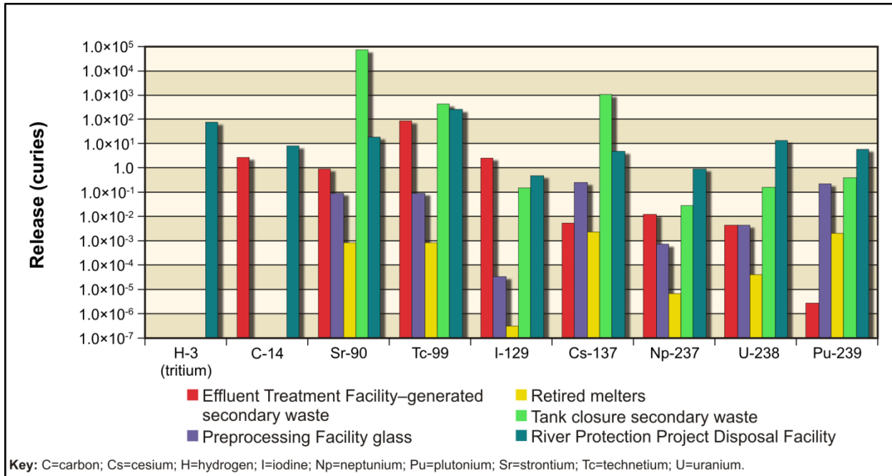
Figure M-108. Waste Management Alternative 3, Disposal Group 2, Subgroup 2-B, Option Case, Radionuclide Releases to the Vadose Zone from the 200-East Area Integrated Disposal Facility
