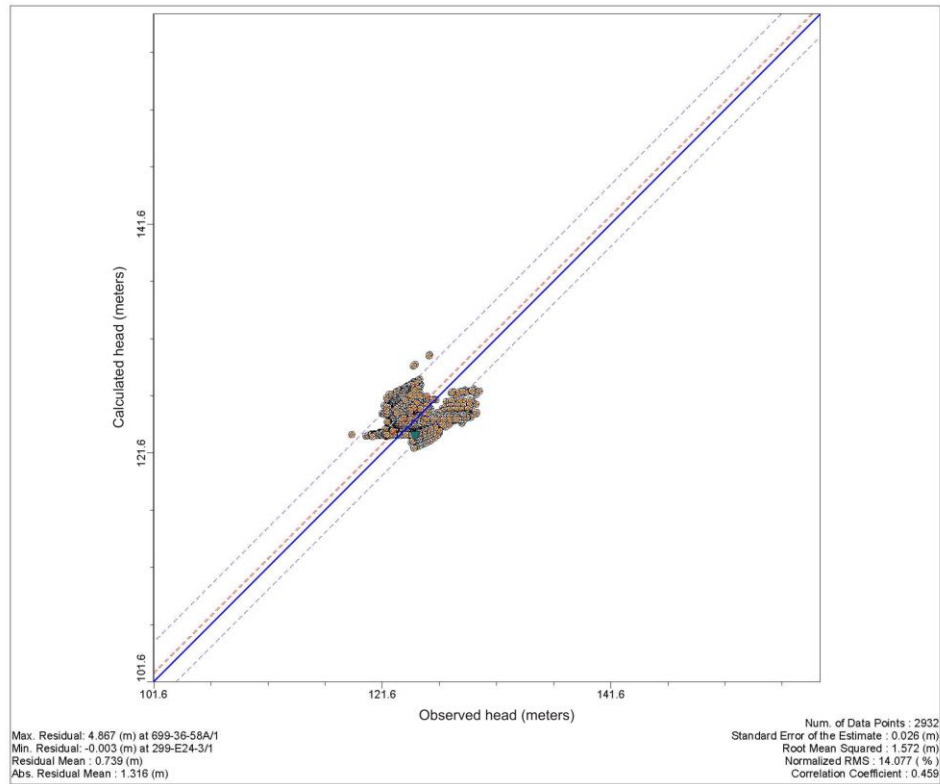
Figure L–33. 95th Percentile (Base Case) Flow Model Residuals – 200-East Area
