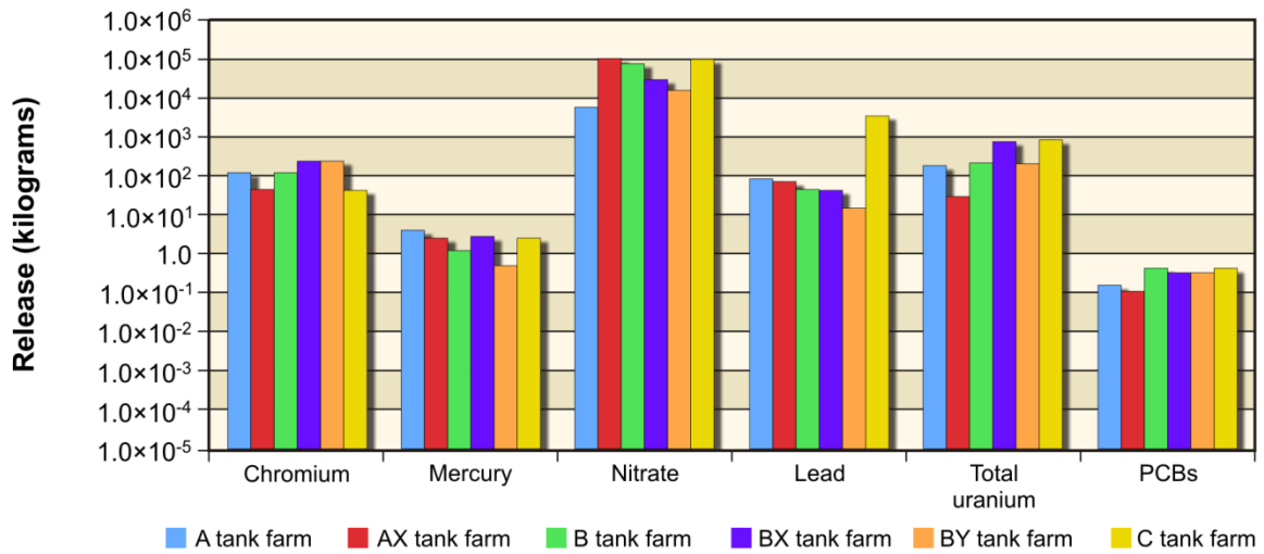
Figure M-33. Tank Closure Alternatives 2B, 3A, 3B, 3C, and 6C Chemical Releases to the Vadose Zone from Retrieval Losses in Tank Farms A, AX, B, BX, BY, and C
