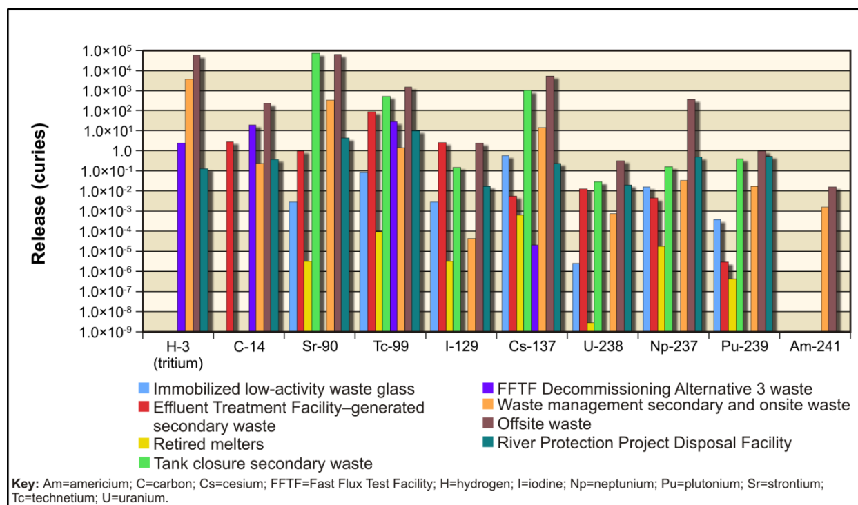
Figure M-64. Waste Management Alternative 2, Disposal Group 1, Subgroup 1-A, Radionuclide Releases to the Vadoso Zone
