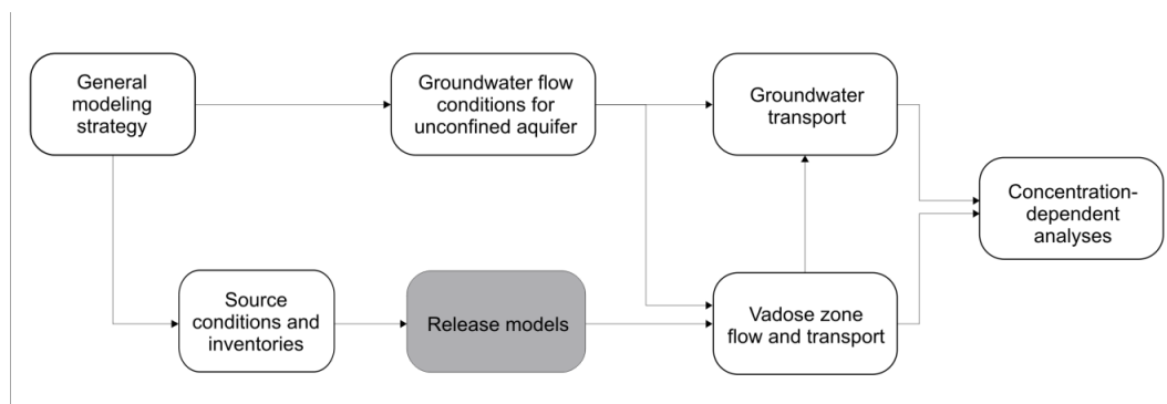
Figure M-1. Groundwater Modeling System Flowchart
