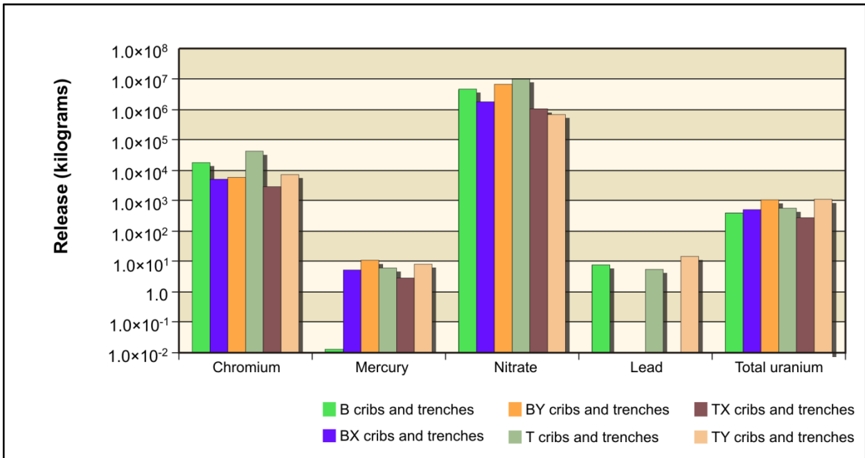
Figure M-12. Chemical Releases to the Vadose Zone from Alternative Cribs and Trenches (Ditches)
