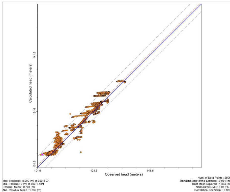
Figure L-70. 100th Percentile Flow Model Residuals in Southern Region of Model
