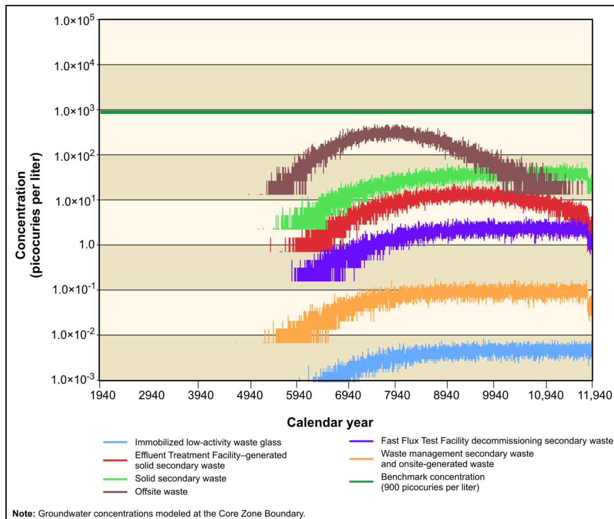
Figure M-134. Tank Closure Alternative 2B Groundwater Technetium-99 Concentration at the Core Zone Boundary
