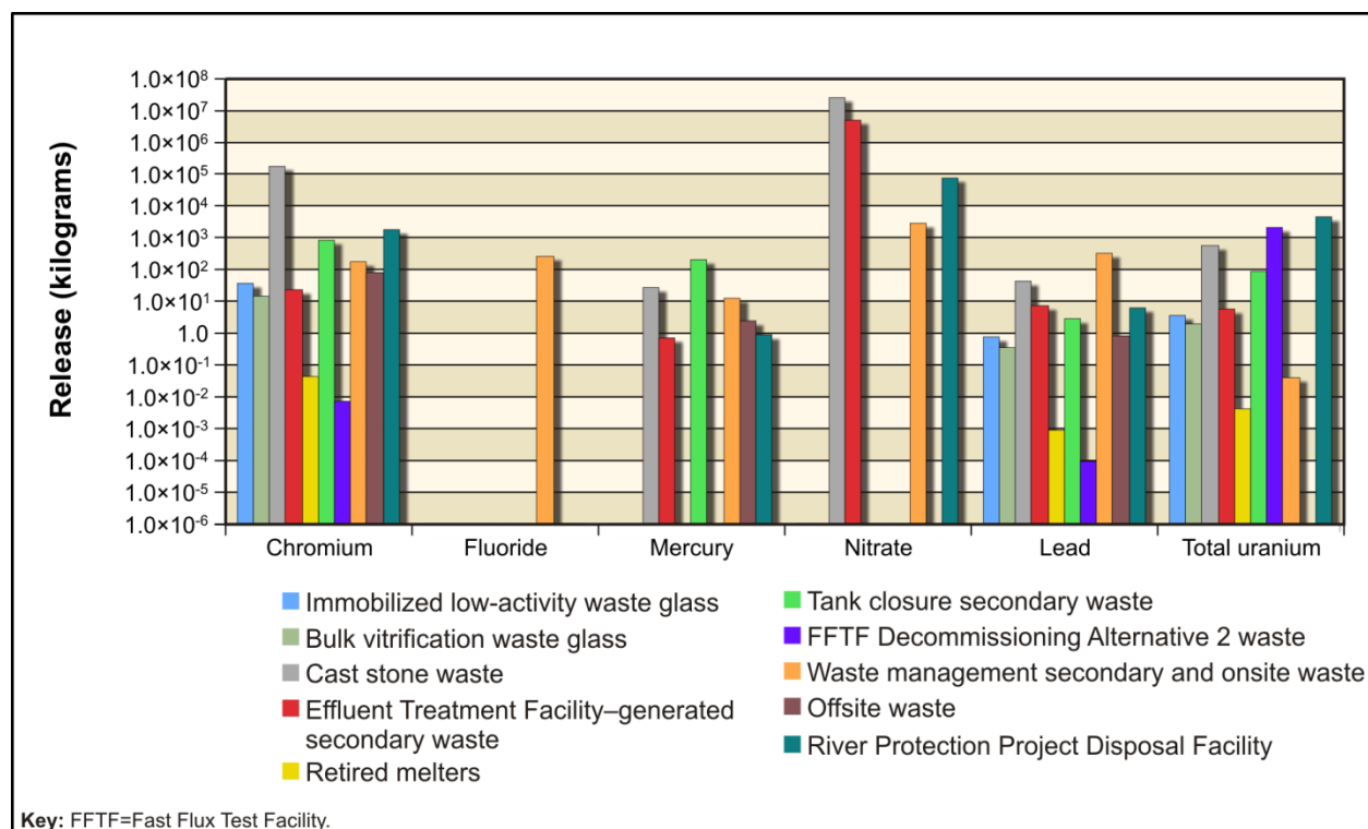
Figure M-73. Waste Management Alternative 2, Disposal Group 1, Subgroup 1-E, Chemical Releases to the Vadoso Zone
