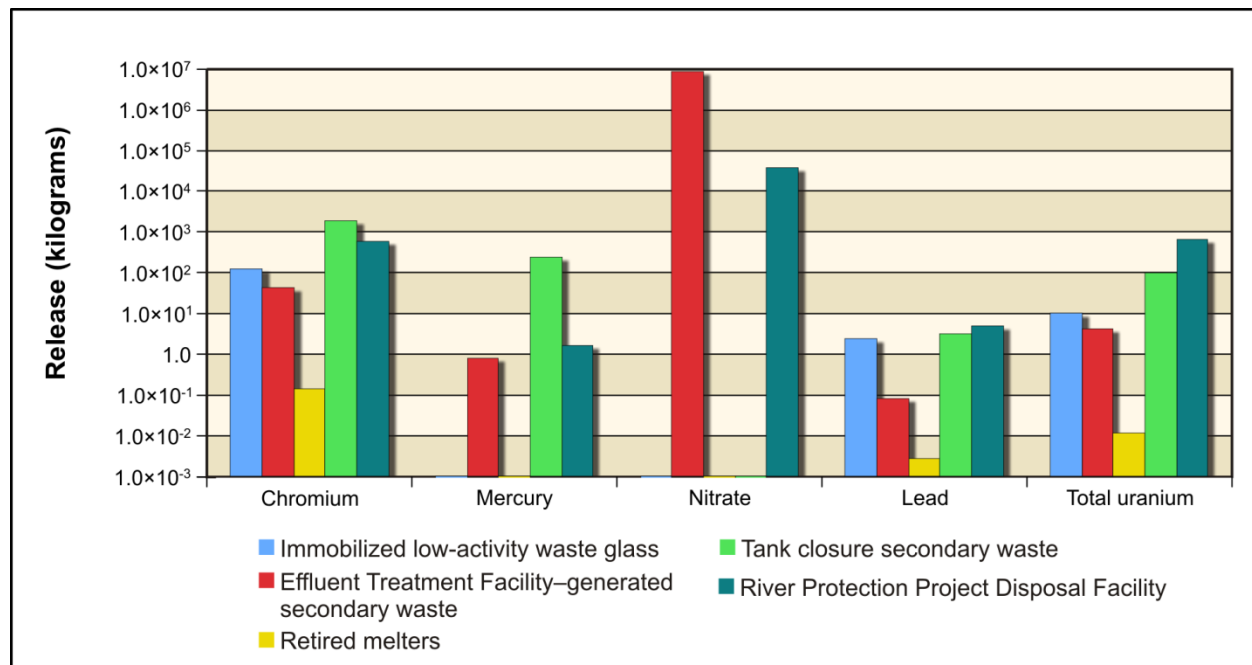
Figure M-91. Waste Management Alternative 3, Disposal Group 1, Subgroup 1-A, Chemical Releases to the Vadose Zone from the 200-East Area Integrated Disposal Facility
