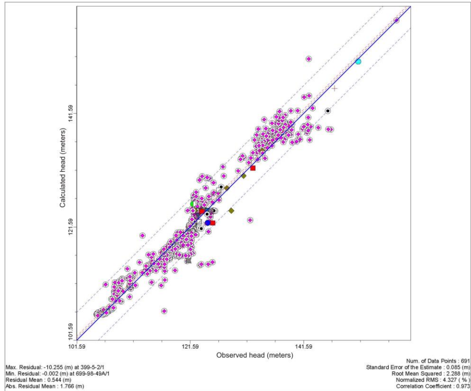
Figure L-95. 66th Percentile Flow Model Residuals, Calendar Year 2010
