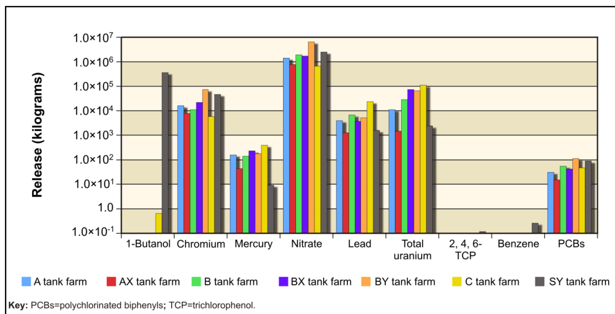
Figure M-17. Tank Closure Alternative 1 Chemical Releases to the Vadose Zone from Other Sources in Tank Farms A, AX, B, BX, BY, C, and SY
