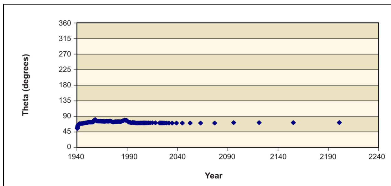
Figure L-52. 95th Percentile (Base Case) Flow Model Velocity Direction at 216-B-26 (BC Crib in 200-East Area)
