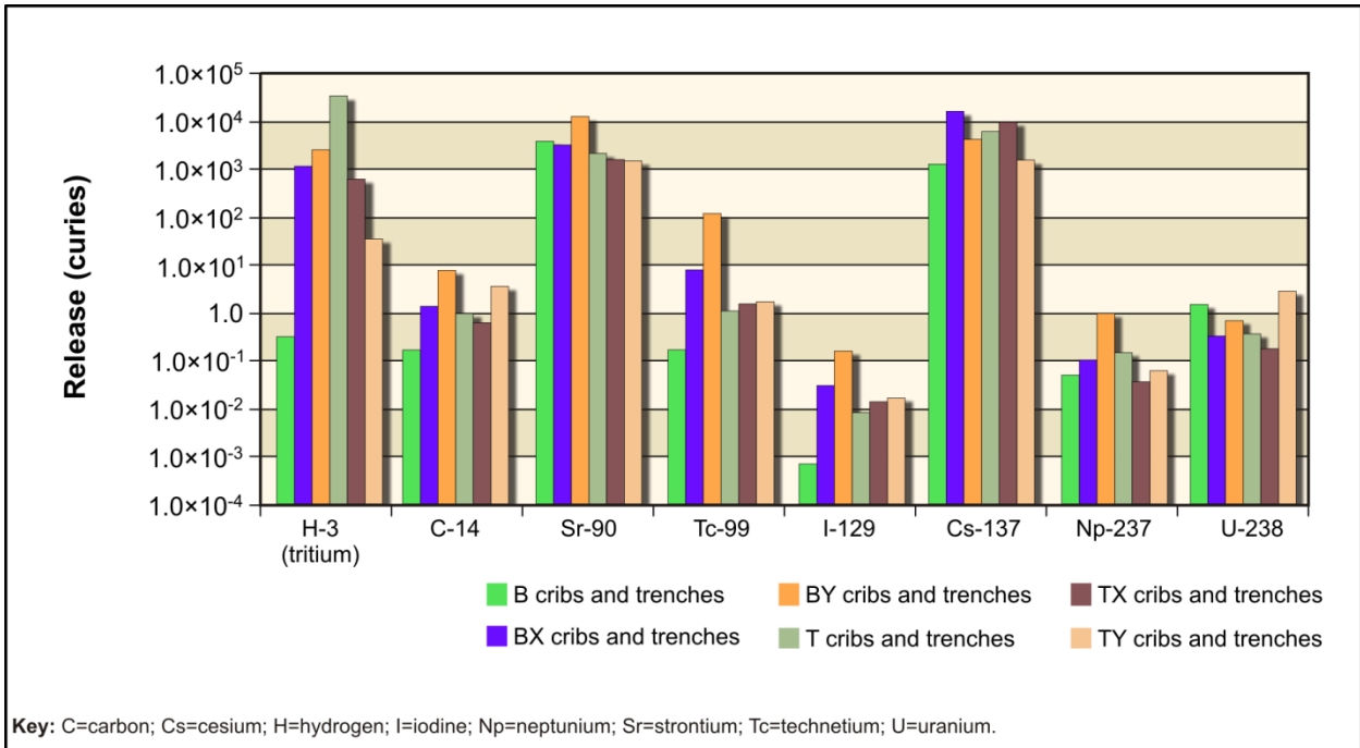
Figure M-11. Radionuclide Releases to the Vadose Zone from Alternative Cribs and Trenches (Ditches)
