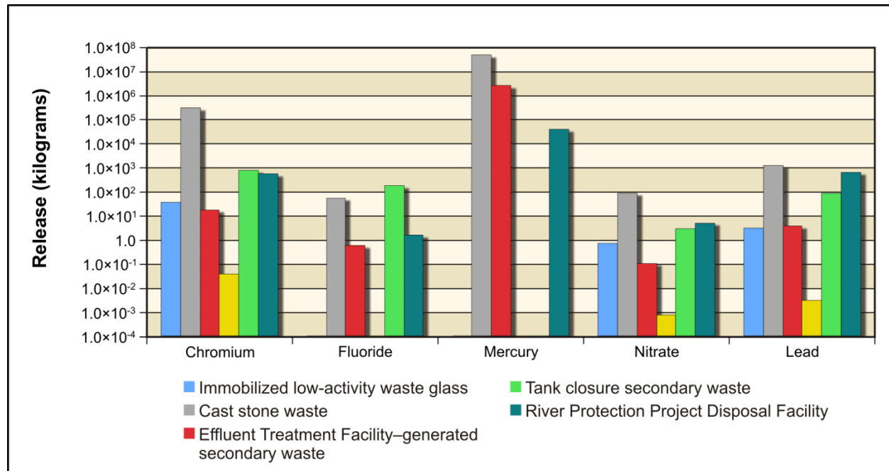
Figure M-95. Waste Management Alternative 3, Disposal Group 1, Subgroup 1-C, Chemical Releases to the Vadose Zone from the 200-East Area Integrated Disposal Facility
