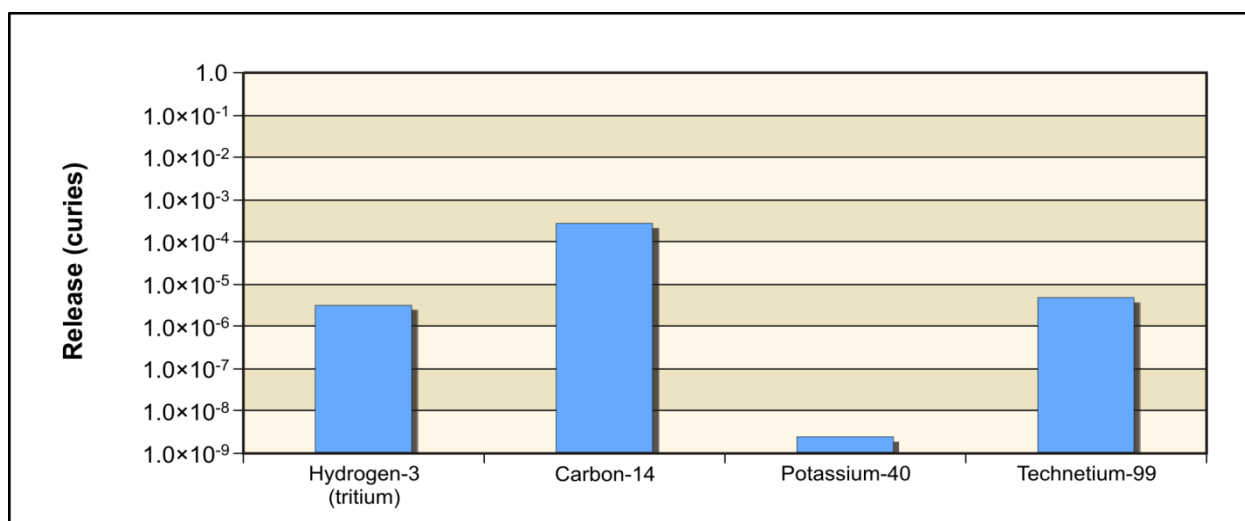
Figure M-61. FFTF Decommissioning Alternative 3 Radionuclide Releases to the Vadose Zone
