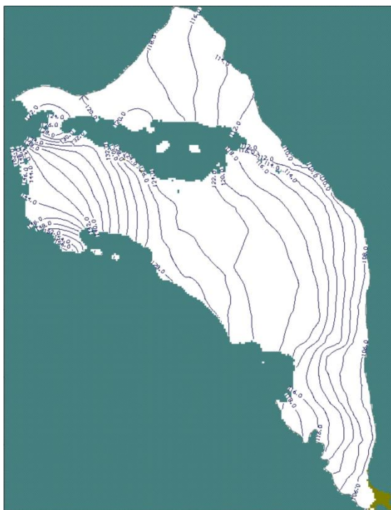
Figure L-104. 66th Percentile Flow Model Potentiometric Head Distribution, Calendar Year 1944
