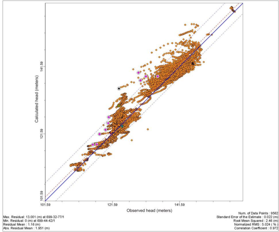
Figure L-97. 66th Percentile Flow Model Residuals in Central Region of Model
