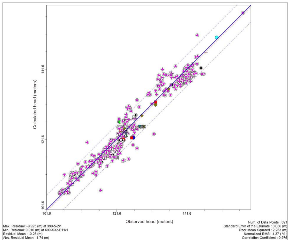
Figure L–66. 100th Percentile Flow Model Residuals, Calendar Year 1995
