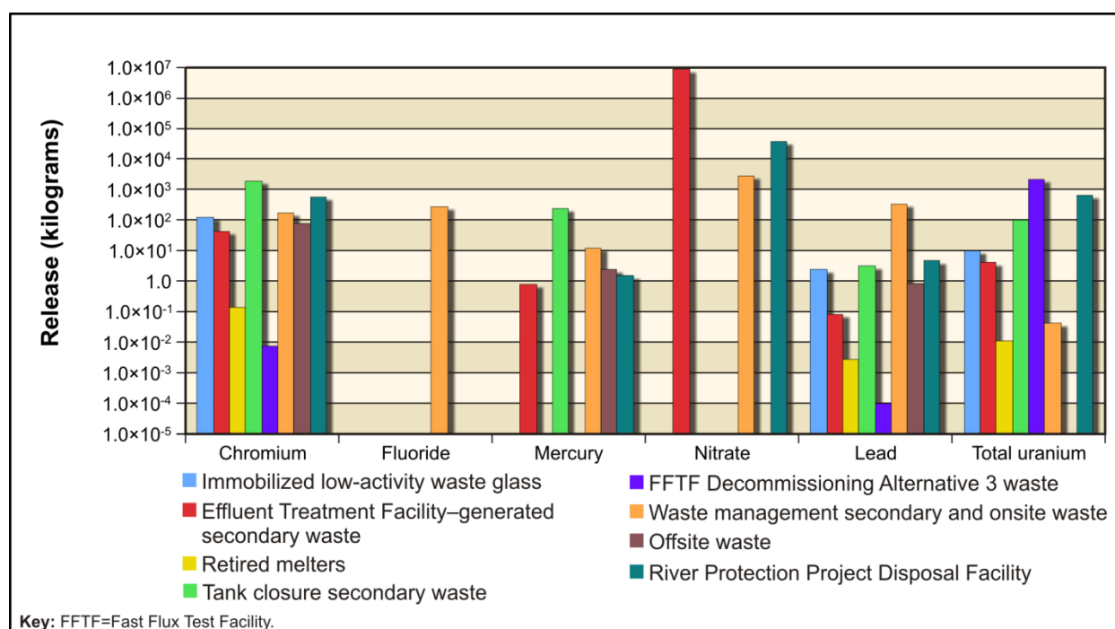
Figure M-65. Waste Management Alternative 2, Disposal Group 1, Subgroup 1-A, Chemical Releases to the Vadoso Zone
