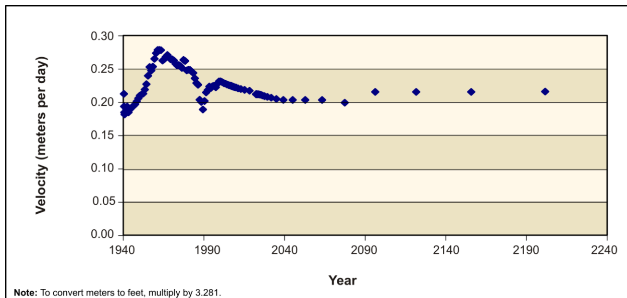
Figure L-51. 95th Percentile (Base Case) Flow Model Velocity Magnitude at 216-B-26 (BC Crib in 200-East Area)
