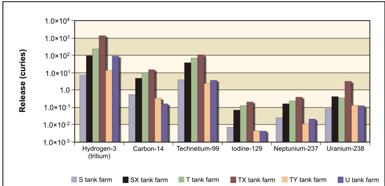
Figure M-9. Radionuclide Releases to the Vadose Zone from the 200-West Area Tank Farm Past Leaks
