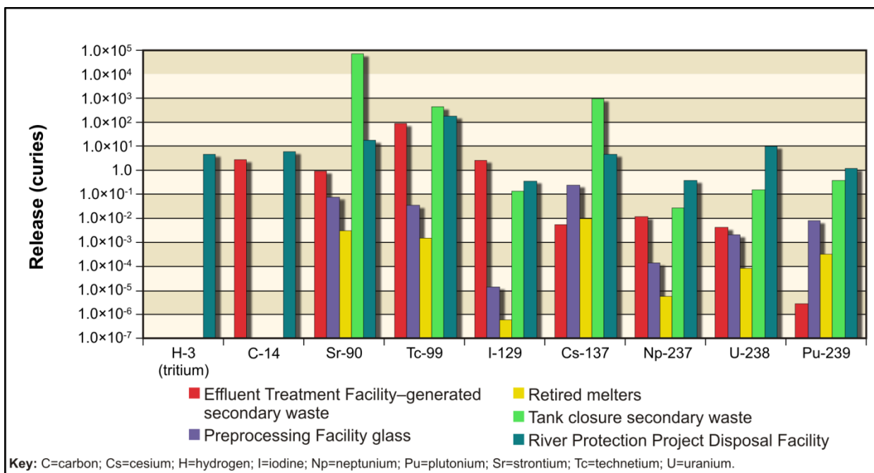
Figure M-106. Waste Management Alternative 3, Disposal Group 2, Subgroup 2-B, Base Case, Radionuclide Releases to the Vadose Zone from the 200-East Area Integrated Disposal Facility
