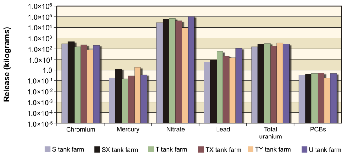
Figure M-34. Tank Closure Alternatives 2B, 3A, 3B, 3C, and 6C Chemical Releases to the Vadose Zone from Retrieval Losses in Tank Farms S, SX, T, TX, TY, and U
