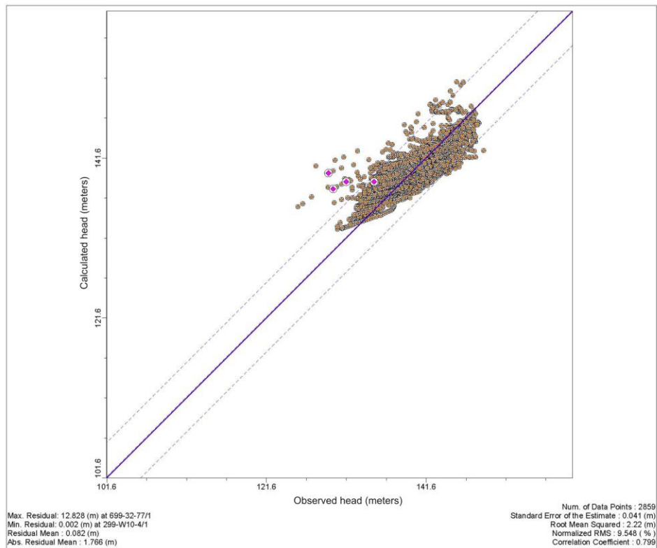
Figure L–34. 95th Percentile (Base Case) Flow Model Residuals – 200-West Area
