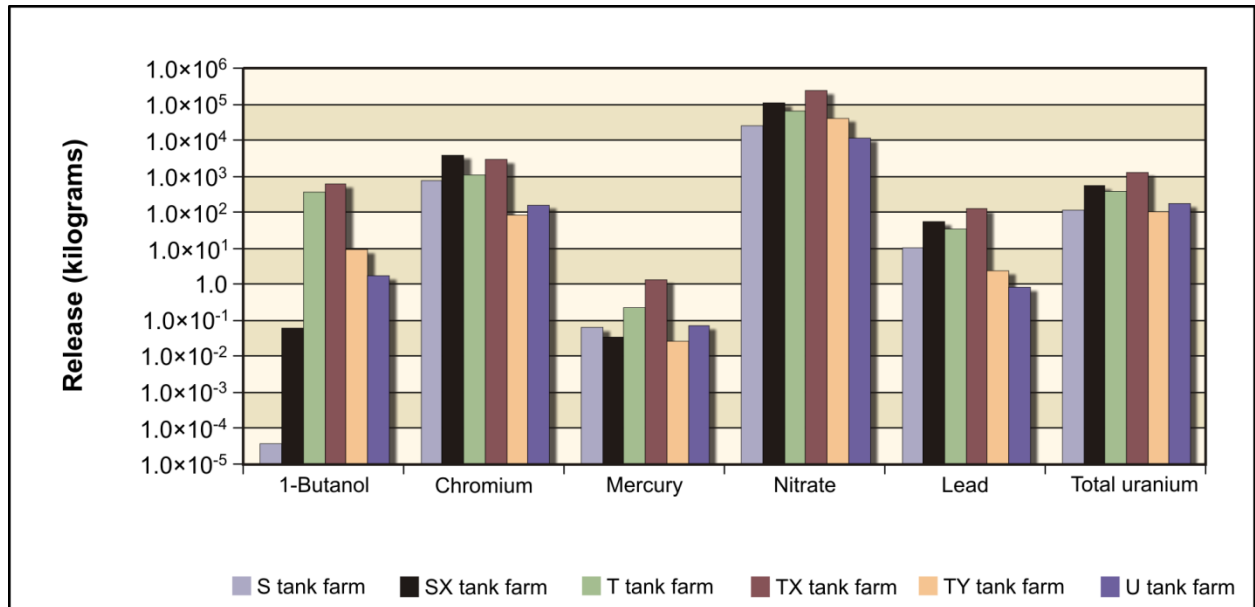
Figure M-10. Chemical Releases to the Vadose Zone from the 200-West Area Tank Farm Past Leaks
