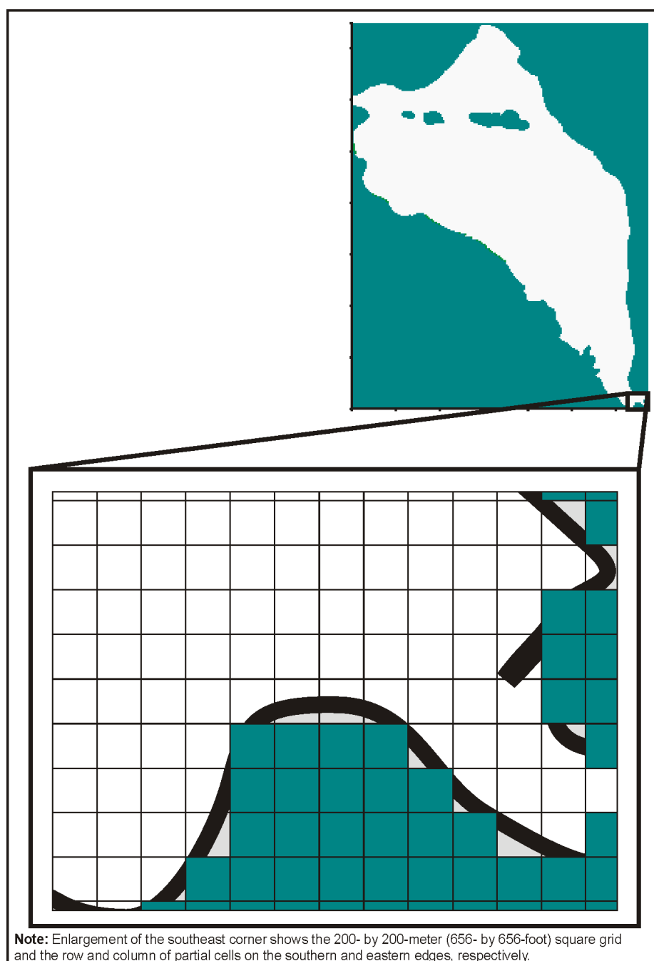
Figure L–17. Plan View of MODFLOW Horizontal Gridding
