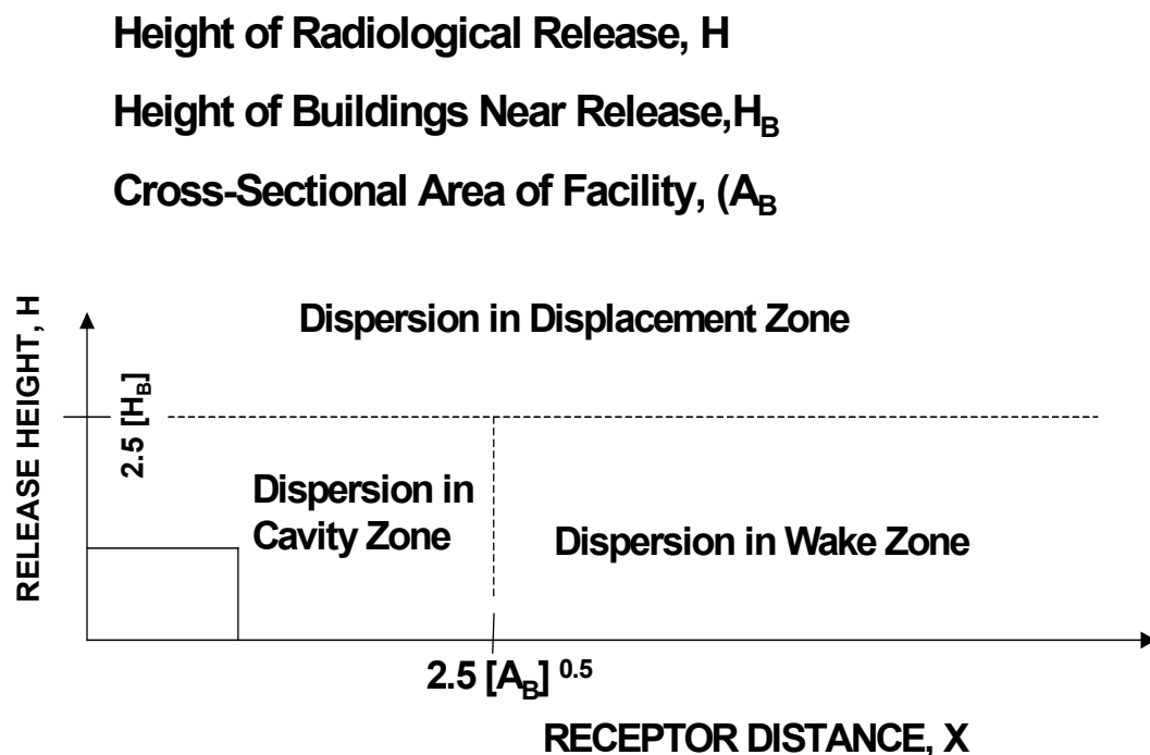
Figure A-3. Cavity and Wake Zones downwind of a Building Structure (Constant Wind Direction from Left to Right).
