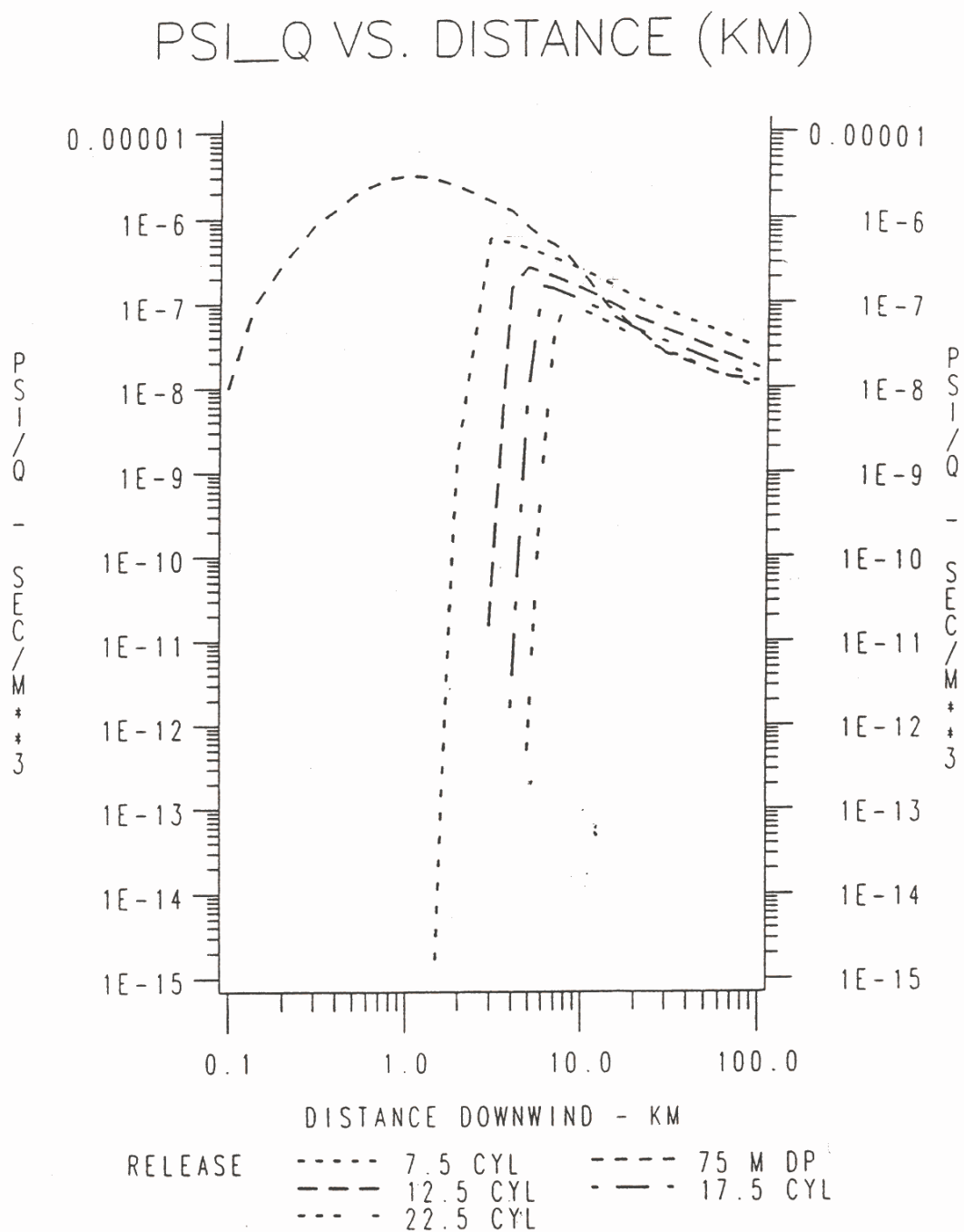
Figure A-2. The maximum time-integrated ground-level centerline air concentration ( \text{s/m}^3 ) versus downwind distance (km) for different mean translational speeds from 7.5m/s to 22.5 m/s. The downdraft speed is 10 m/s and the height of the cylindrical mesocyclone is 3500 m (from Weber and Hunter, 1996).
