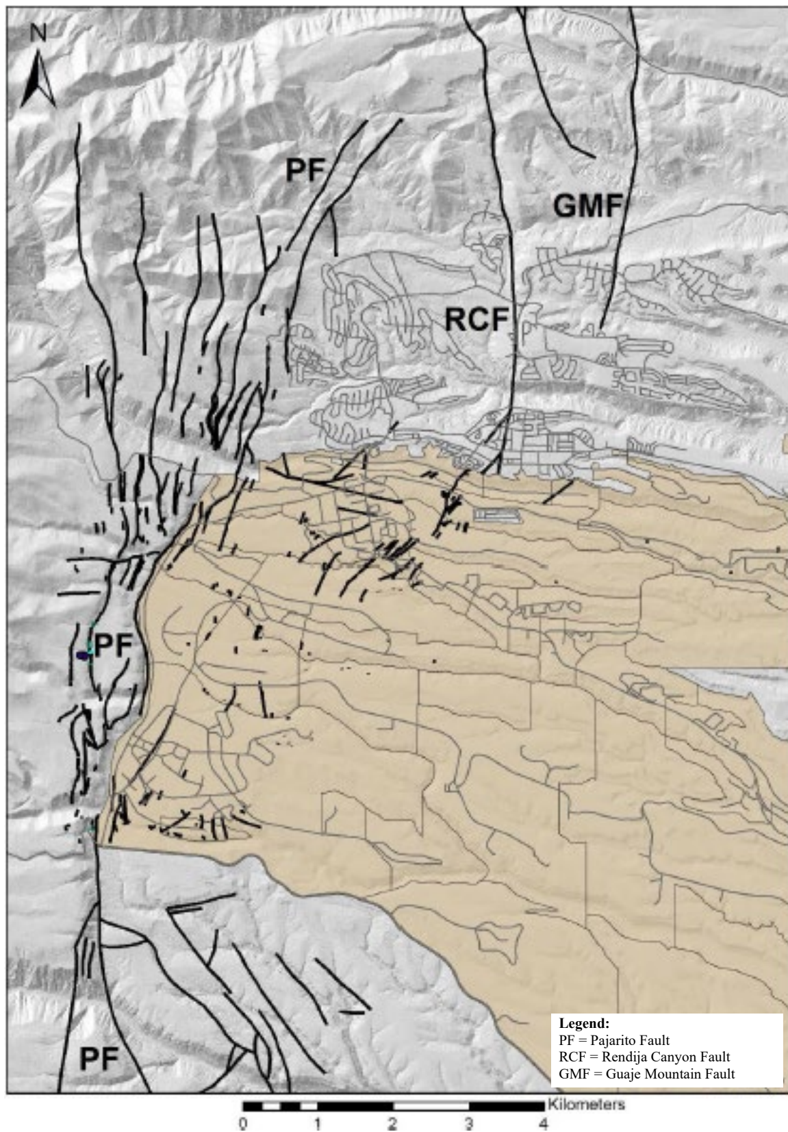
Figure A.4.3-2 Seismic Faults in the LANL Area
