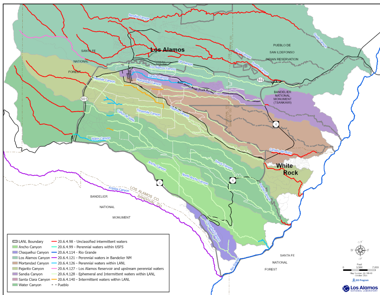
Figure A.4.4-1 Stream Reaches and Watersheds within and around LANL
