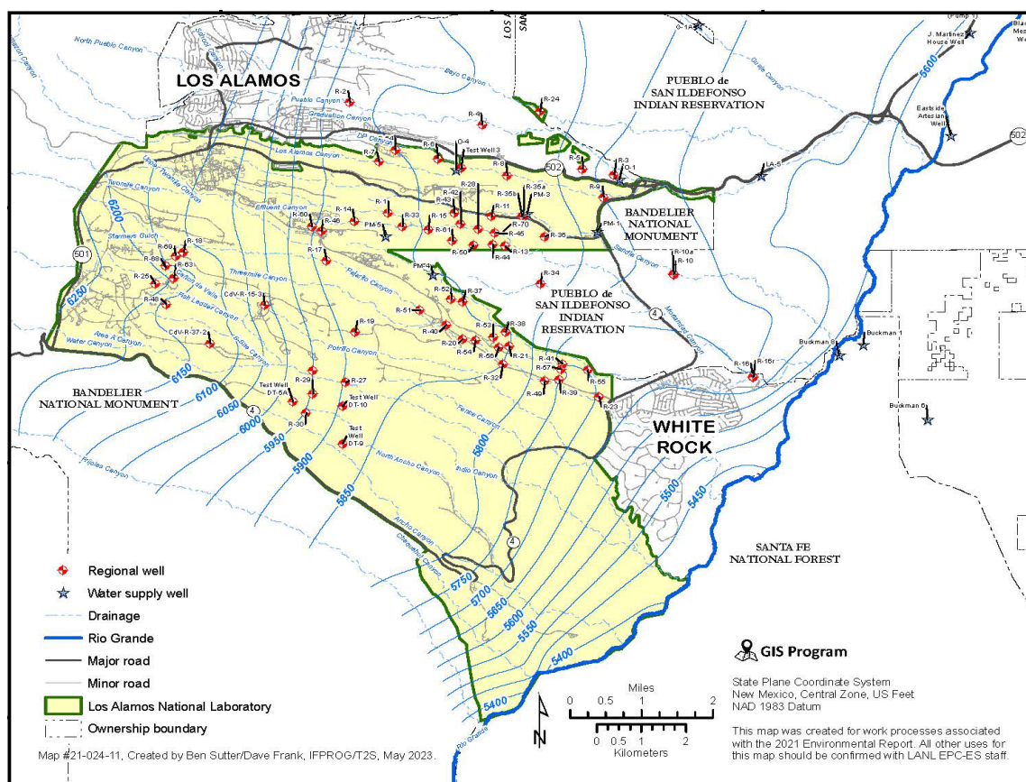
Figure A.4.4-8 Contour Map of Average Water Table Elevations for the Regional Aquifer
