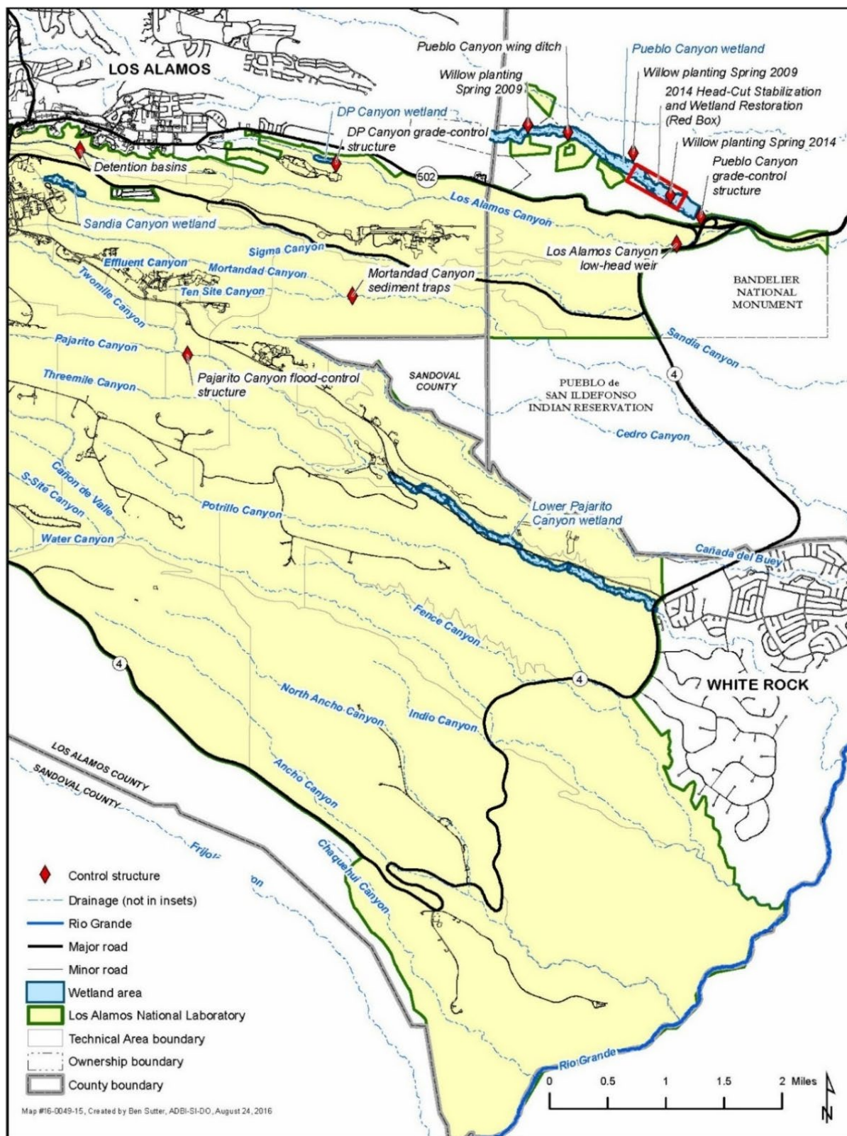
Figure A.4.4-4 Watershed Control Measures at the Laboratory in the Pueblo, Los Alamos, Sandia, and Mortandad Canyons
