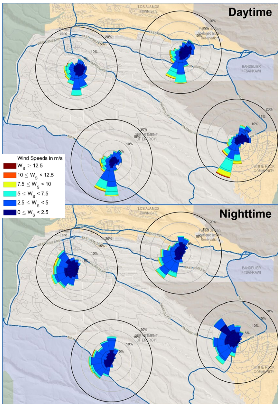
Figure A.4.5-2 Annual 15-Minute Average Wind Roses for 2021 at Four LANL Mesa-Top Meteorological Towers
