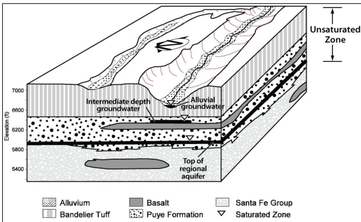
Figure A.4.4-7 Geologic and Hydrologic Relationships on the Pajarito Plateau
