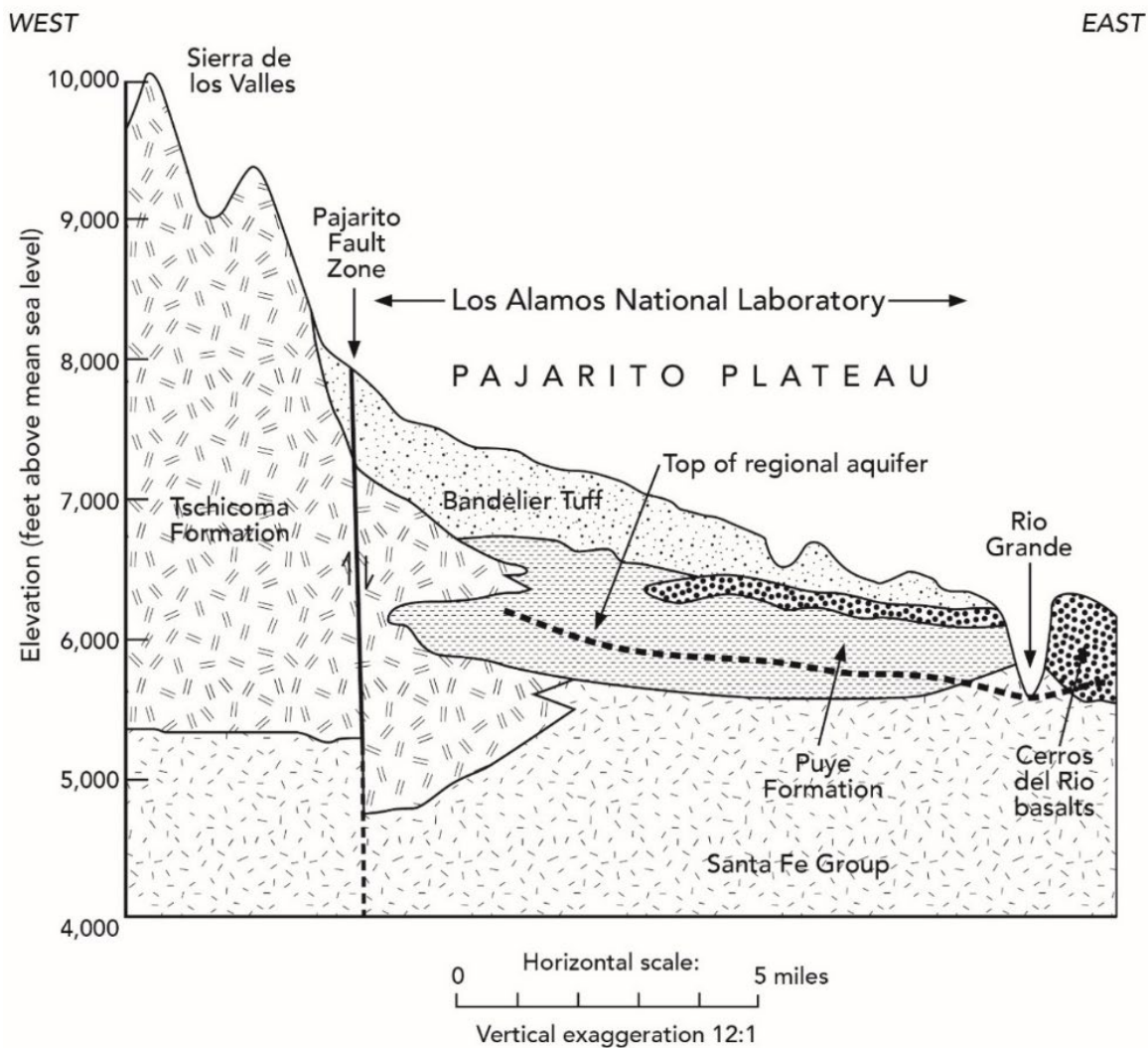
Figure A.4.3-1 Generalized Cross Section of the Los Alamos National Laboratory Area
