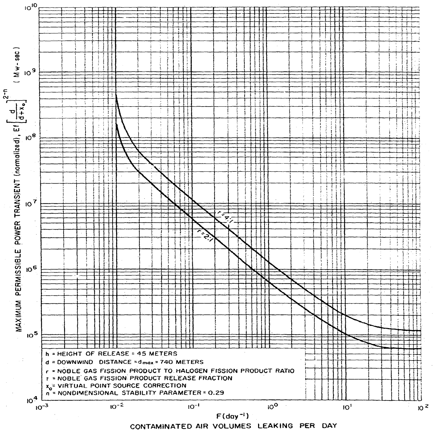
Figure III-9. Maximum Permissible Total Integrated Transient as a Function of Leakage Rate for 45 Meter Stack Release (Based on Dose Requirements for Site Boundary)
