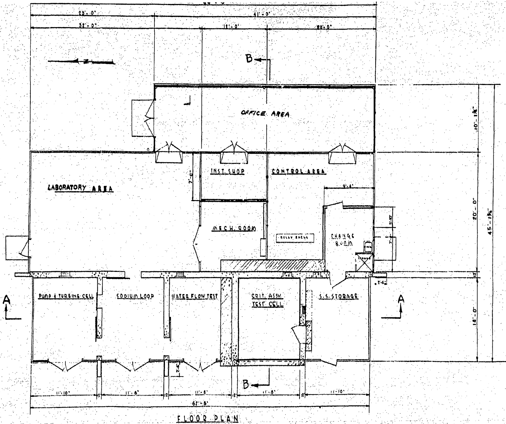
Figure V-1. Plan View of SNAP Critical Facility
