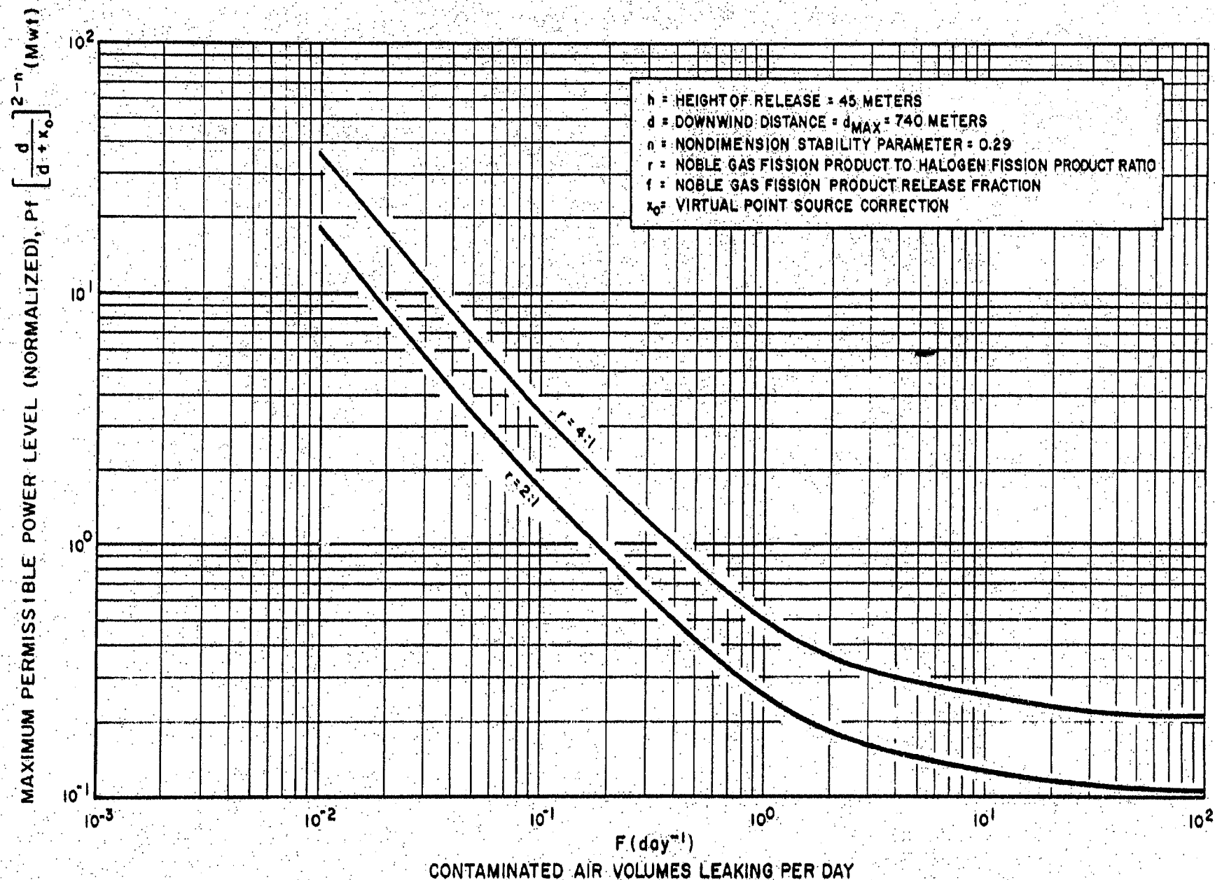
Figure III-4. Maximum Permissible Steady-State Power Level as a Function of Leakage Rate for 45 Meter Stack Release (Based on Dose Requirements for Site Boundary)
