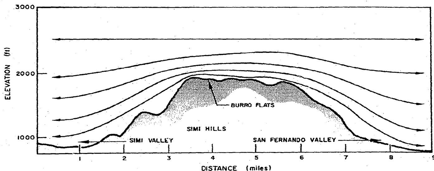
Figure II-13. Idealized Air Flow Over the Simi Hills
