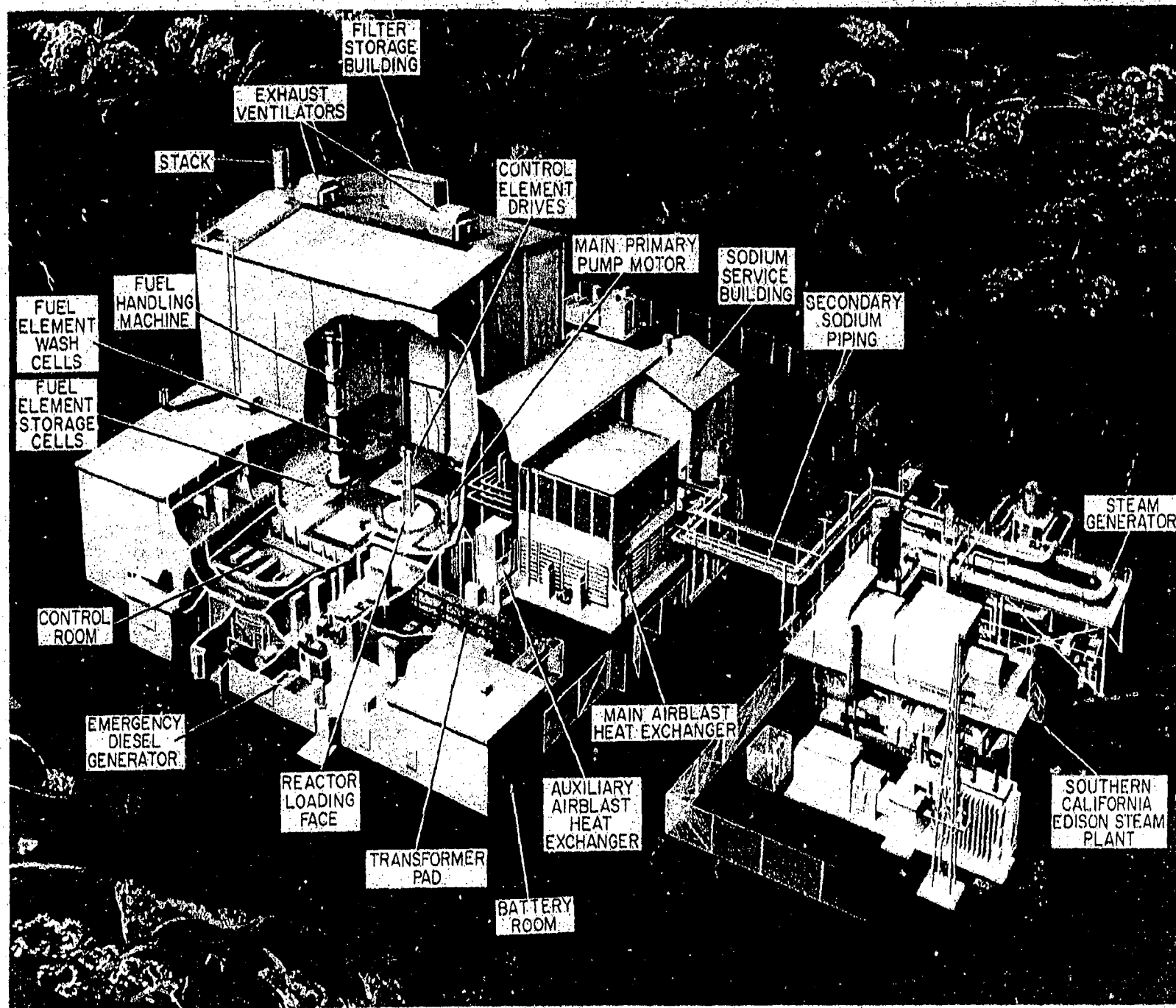
Figure V-14. Design of Sodium Reactor Experiment Facility
