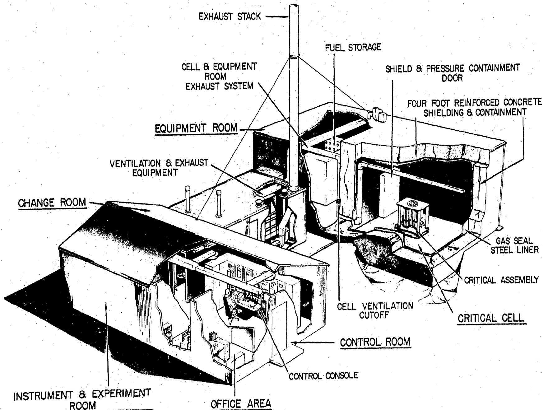
Figure V-3. Isometric View of SNAP Generalized Critical Facility
