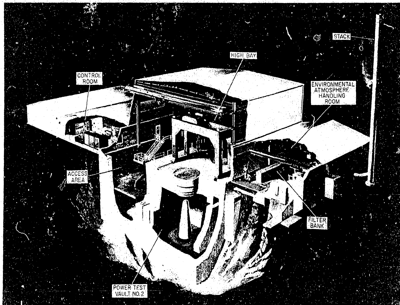
Figure V-7. Design of SNAP Environmental Test Facility
