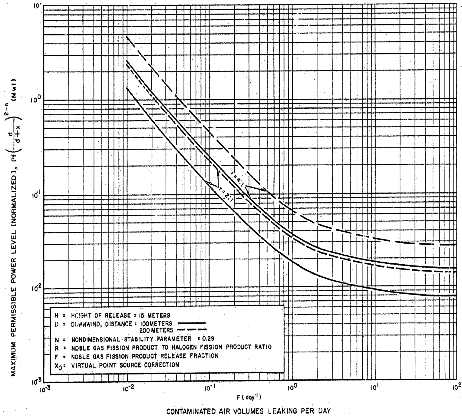
Figure III-2. Maximum Permissible Steady-State Power Level as a Function of Leakage Rate for 15 Meter Stack Release (Based on Dose Requirements for Site Boundary)
