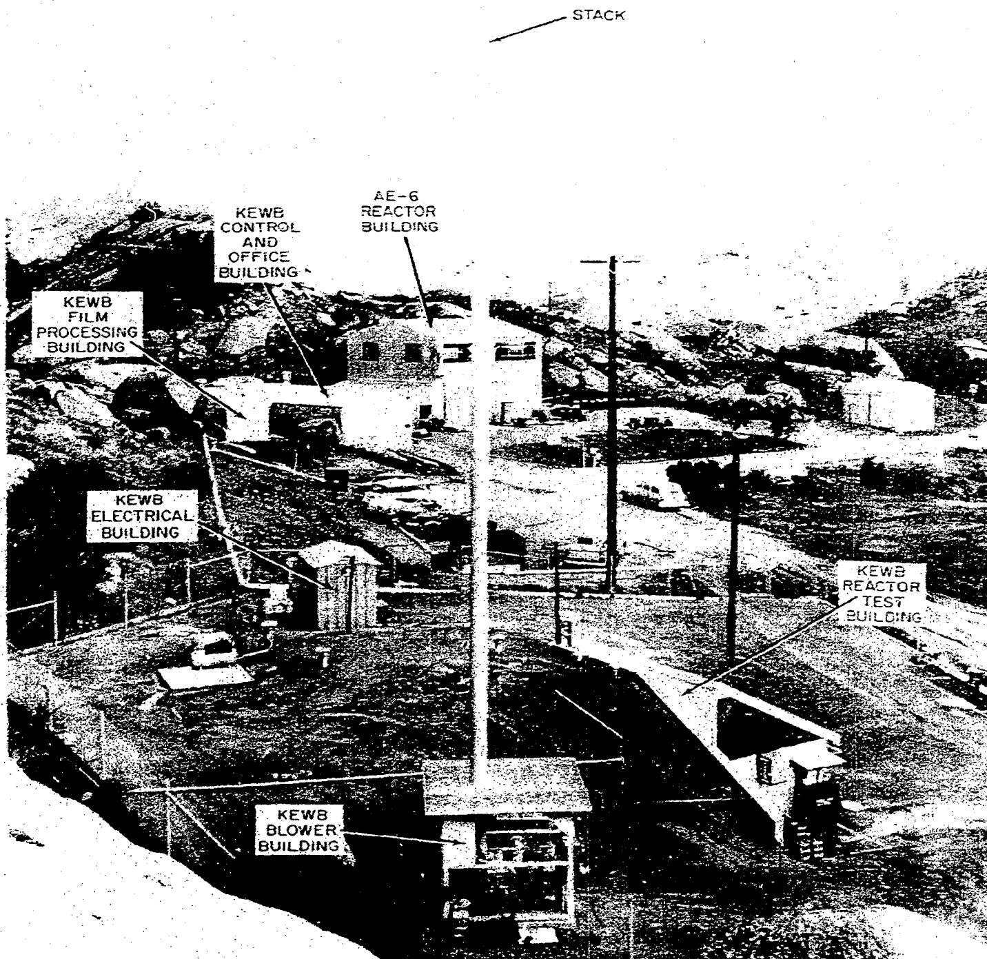
Figure V-10. Photograph of Kinetic Experiment Water Boiler Area and Facilities
