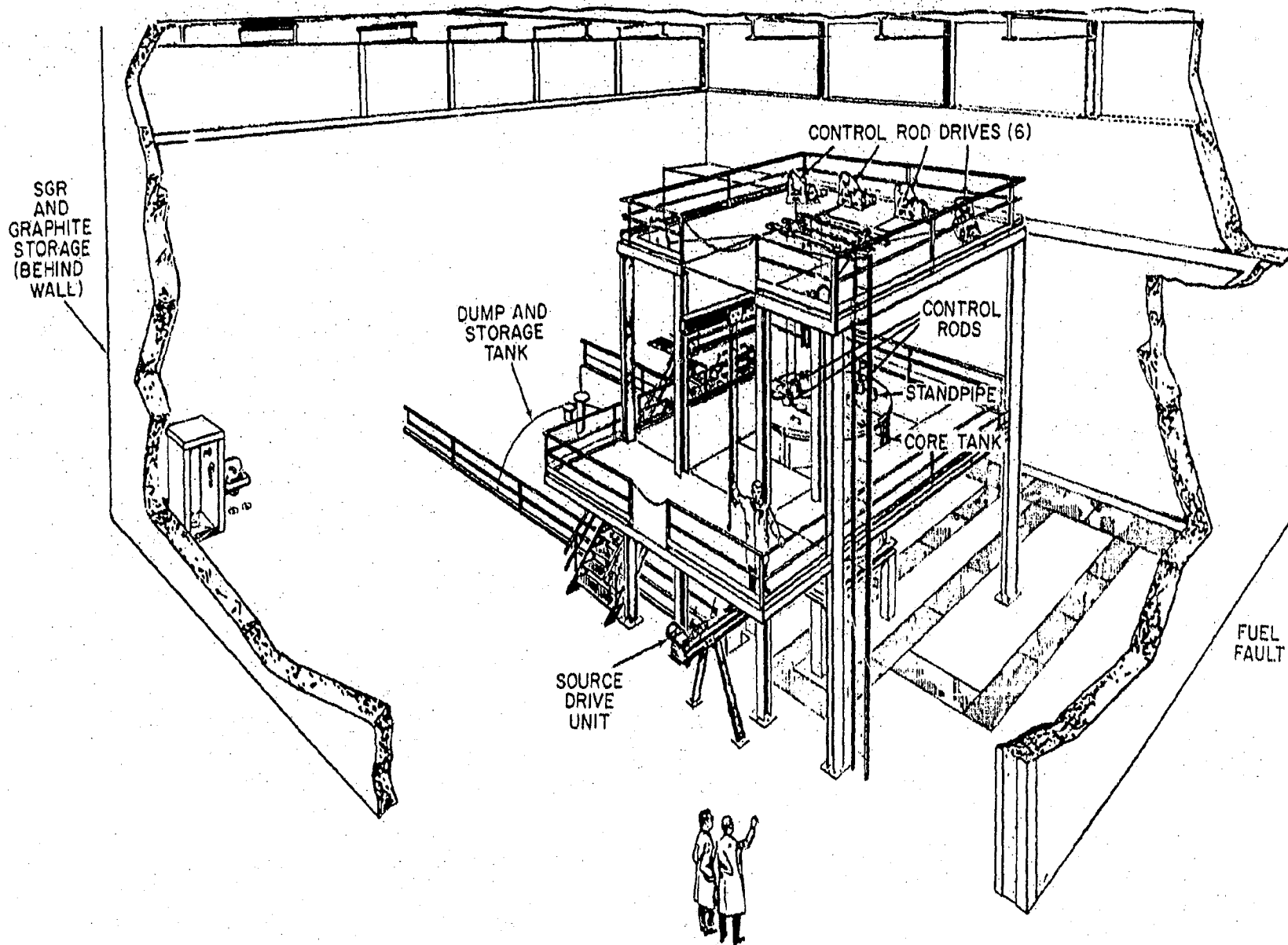
Figure V-13. Design of OMR Critical Facility
