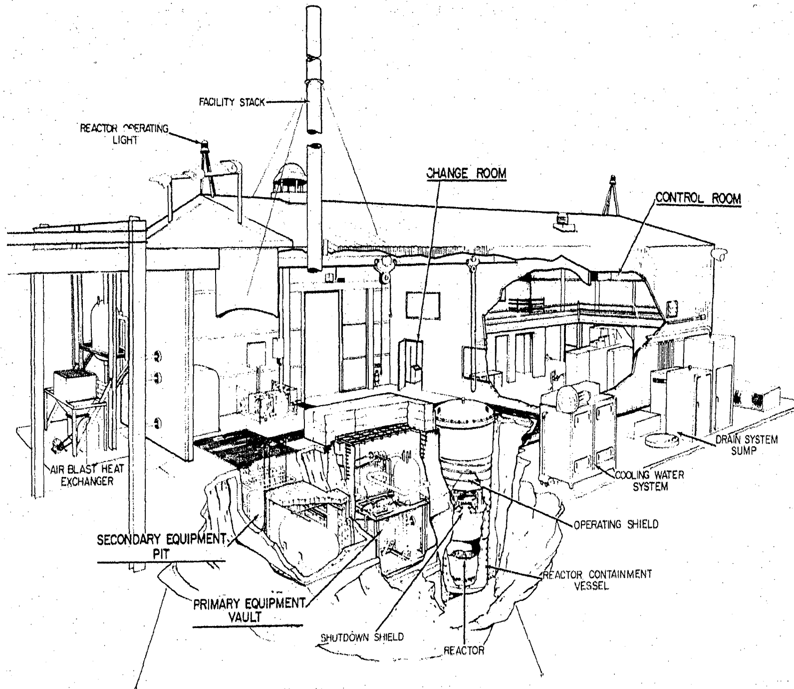
Figure V-4. Isometric View of SNAP 8 Experimental Reactor
