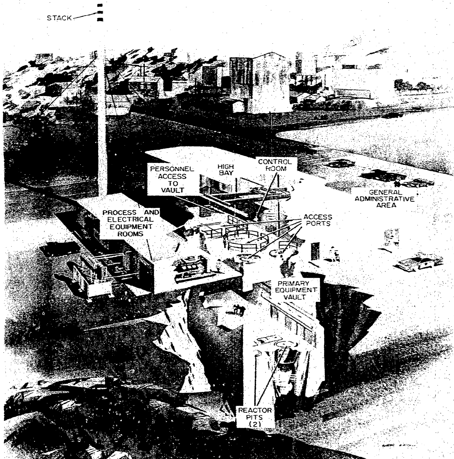
Figure V-5. Isometric View of SNAP 8 Ground Prototype Test Facility
