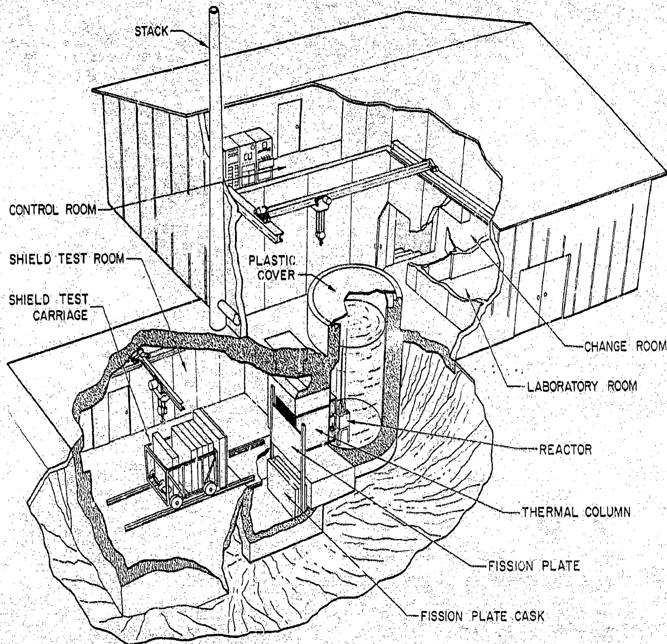
Figure V-9. Design of the Shield Test Experiment Facility
