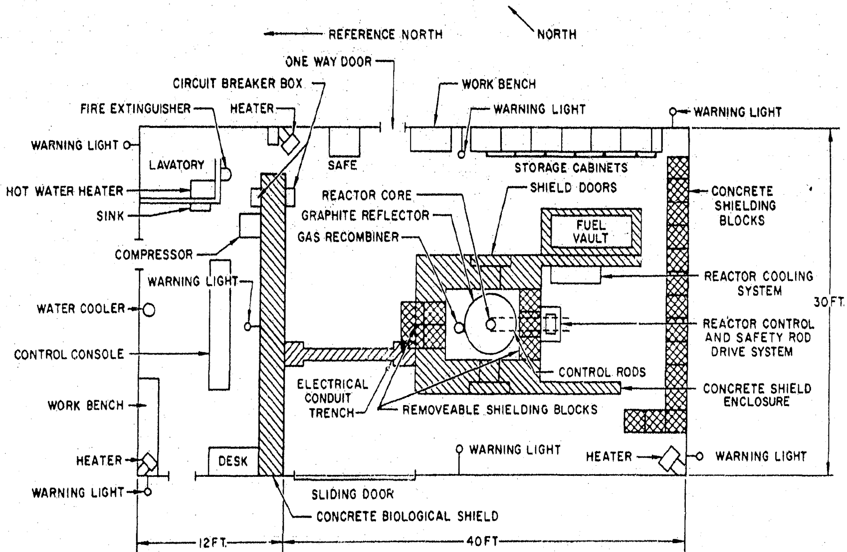
Figure V-11. Floor Plan of AE-6 Reactor Building
