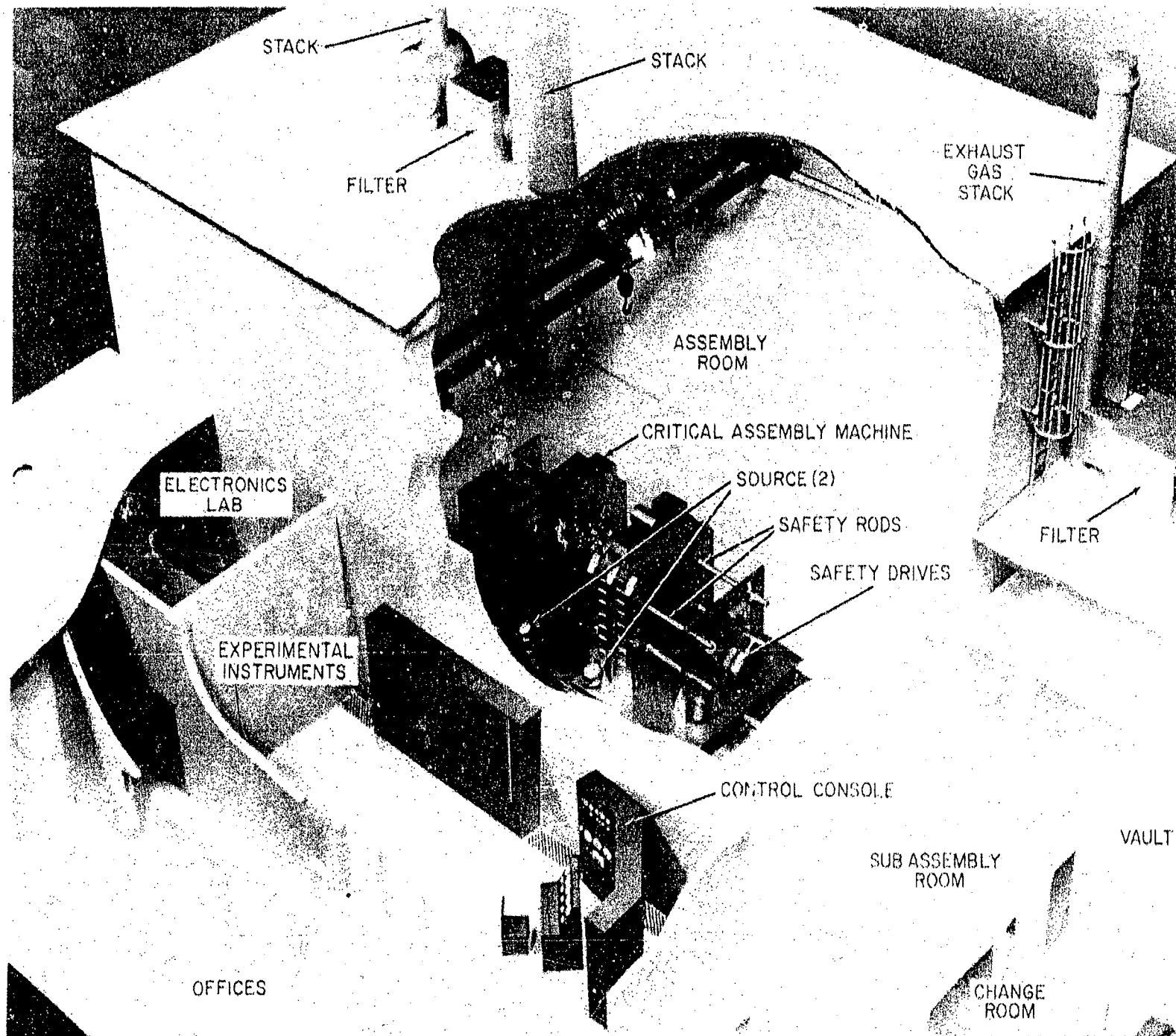
Figure V-15. Design of the Epithermal Critical Experiments Laboratory
