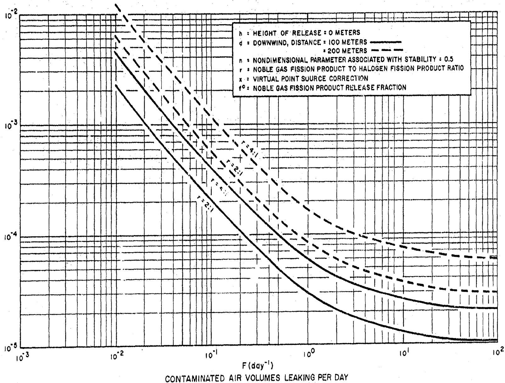
Figure III-1. Maximum Permissible Steady-State Power Level as a Function of Leakage Rate for Ground Release (Based on Dose Requirements for Site Boundary)
