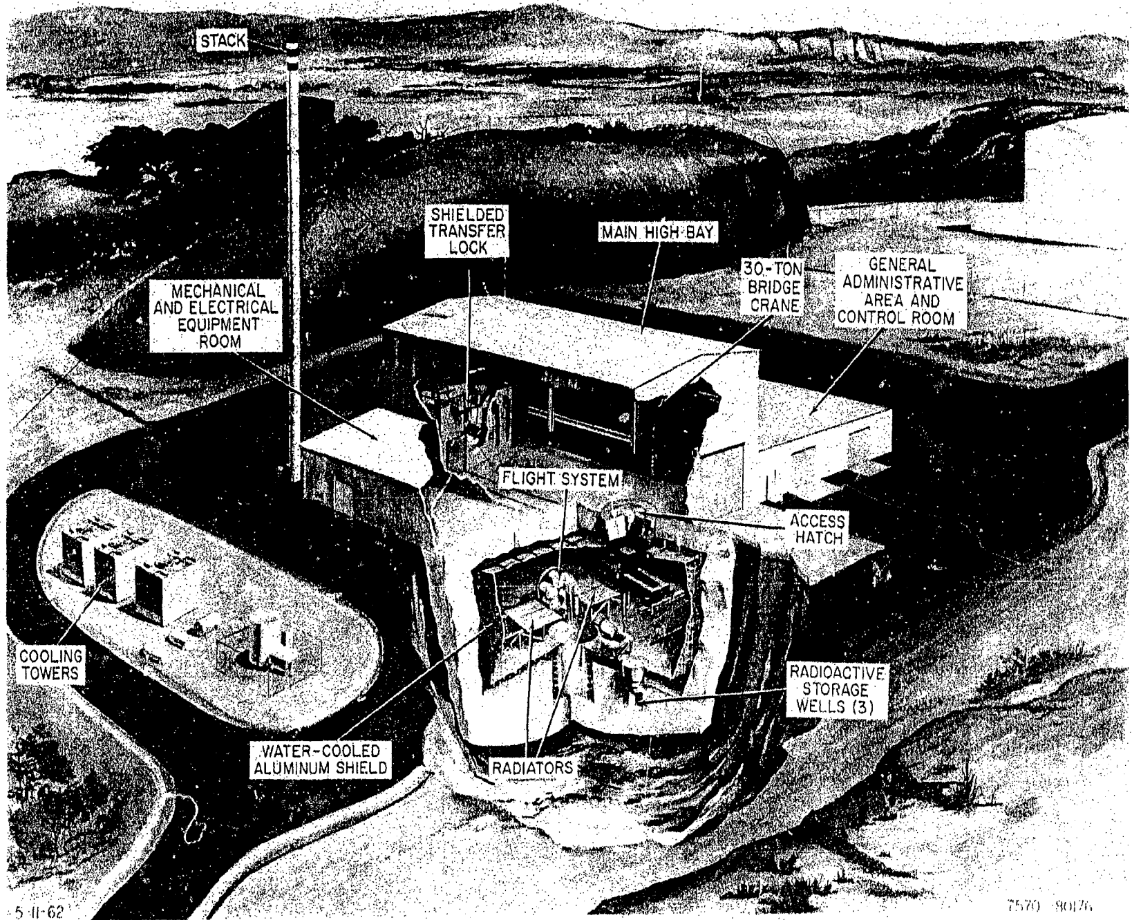
Figure V-6. Artist's Conception of SNAP 8 Flight System Test Facility
