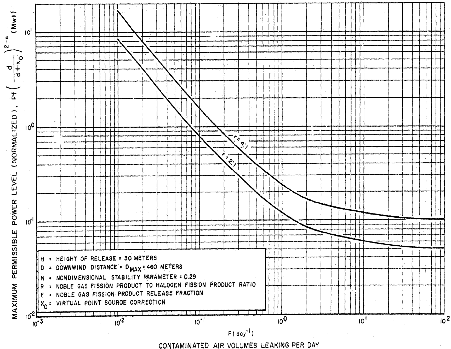
Figure III-3. Maximum Permissible Steady-State Power Level as a Function of Leakage Rate for 30 Meter Stack Release (Based on Dose Requirements for Site Boundary)
