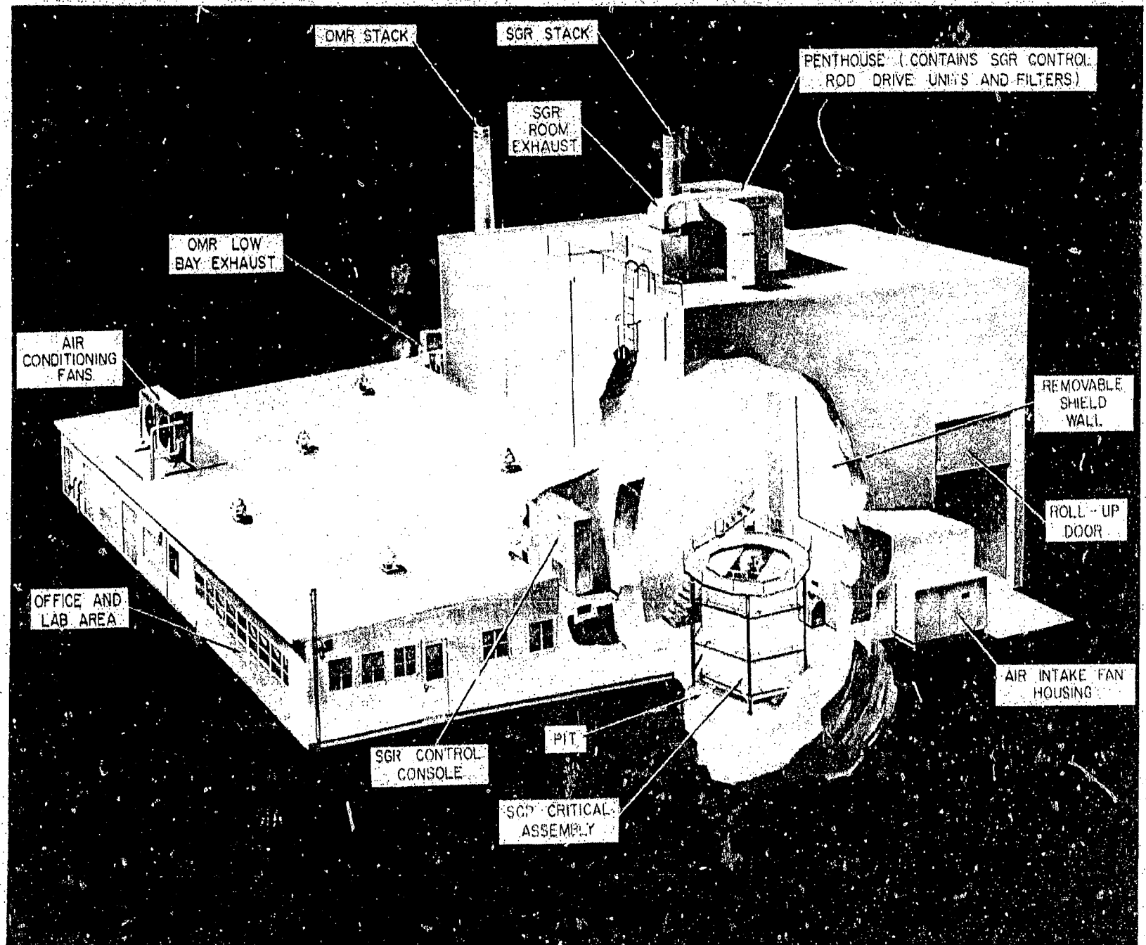
Figure V-12. Artist's Conception of SGR-OMR Critical Facility
