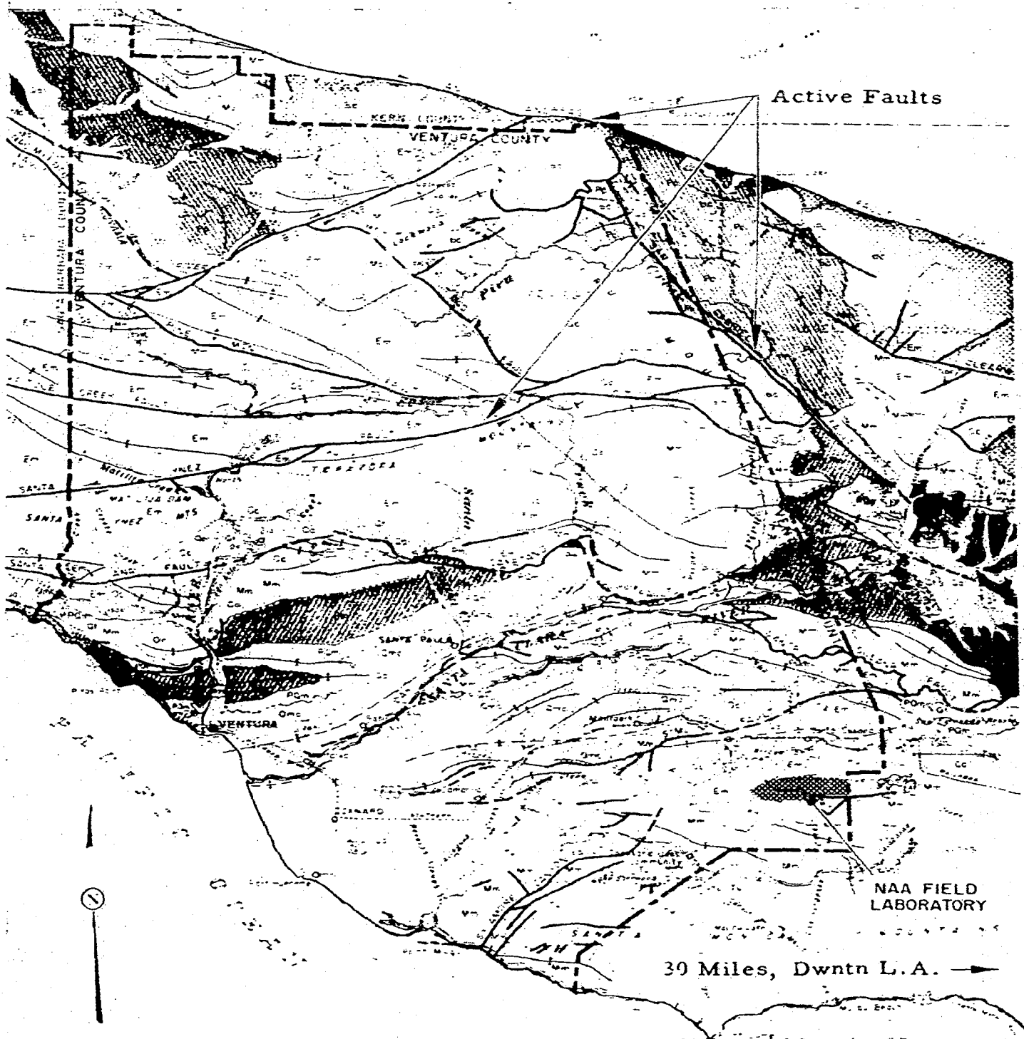
Figure II-18. Earthquake Faults in the Los Angeles Vicinity
