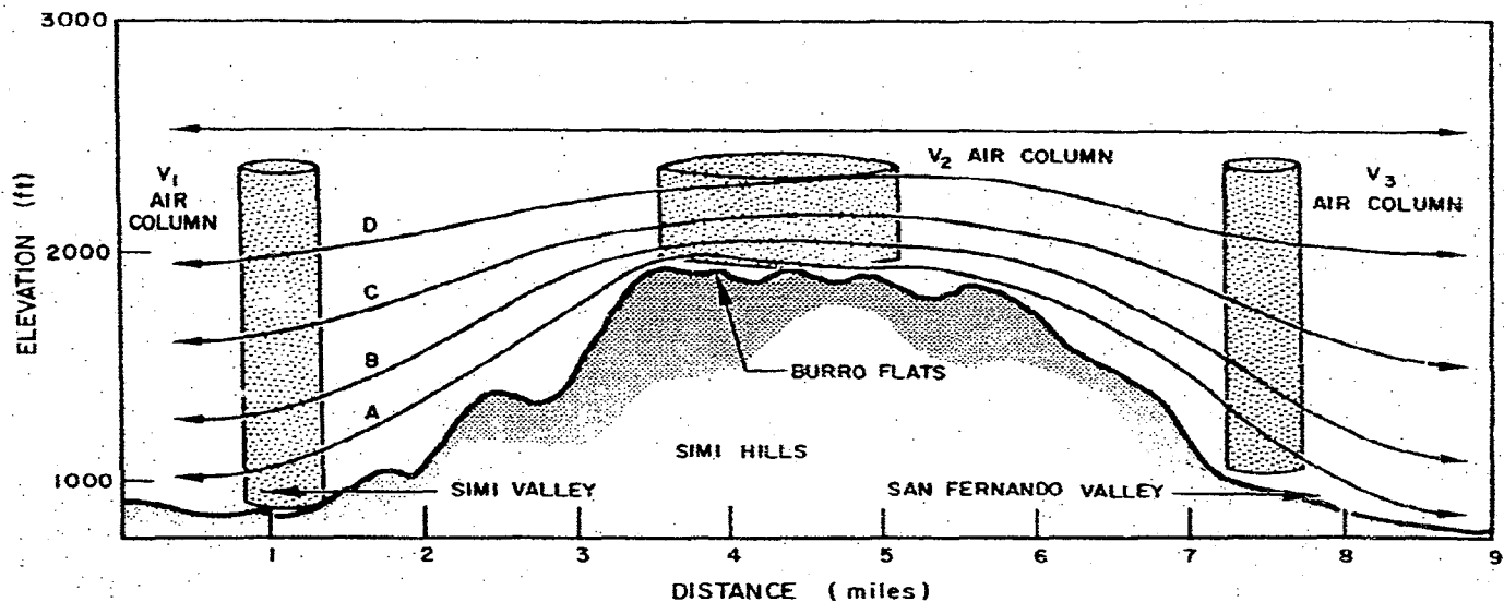
Figure II-14. Representative Air Flow Across Simi Hills
