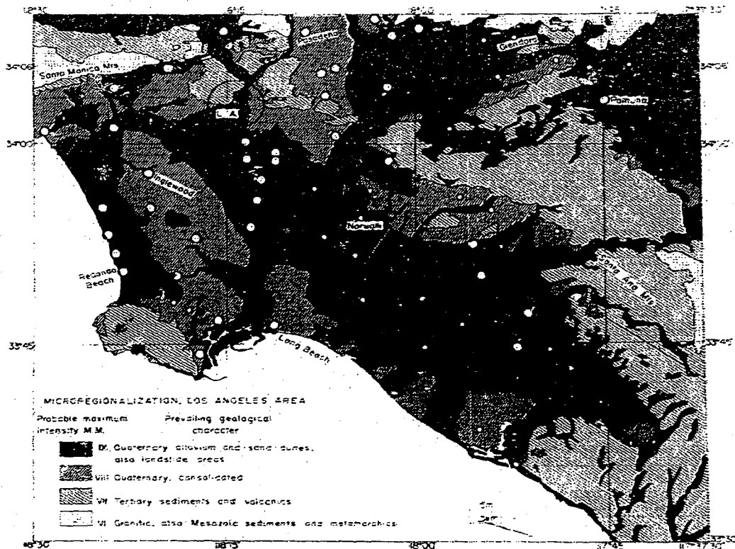
Figure II-20. Seismic Microregionalization Map of the Los Angeles Basin and Vicinity
