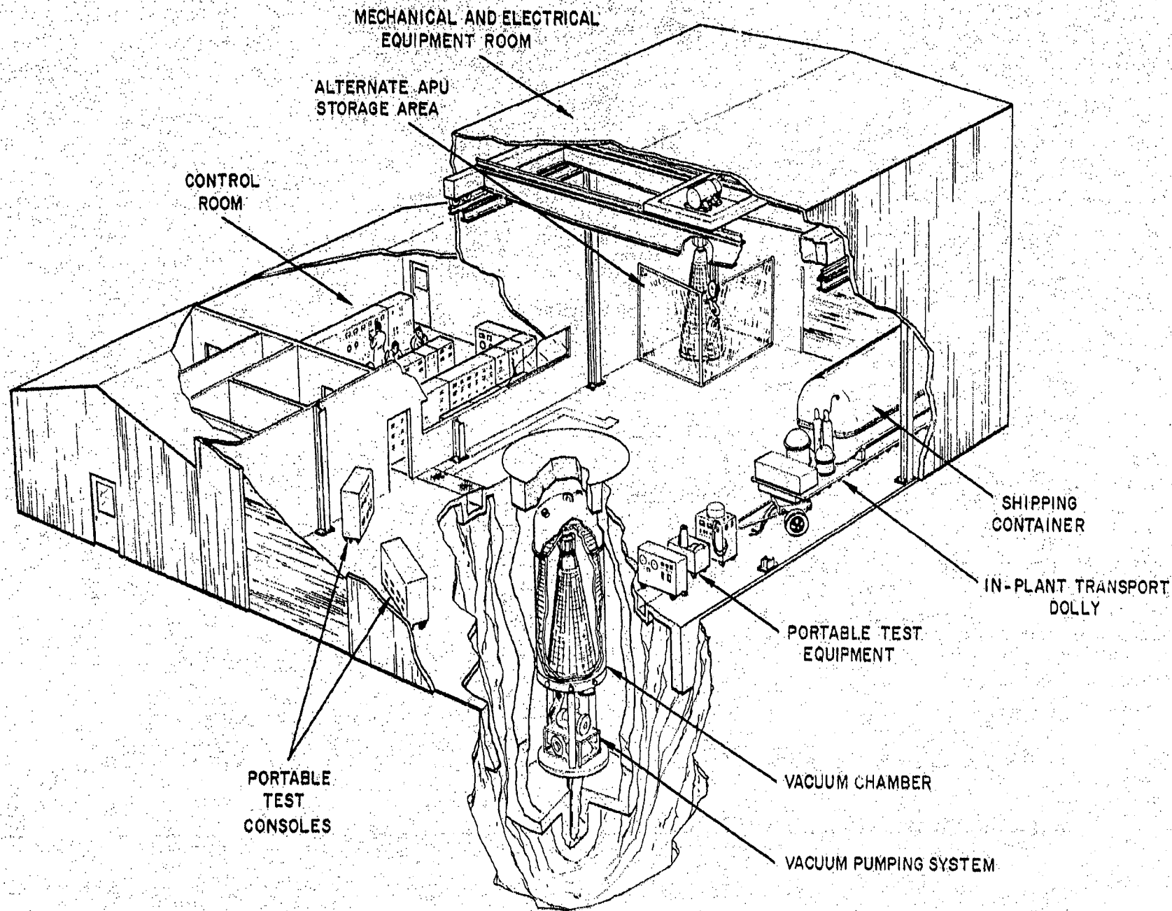
Figure V-8. Design of the Flight Systems Nuclear Qualifications Test Facility
