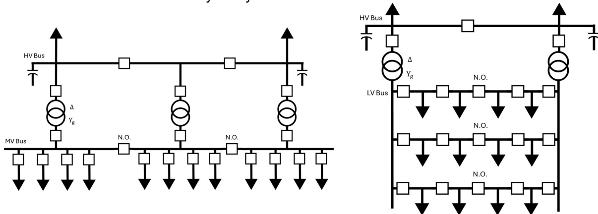
Figure 7: Exemplar substation layouts for data center HV substations.
