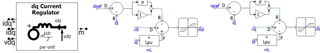
Figure 45: Icon (Left) and Main Controls (Center, Right) for the ireg Component.
