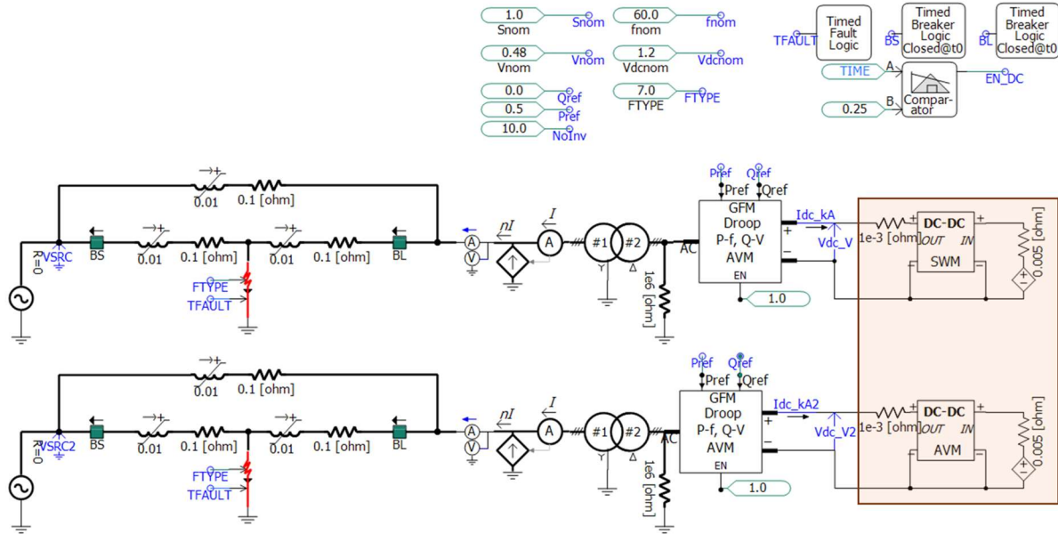
Figure 32: Overview of DML_DC_DC_Demo Model.
