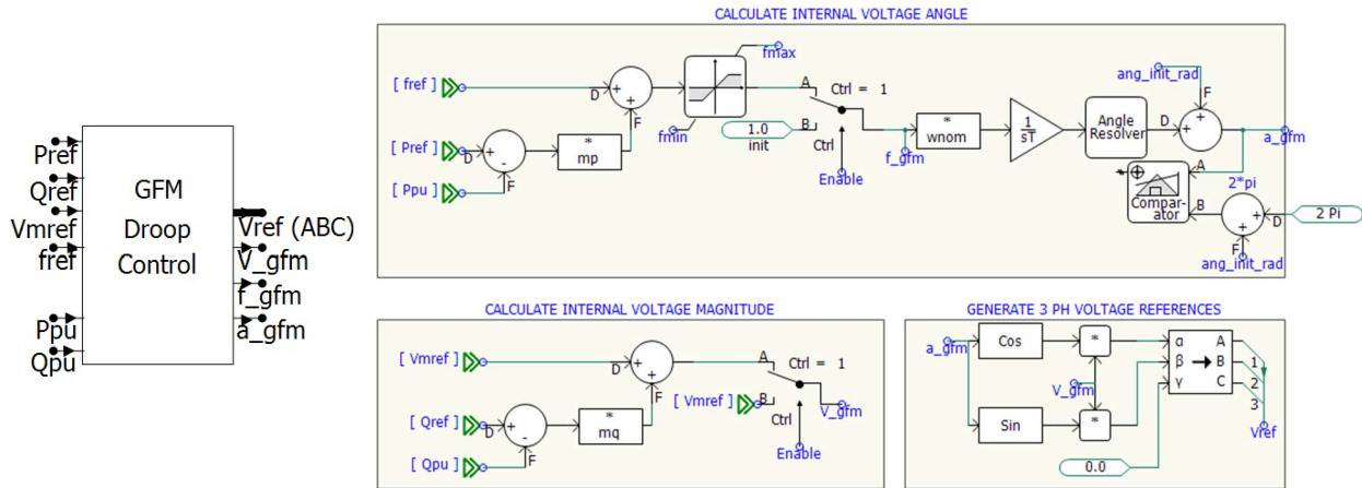
Figure 43: Icon (Left) and Main Control Elements (Right) for the gfm_droop Component.
