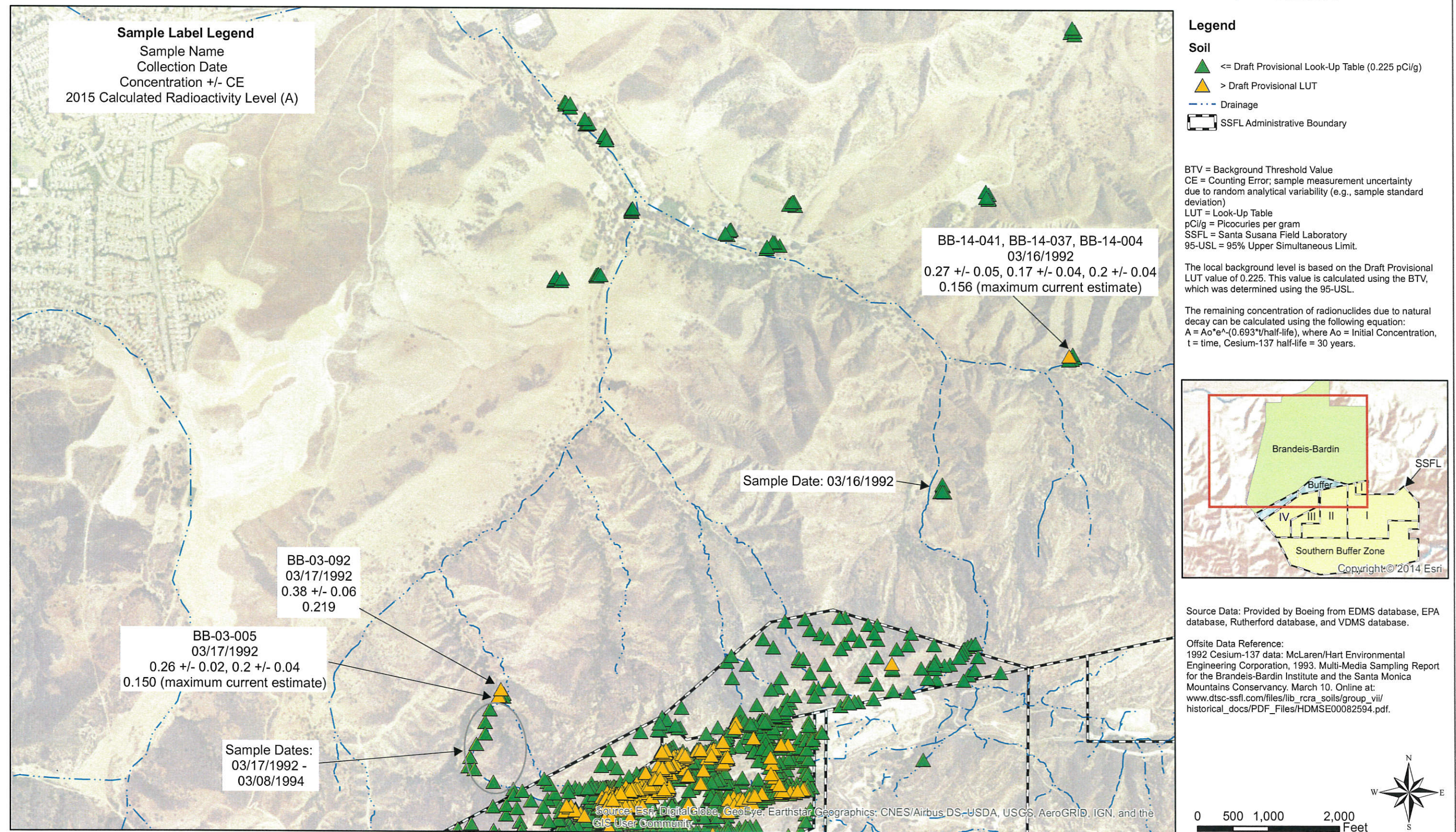
Figure 4 - Cesium-137 (pCi/g) Soil Analytical Data Compared to SSFL Local Background Level
