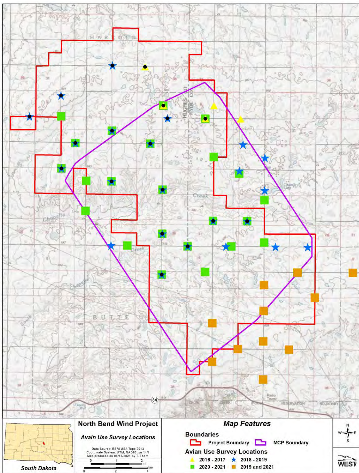
Figure 3. Location of fixed-point avian use survey stations completed in from 2016-2021 throughout the North Bend Wind Project boundary located in Hughes and Hyde counties, South Dakota. The MCP Boundary (purple outline) encapsulates the final proposed turbine layout.
