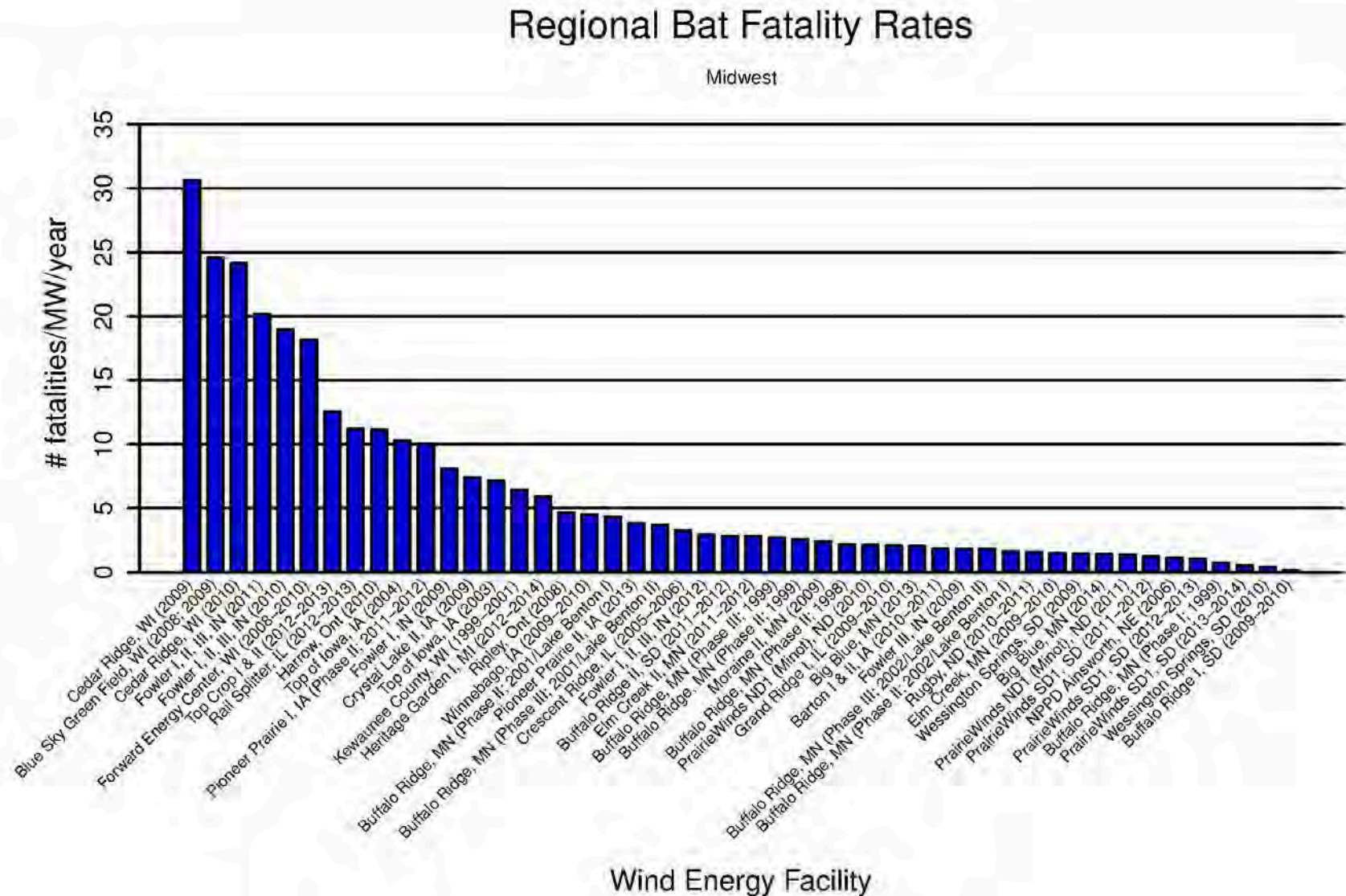
Figure 8. Fatality rates for bats (number of bats per megawatt per year) from publicly available studies at wind energy facilities in the Midwest.
