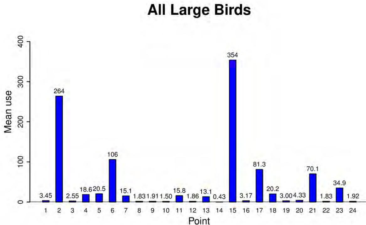
Figure 4a. Relative large bird use (birds/800-meter plot/60-minute survey) by observation point during avian use surveys at the Triple H Wind Project from April 18, 2016 to March 28, 2017.
