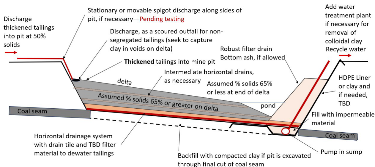
Schematic 1 Tailings Impoundment Conceptual Design – Cross-Section
