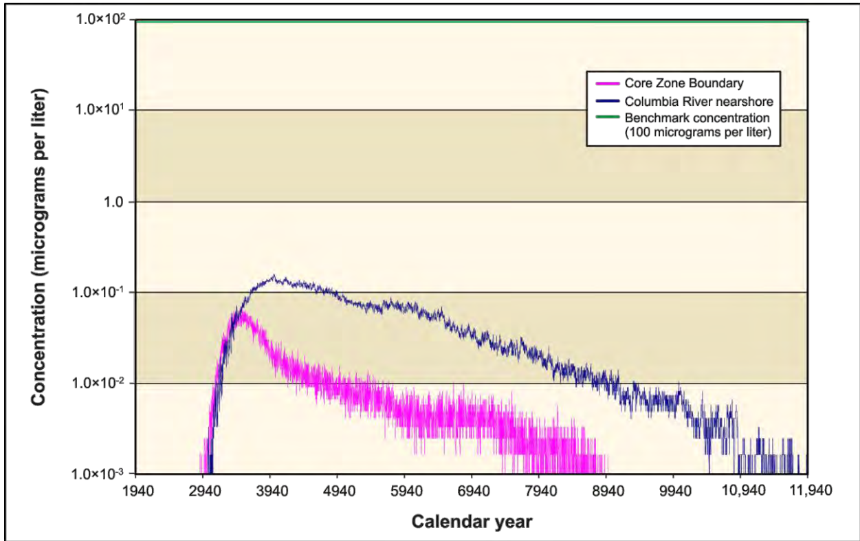
Figure 5–366. Waste Management Alternative 1 Chromium Concentration Versus Time
