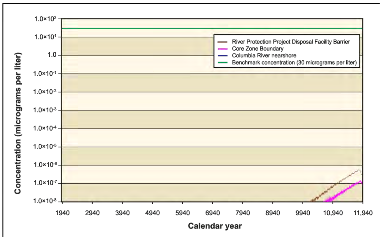
Figure 5–425. Waste Management Alternative 2, Disposal Group 1, Subgroup 1-B, Total Uranium Concentration Versus Time
