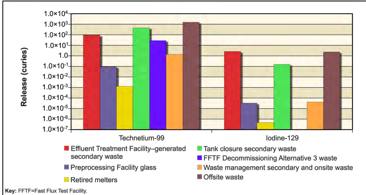
Figure 5–655. Waste Management Alternative 2, Disposal Group 3, Option Case, Radionuclide Releases from 200-East Area Integrated Disposal Facility to Vadose Zone
