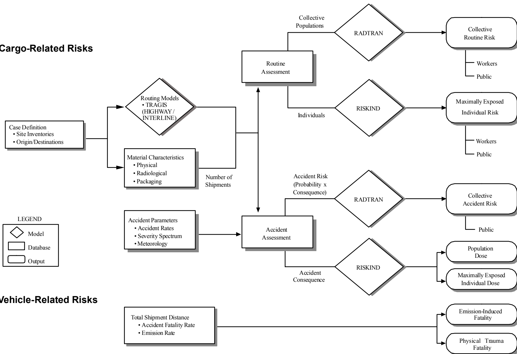
Figure 4.1. Technical Approach for Transportation Radiological Risk Assessments
