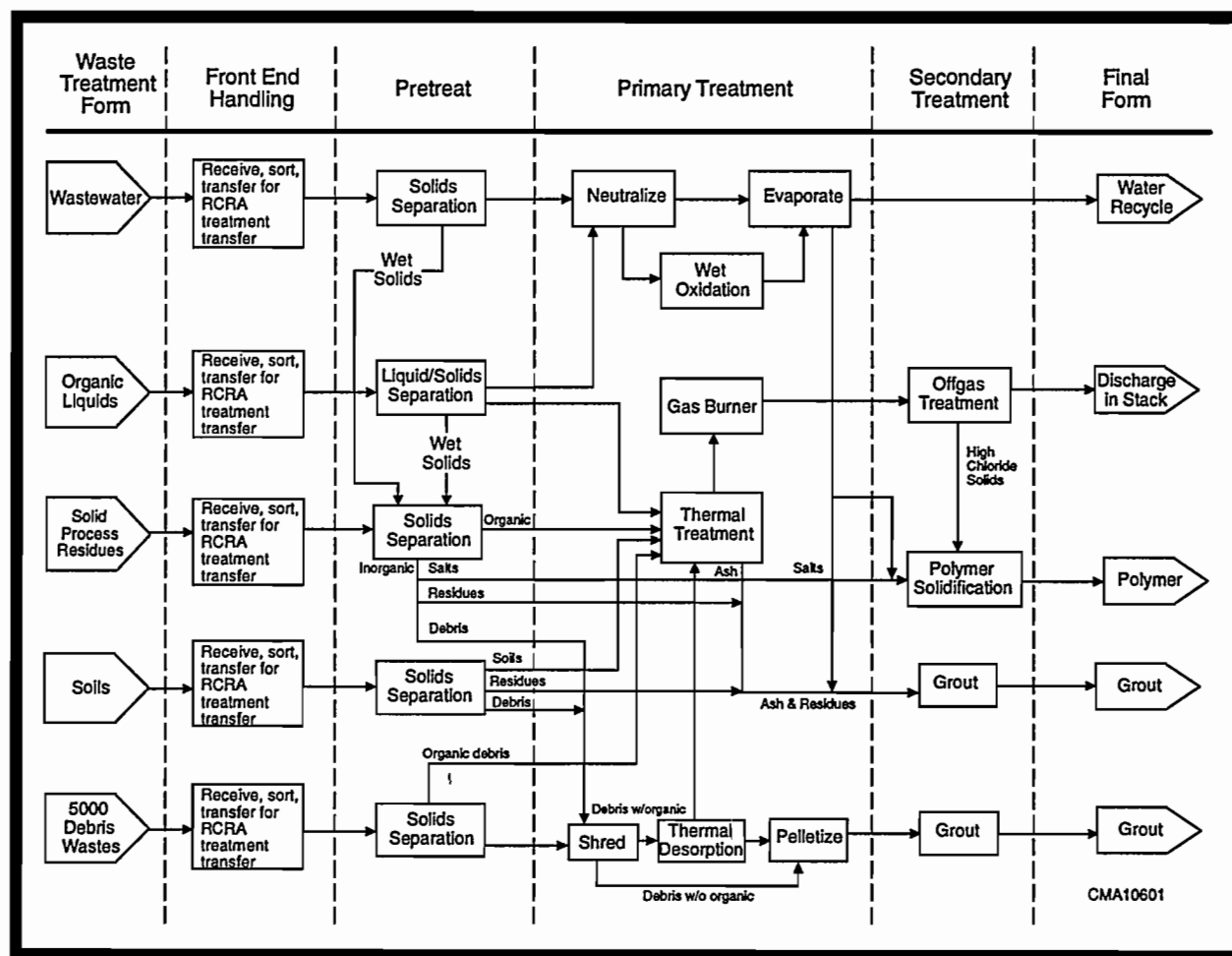
Figure 6.2-1. WM PEIS LLMW Flow Diagram
