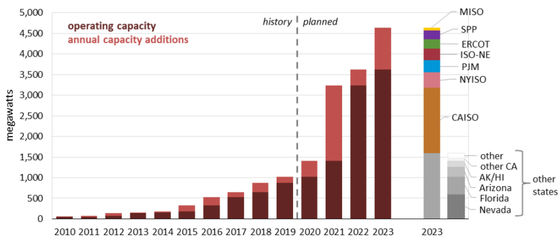
Figure I.3: United States BPS-Connected Battery Energy Storage Power Capacity (July 2020) 4
