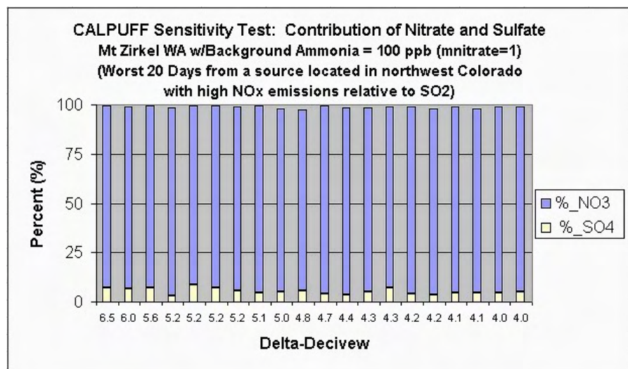
Figure 16. Contribution of sulfate and nitrate to the modeled change in deciview, assuming a background ammonia of 100 ppb in CALPUFF.
