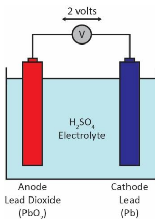
Figure I.1: Schematic of a Battery
