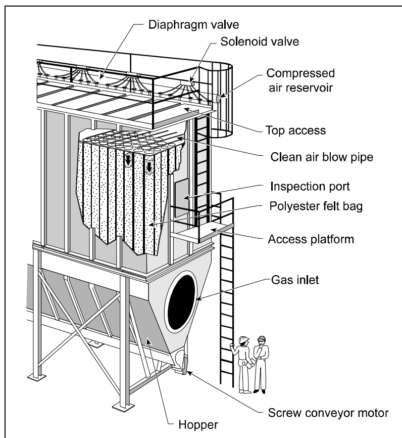
Figure 5-1. Design considerations for a pulse-jet baghouse
