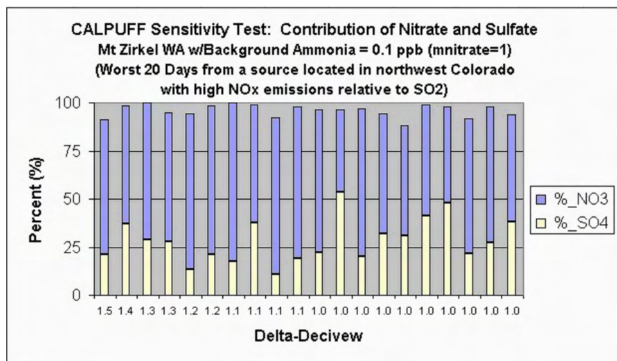
Figure 15. Contribution of sulfate and nitrate to the modeled change in deciview, assuming a background ammonia of 0.1 ppb in CALPUFF.
