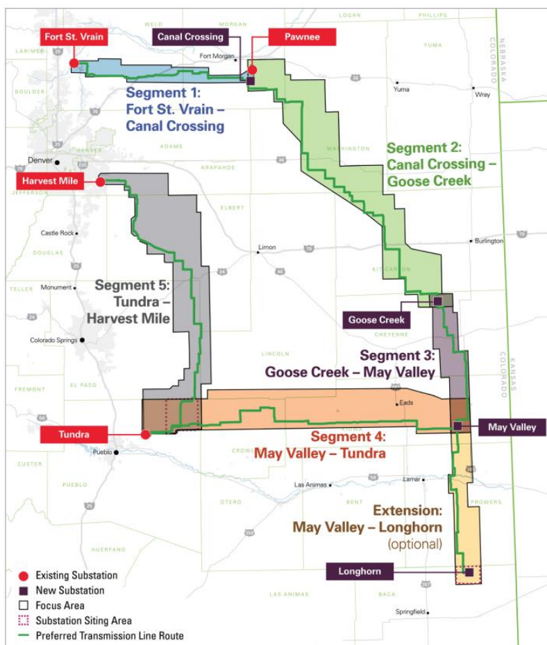
Figure 10. Colorado’s Power Pathway Transmission Investment
