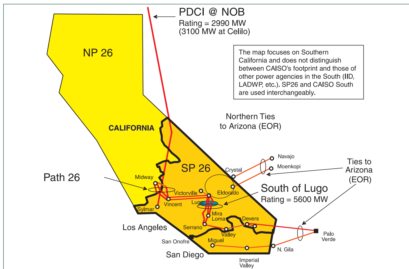
Figure 5-3. Southern California: Major Transmission into SP26
