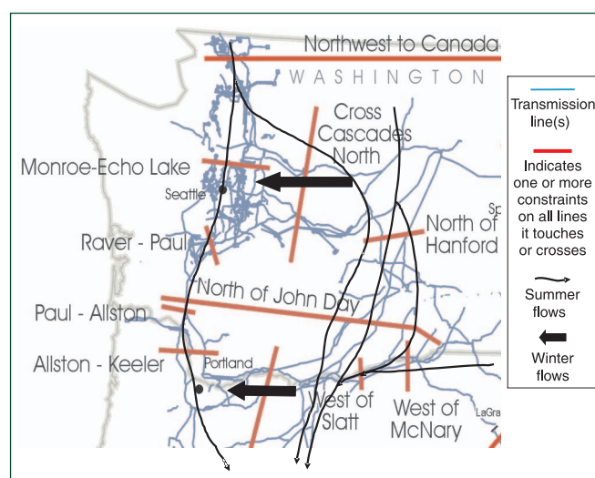
Figure 5-4. Congested Paths and Seasonal Power Flows in the Pacific Northwest
