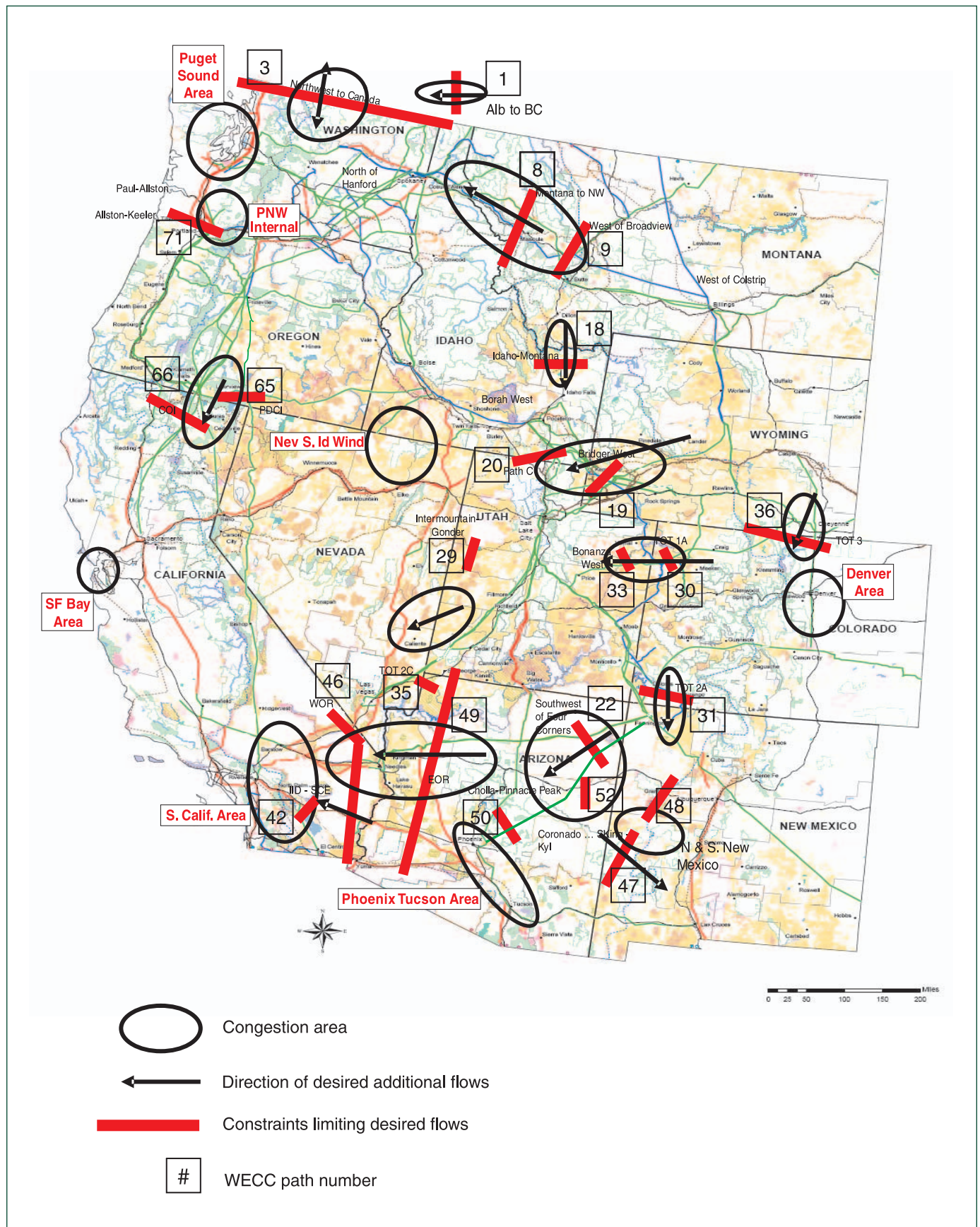
Figure 4-7. Existing and Projected Major Transmission Constraints in the Western Interconnection
