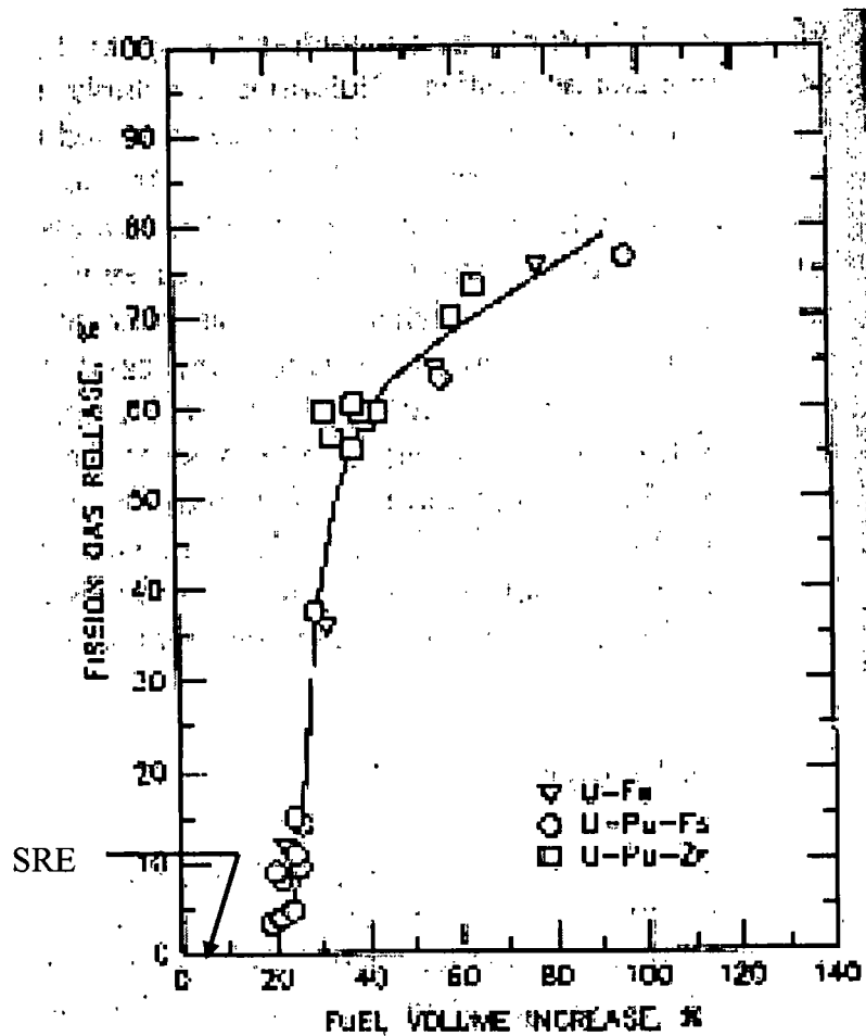
Fig. 3. Fission-Gas Release Versus Fuel-Volume Increase (Beck, 1968).
