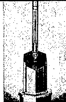
Fig. 31—Model of the SRE 7-rod fuel element showing its position within the central channel of the moderator assembly (SRE Photo 31)
