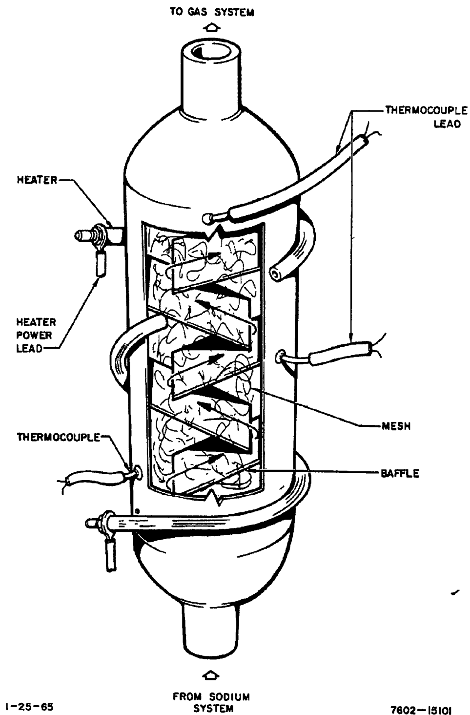
Figure 3-37 Vapor Trap
