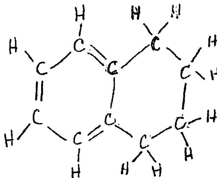
Figure 7. Tetralin molecule, 1,2,3,4-tetrahydronaphthalene, C_{10}H_{12} , melting point -35.8^{\circ}\text{C} , boiling point 207.6^{\circ}\text{C} . Used for cooling reactor components.
