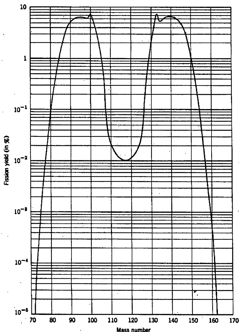
Fig. 10-7 Yields of fission-product chains as a function of mass number for the slow-neutron fission of U^{235} .
