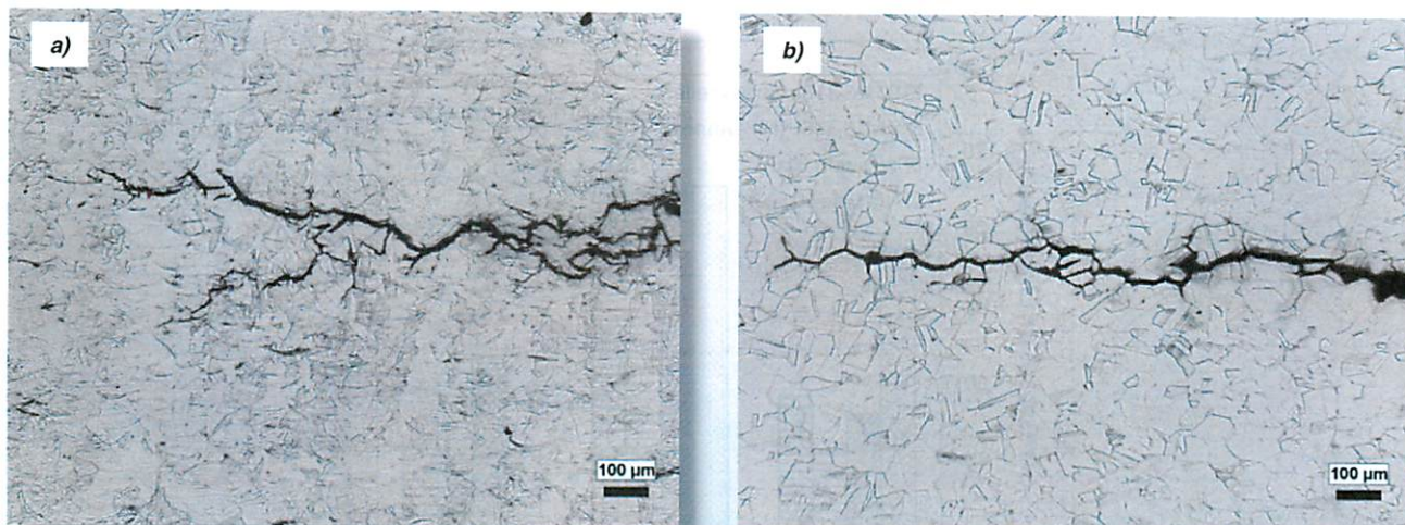
Figure 2. Cross-sectional image of stress corrosion crack on DMLM316L stainless steel after SCC test.
