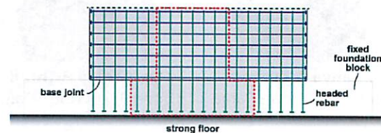
Figure 4. Vertical wall slice from capstone wall as basis of a deep beam specimen.
