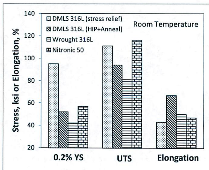
Figure 3. Mechanical property comparison among different stainless steels.
