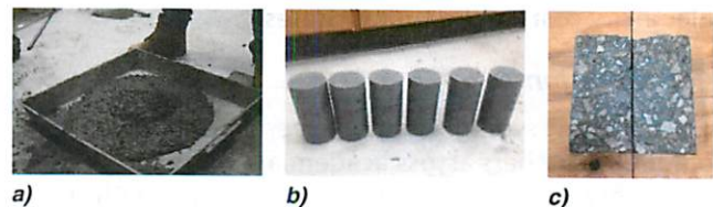
Figure 2. Properties of high-strength concrete: (a) slump, (b) compression cylinders (before testing), (c) tension cylinder (after testing)
