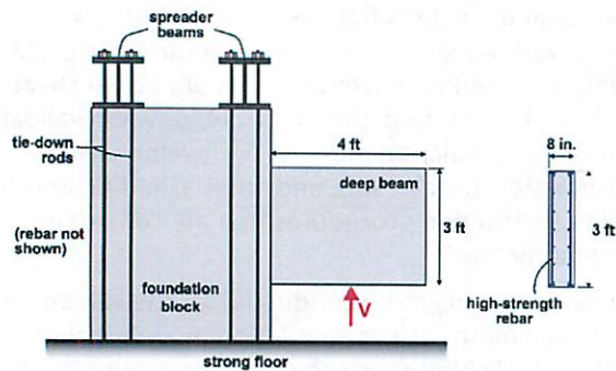
Figure 3. Preliminary elevation (left) and cross-section (right) views of deep beam specimens
