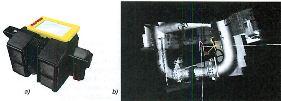
Figure 2. Phase II handheld 3D video camera (a) will be coupled with optimized registration software to create near real-time as-built models of large plant areas. Preliminary testing with DotProduct's Phi3D software created a registered point cloud (b) in less time than it took to take the data (4 sec registration for 10 sec of data).
