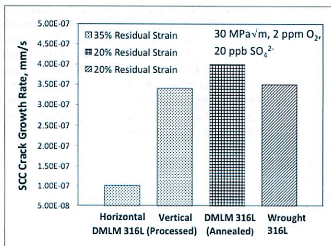
Figure 1. Stress corrosion crack growth rate comparison among different stainless steels.
