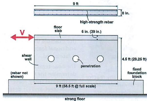
Figure 5. Preliminary cross-section (top) and elevation (bottom) views of reduced-scale capstone shear wall specimens.
