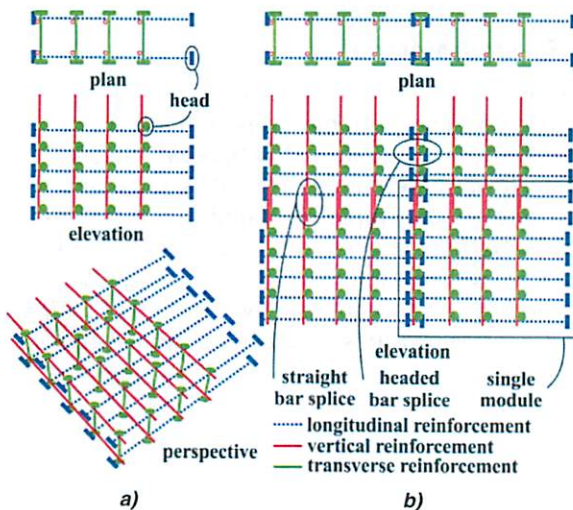
Figure 1. Prefabricated rebar cages: (a) single module, (b) four field-tied modules.
