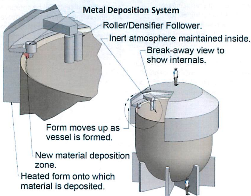
Figure 1. Concept of fabrication of large pressure vessel.
