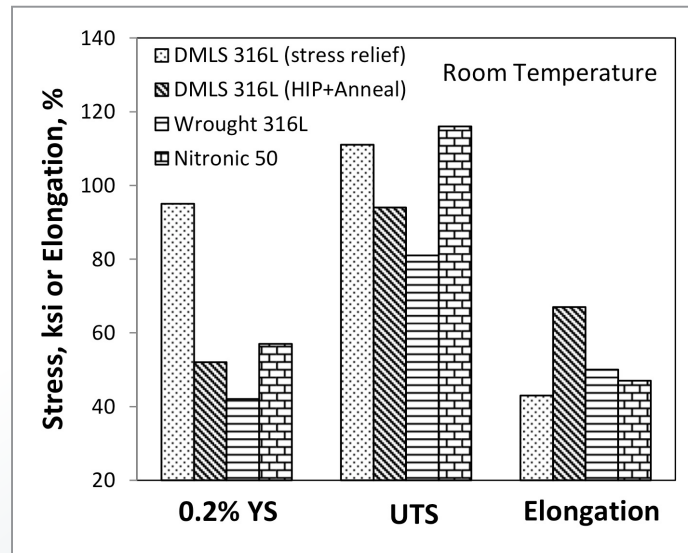
Figure 3. Mechanical property comparison among different stainless steels.
