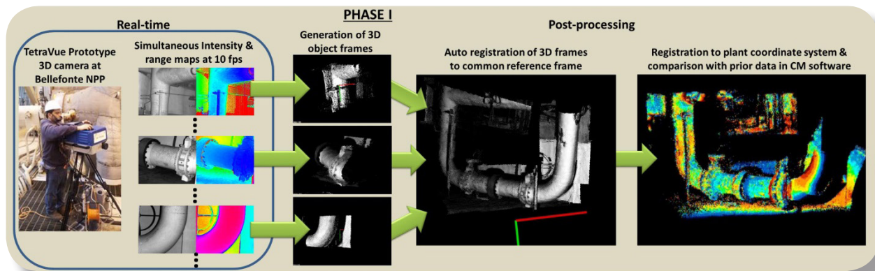
Figure 1. Phase I has demonstrated path to collect frames of intensity and range maps, convert to 3D frames, register these frames together, and then compare with design or prior as-built information in an NPP. This demonstration will be made robust and practical in Phase II.
