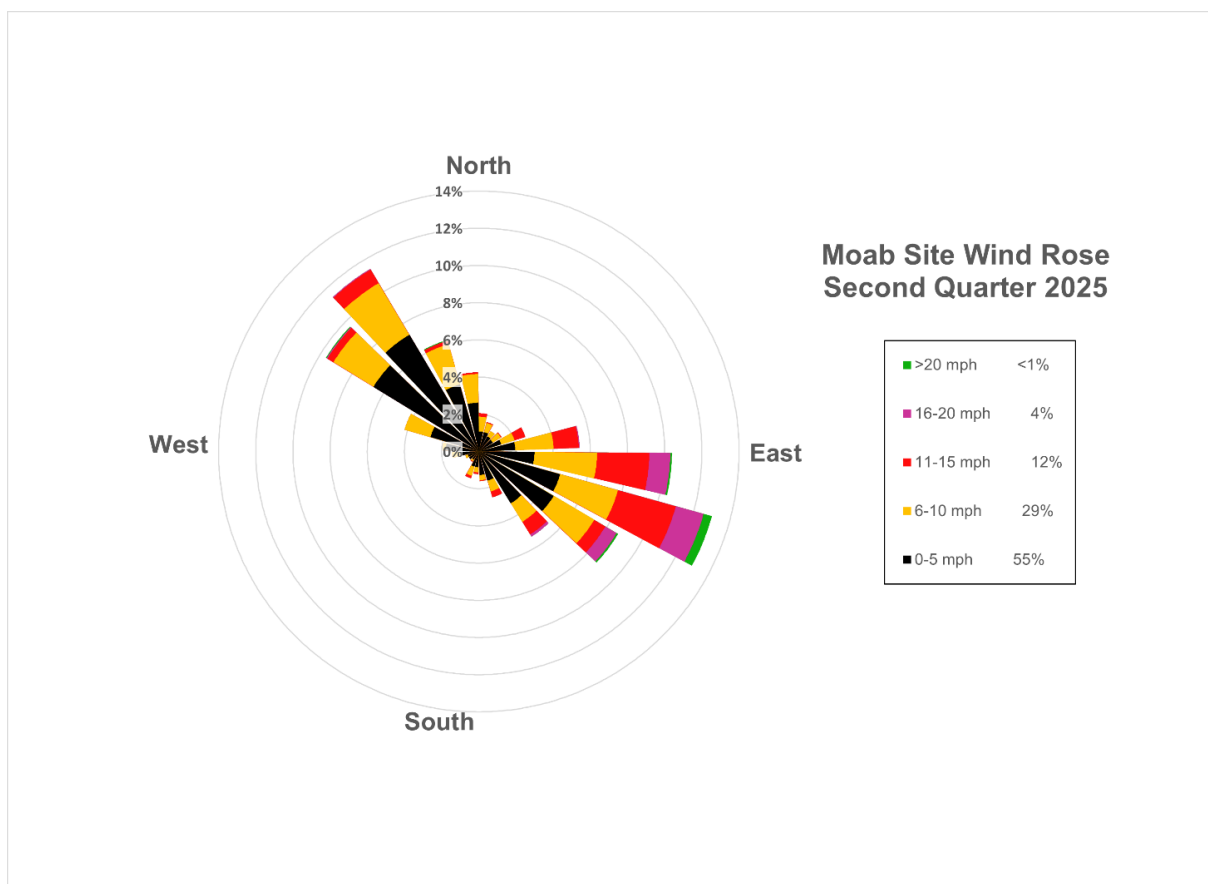
Figure 4. Moab Wind Rose for Second Quarter 2025
