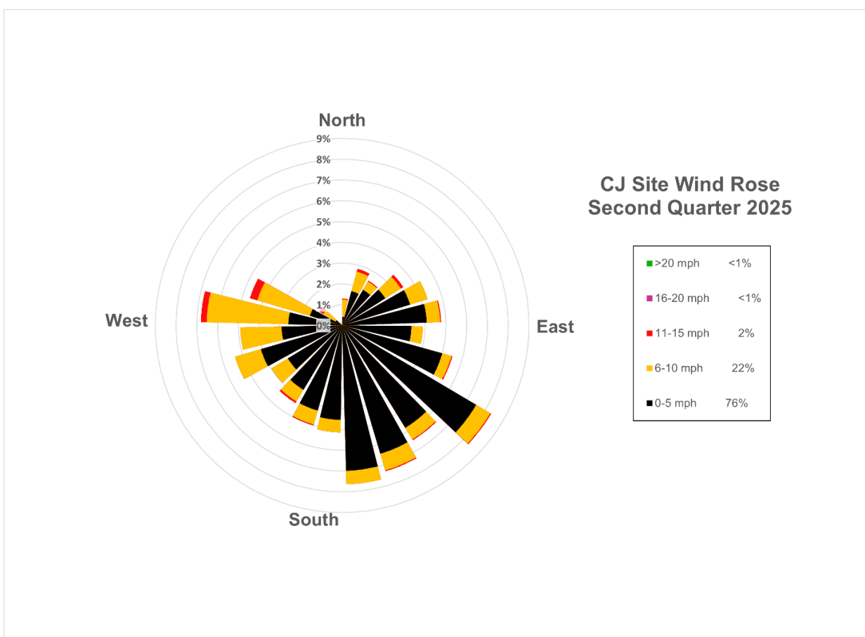
Figure 5. Crescent Junction Wind Rose for Second Quarter 2025
