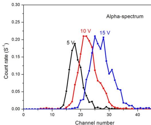
Alpha spectra by GaN at reactor
