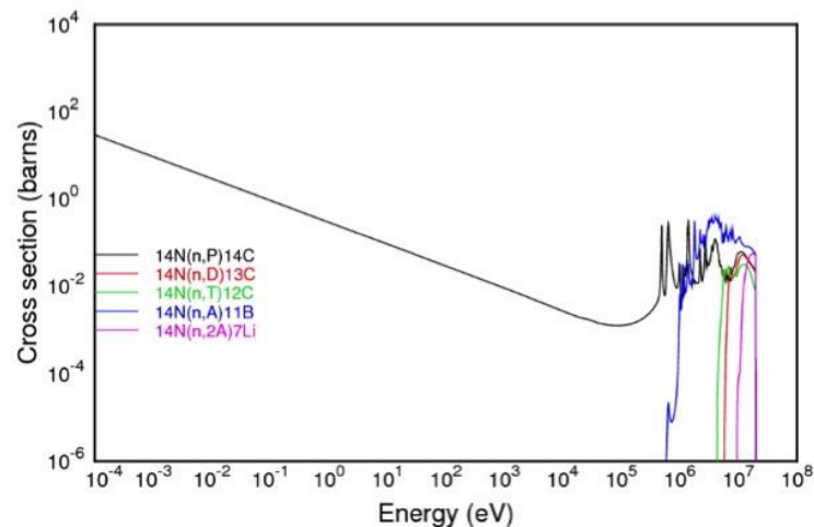
^{14}\text{N} Cross Sections Various Reactions
