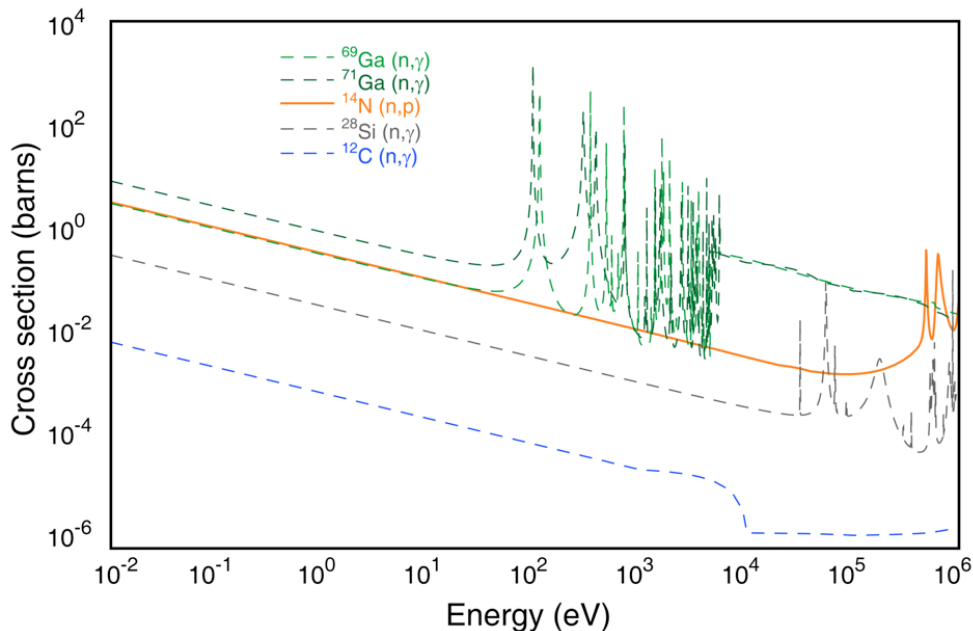
Semiconductor Transmutation Reactions in GaN and SiC
