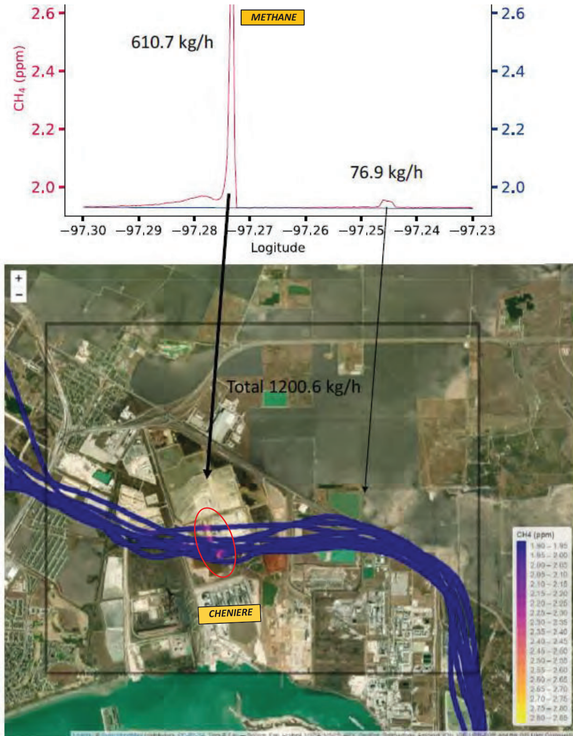
Figure 19b: Atmospheric \text{CH}_4 concentrations and \text{CH}_4 fluxes (97.23°W to 97.30°W, black rectangle) from the Ingleside-Gregory during the flight on January 6, 2023.
