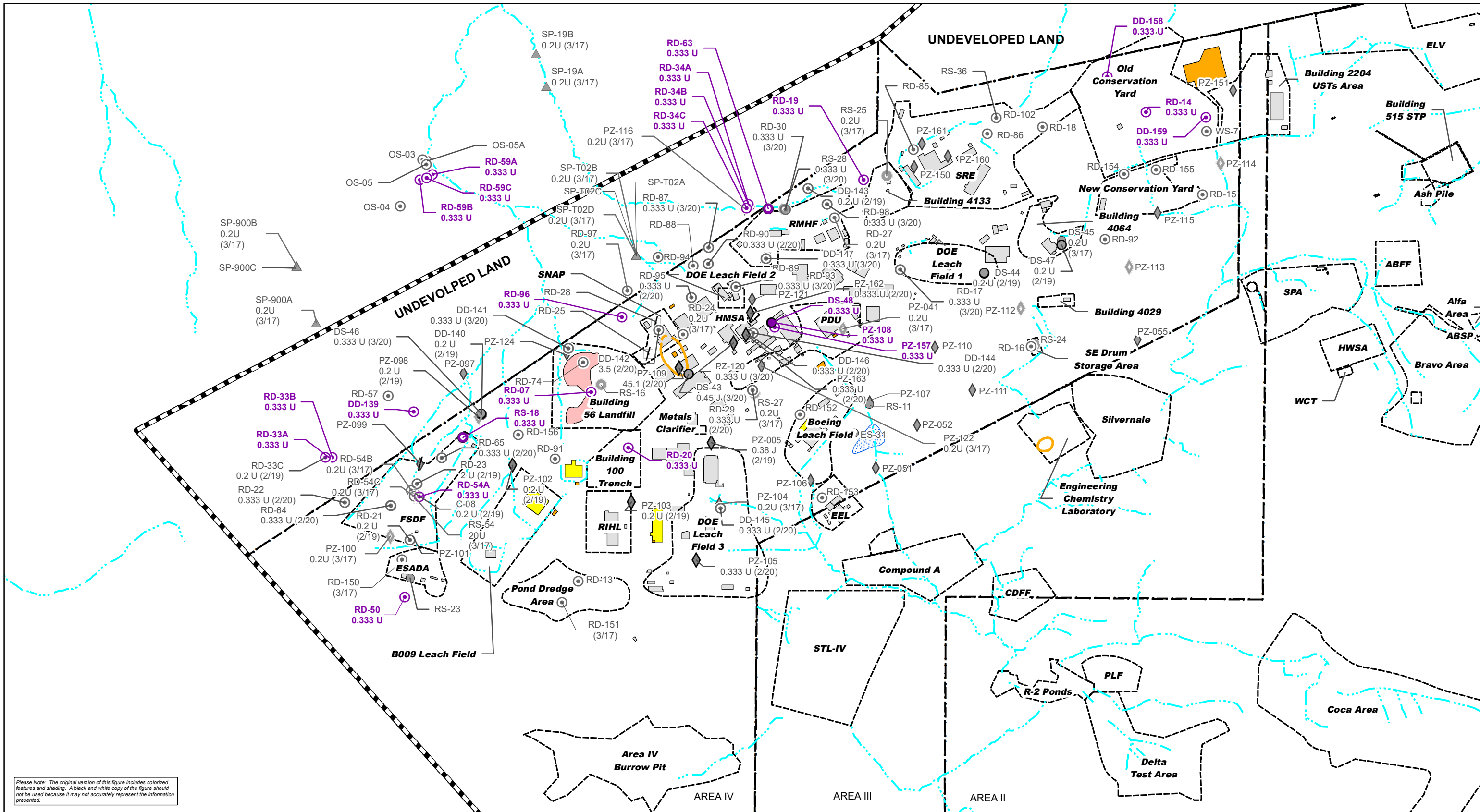
SANTA SUSANA FIELD LABORATORY VENTURA COUNTY, CALIFORNIA AREA IV EXTENT OF TETRACHLOROETHENE IN GROUNDWATER, 2021 FIGURE 7
