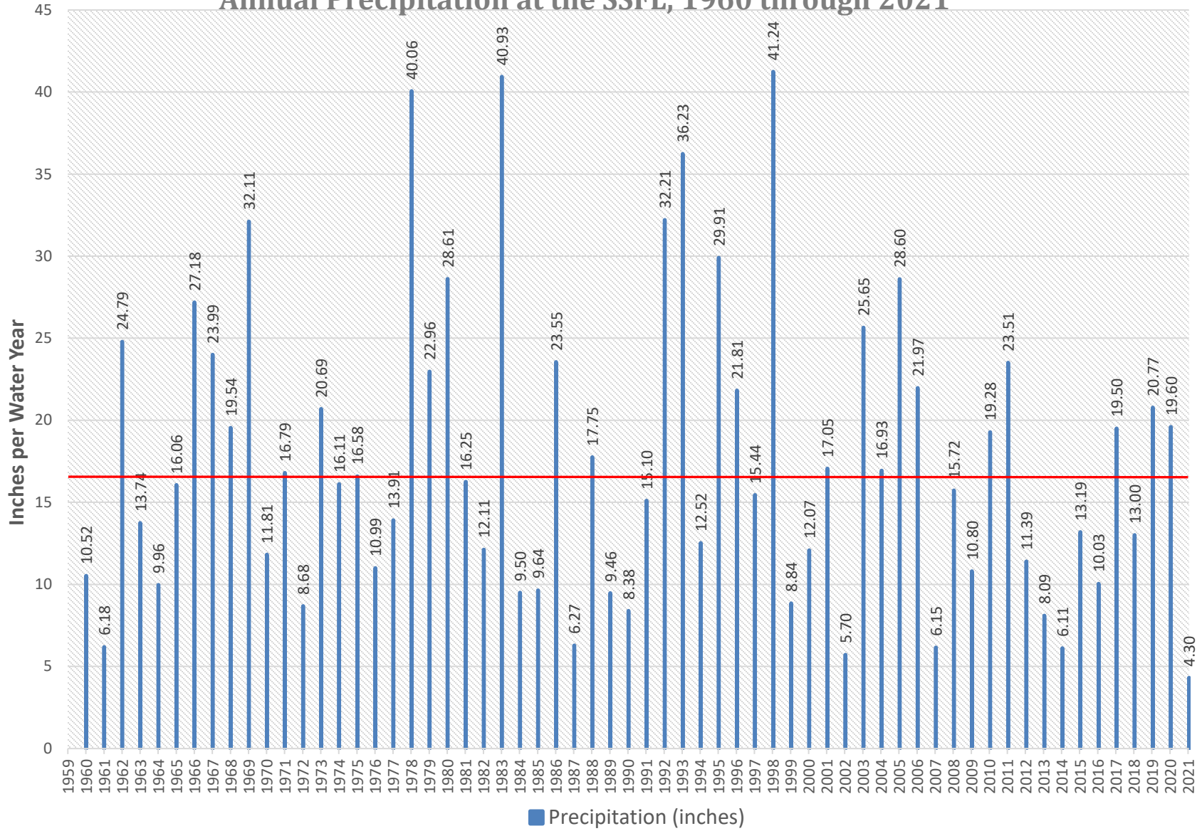
Figure B-1 Annual Precipitation at the SSFL, 1960 through 2021
