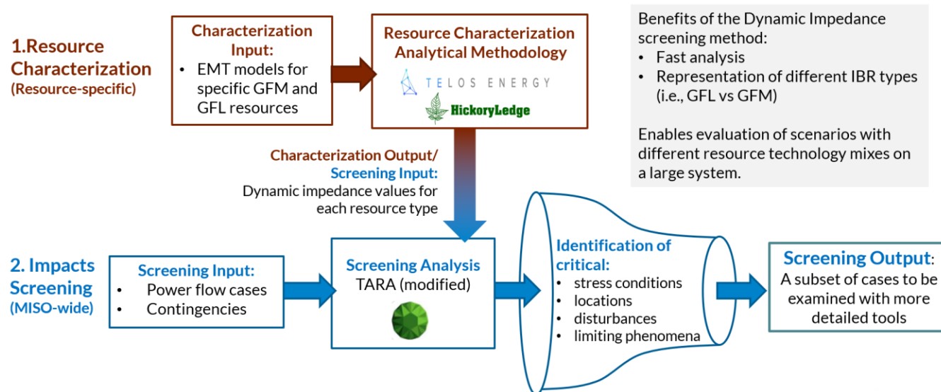
Figure C-13. Process diagram of the Dynamic Impedance screening method
