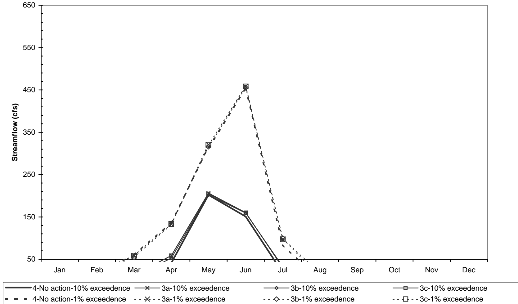
Simulated High-Flow, Low-Frequency Streamflow, 1904-2002 - Lower Reach Salmon Creek No Action vs OID Water Rights Purchase Alternative
