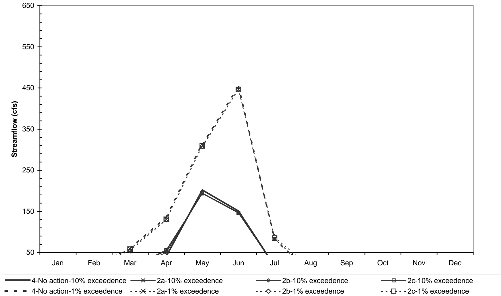
Simulated High-Flow, Low-Frequency Streamflow, 1904-2002 - Lower Reach Salmon Creek No Action vs Upgrade Shellrock Pumping Plant Alternative
