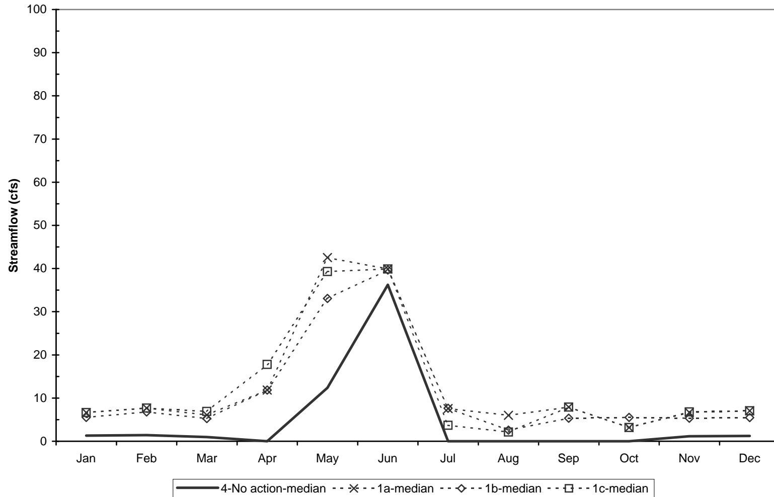
Simulated Median Streamflow, 1904-2002 - Lower Reach Salmon Creek No Action vs Okanogan River Water Exchange Alternative
