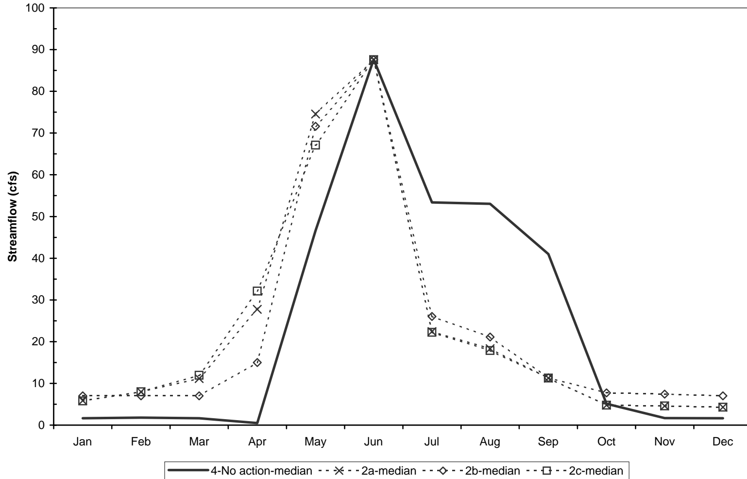
Simulated Median Streamflow, 1904-2002 - Middle Reach Salmon Creek No Action vs Upgrade Shellrock Pumping Plant Alternative
