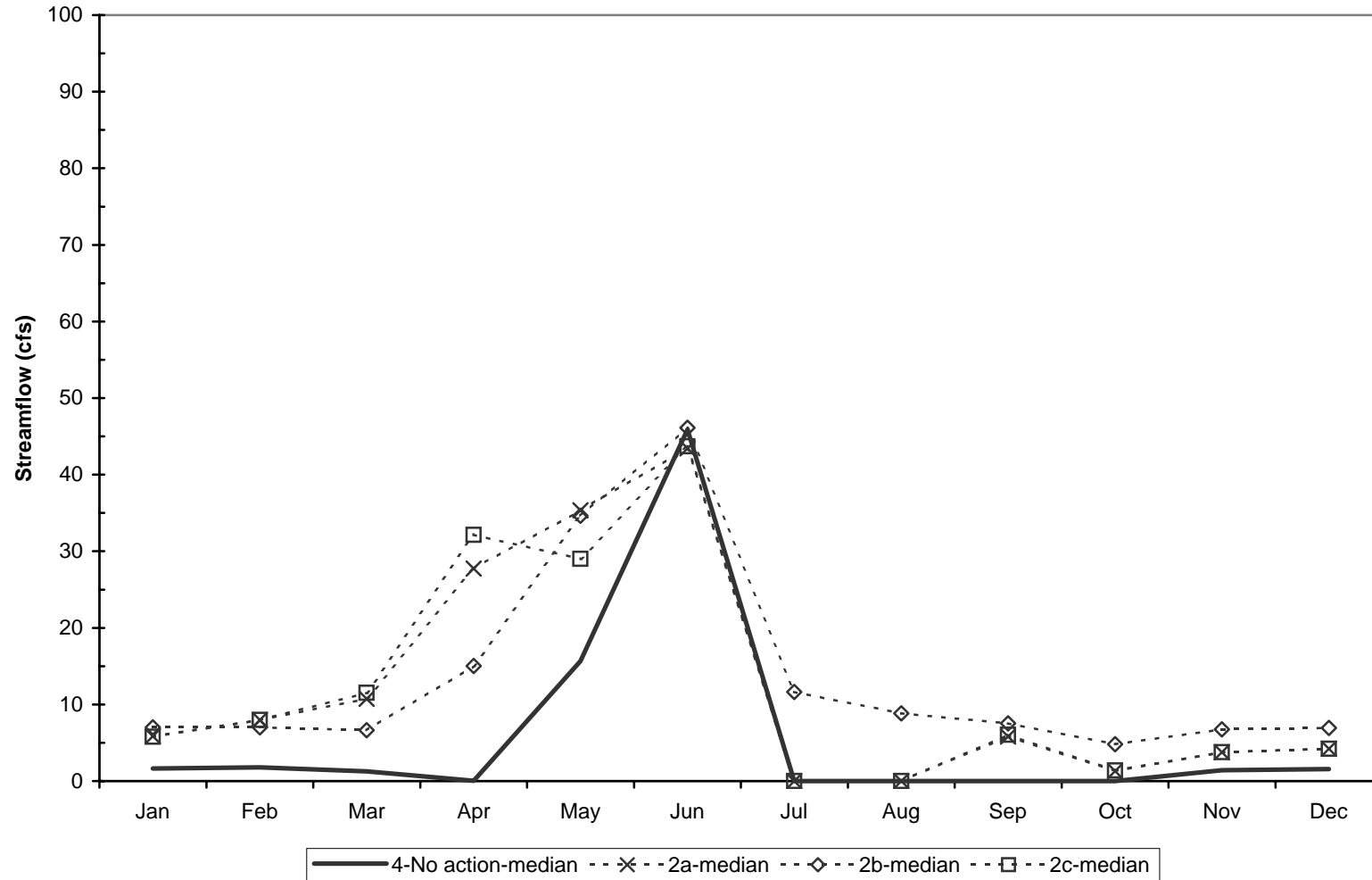
Simulated Median Streamflow, 1904-2002 - Below Weir Salmon Creek No Action vs Upgrade Shellrock Pumping Plant Alternative
