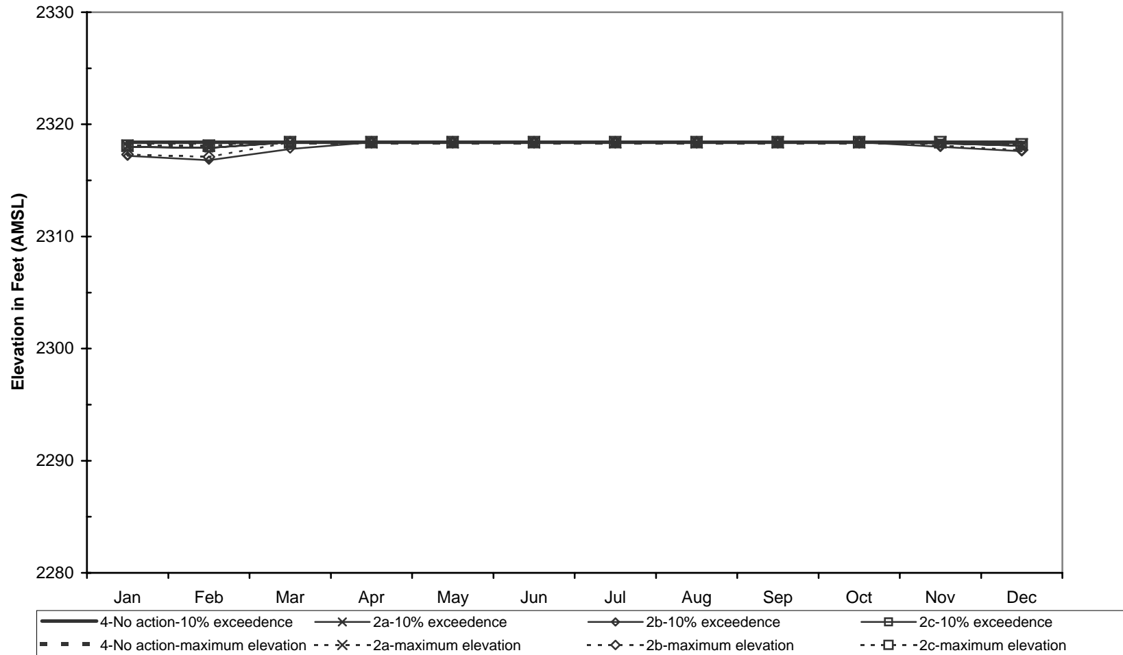
Simulated Maximum Lake Elevation, 1904-2002 - Salmon Lake No Action vs Upgrade Shellrock Pumping Plant Alternative
