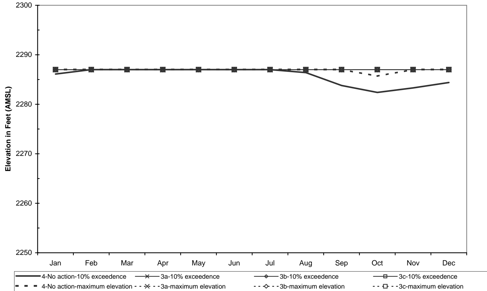
Simulated Maximum Lake Elevation, 1904-2002 - Conconully Reservoir No Action vs OID Water Right Purchase Alternative
