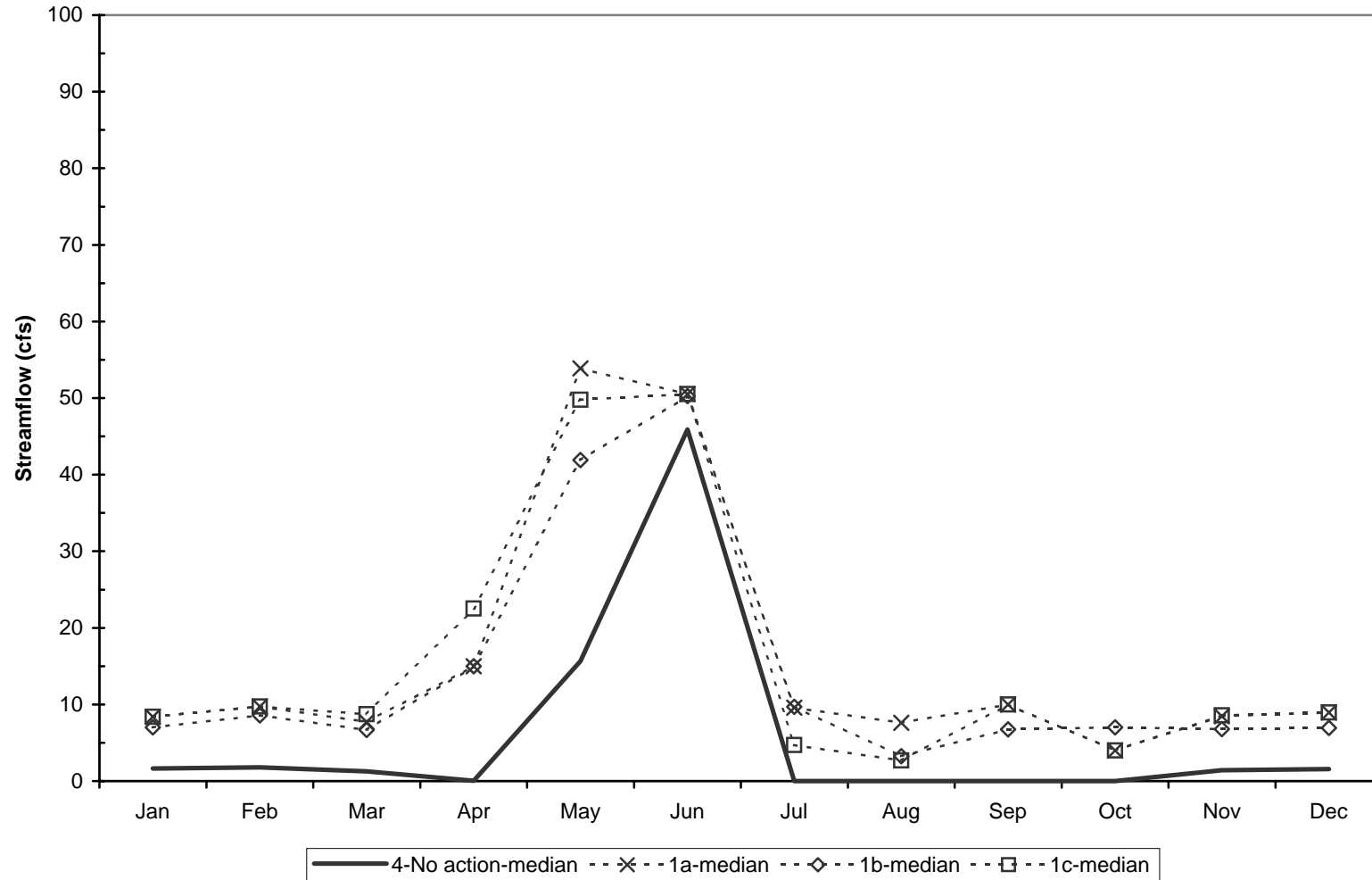
Simulated Median Streamflow, 1904-2002 - Below Weir Salmon Creek No Action vs Okanogan River Water Exchange Alternative
