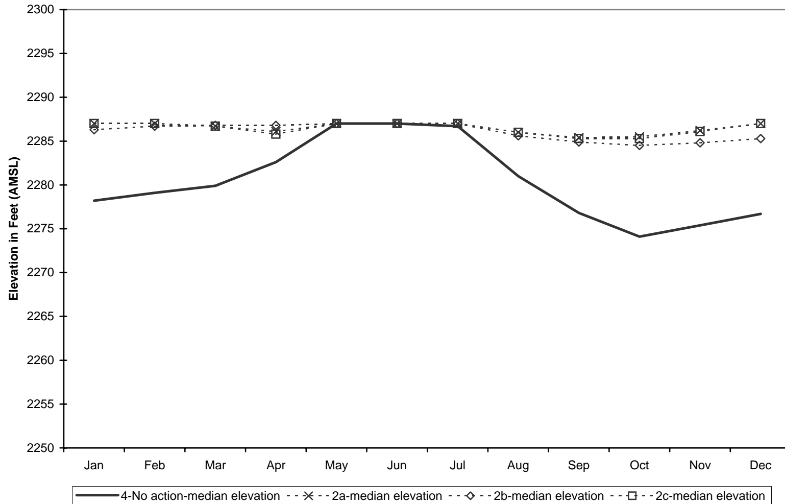
Simulated Median Elevation, 1904-2002 - Conconully Reservoir No Action vs Upgrade Shellrock Pumping Plant Alternative
