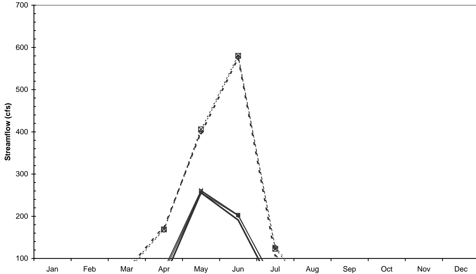
Simulated High-Flow, Low-Frequency Streamflow, 1904-2002 - Below Weir Salmon Creek No Action vs OID Water Right Purchase Alternative
