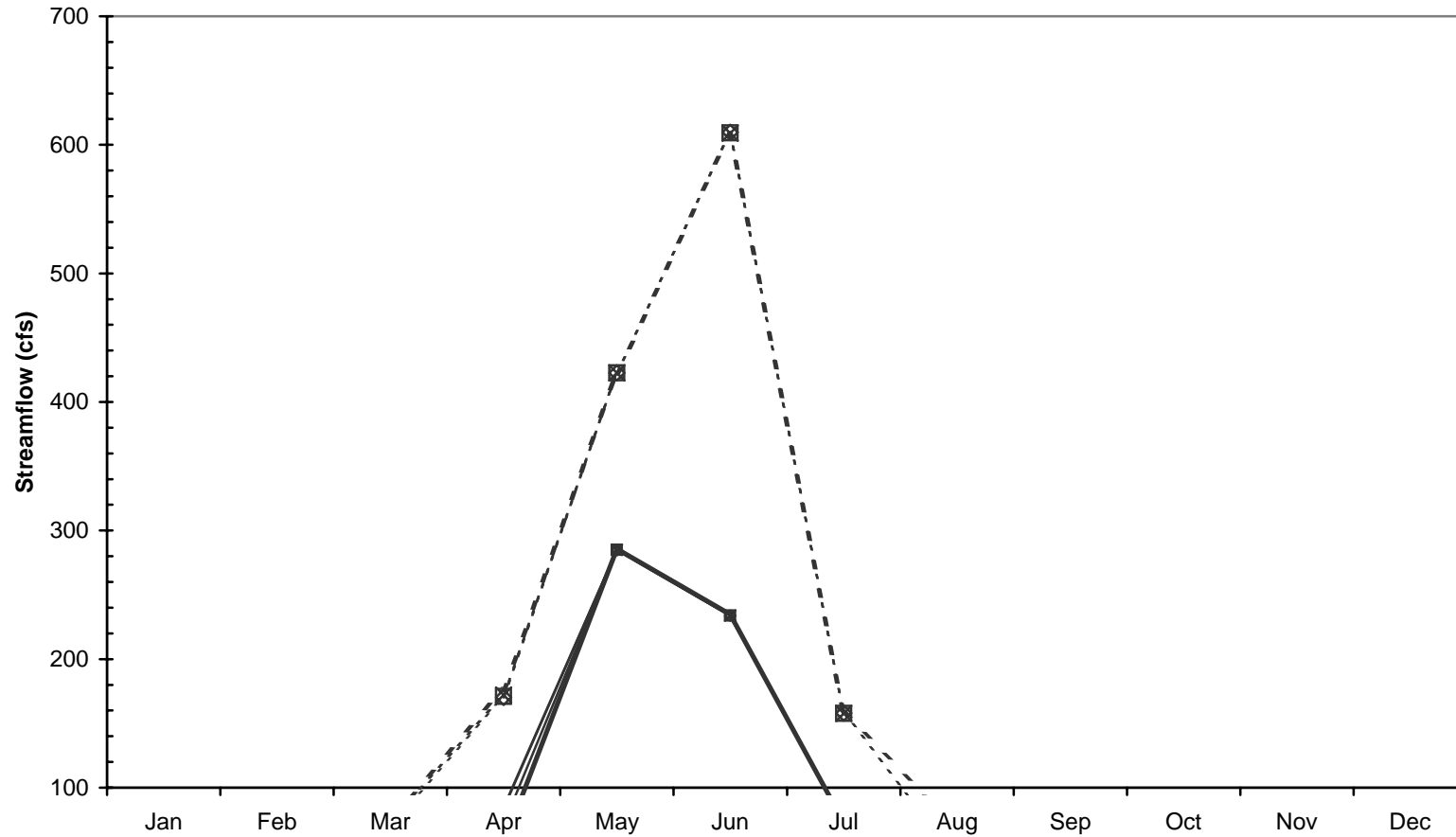
Simulated High-Flow, Low-Frequency Streamflow, 1904-2002 - Middle Reach Salmon Creek No Action vs Okanogan River Water Exchange Alternative
