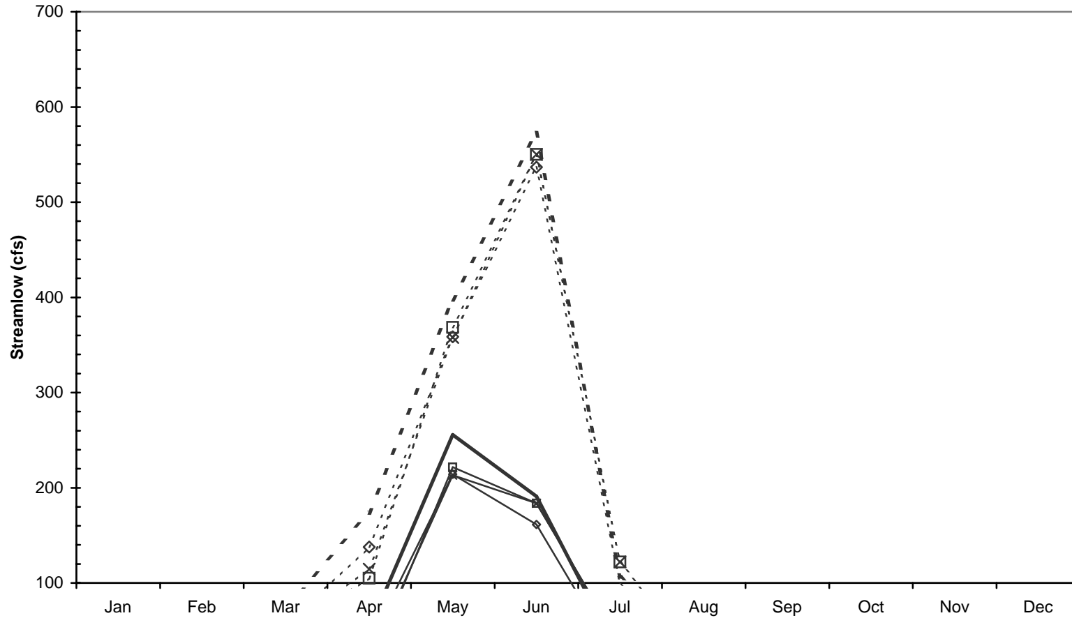
Simulated High-Flow, Low-Frequency Streamflow, 1904-2002 - Conconully Reservoir Spill No Action vs OID Water Right Purchase Alternative
