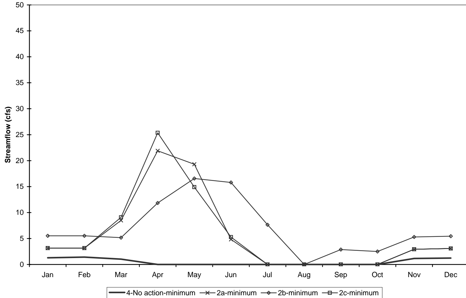
Simulated Minimum Streamflow, 1904-2002 - Lower Reach Salmon Creek No Action vs Upgrade Shellrock Pumping Plant Alternative
