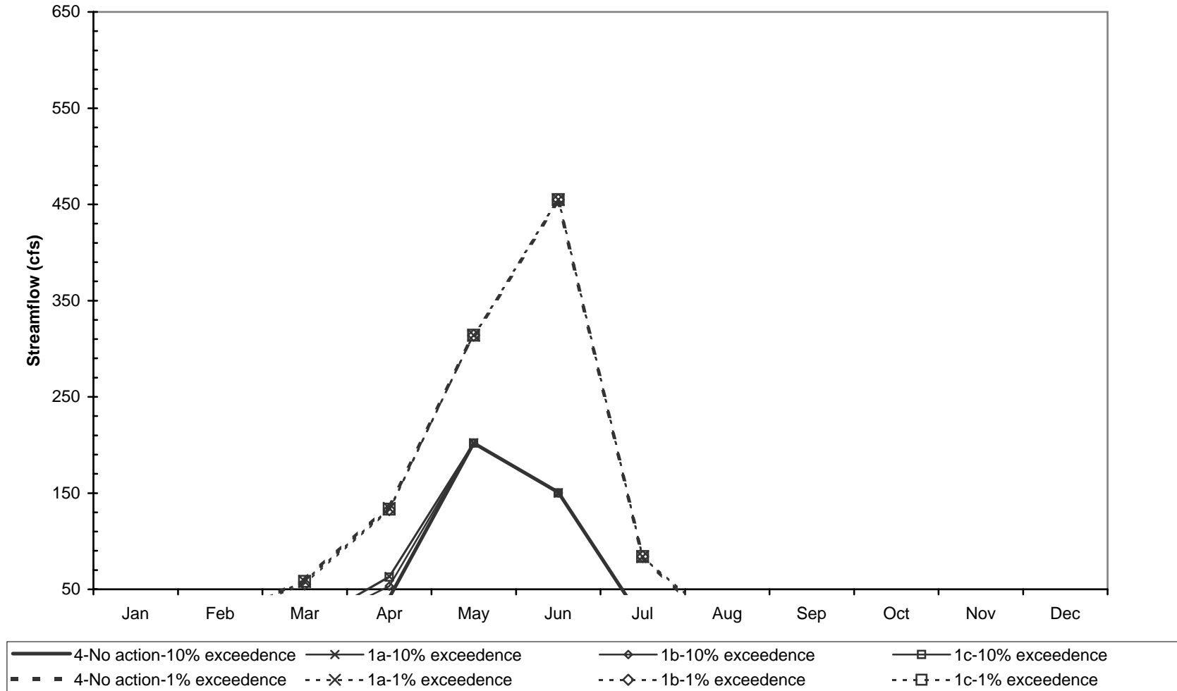
Simulated High-Flow, Low-Frequency Streamflow, 1904-2002 - Lower Reach Salmon Creek No Action vs Okanogan River Water Exchange Alternative
