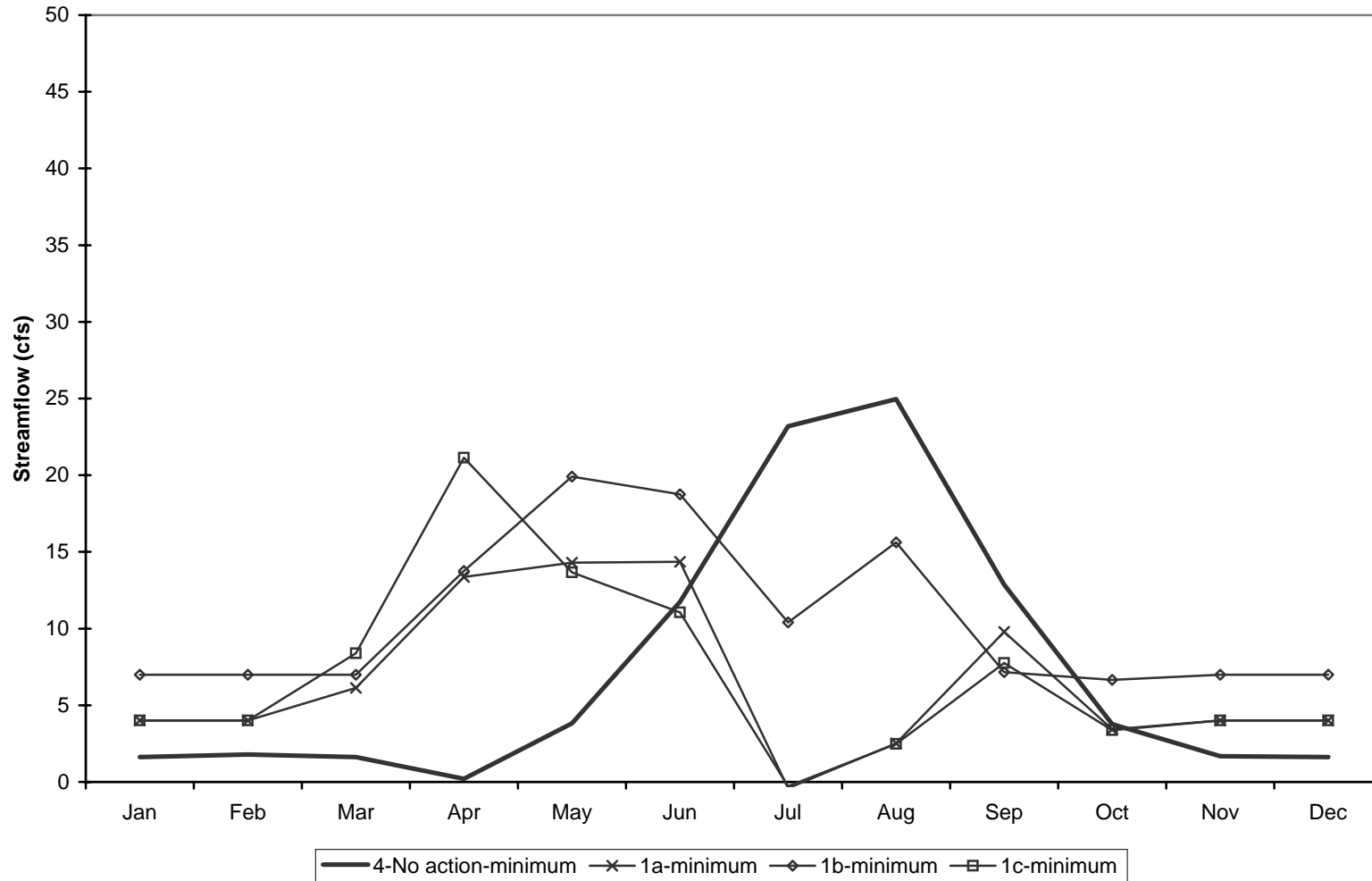
Simulated Minimum Streamflow, 1904-2002 - Middle Reach Salmon Creek No Action vs Okanogan River Water Exchange Alternative
