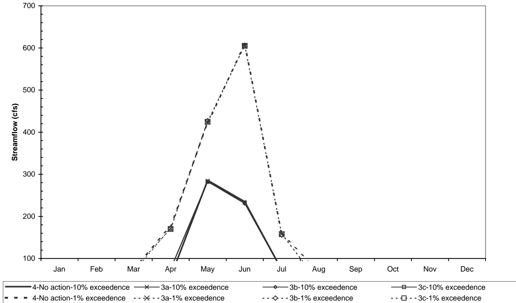
Simulated High-Flow, Low-Frequency Streamflow, 1904-2002 - Middle Reach Salmon Creek No Action vs OID Water Right Purchase Alternative
