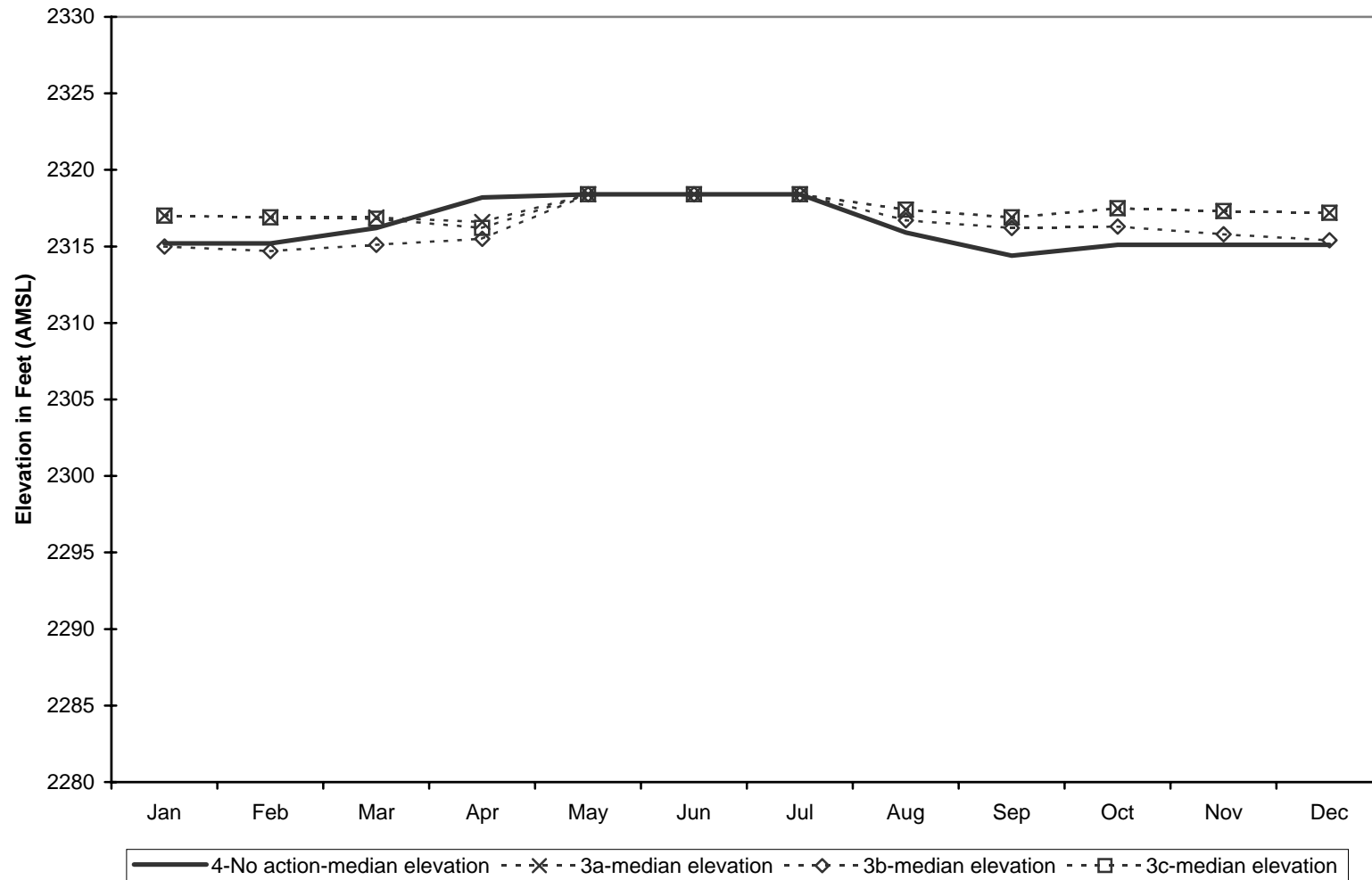
Simulated Median Lake Elevation, 1904-2002 - Salmon Lake No Action vs OID Water Right Purchase Alternative
