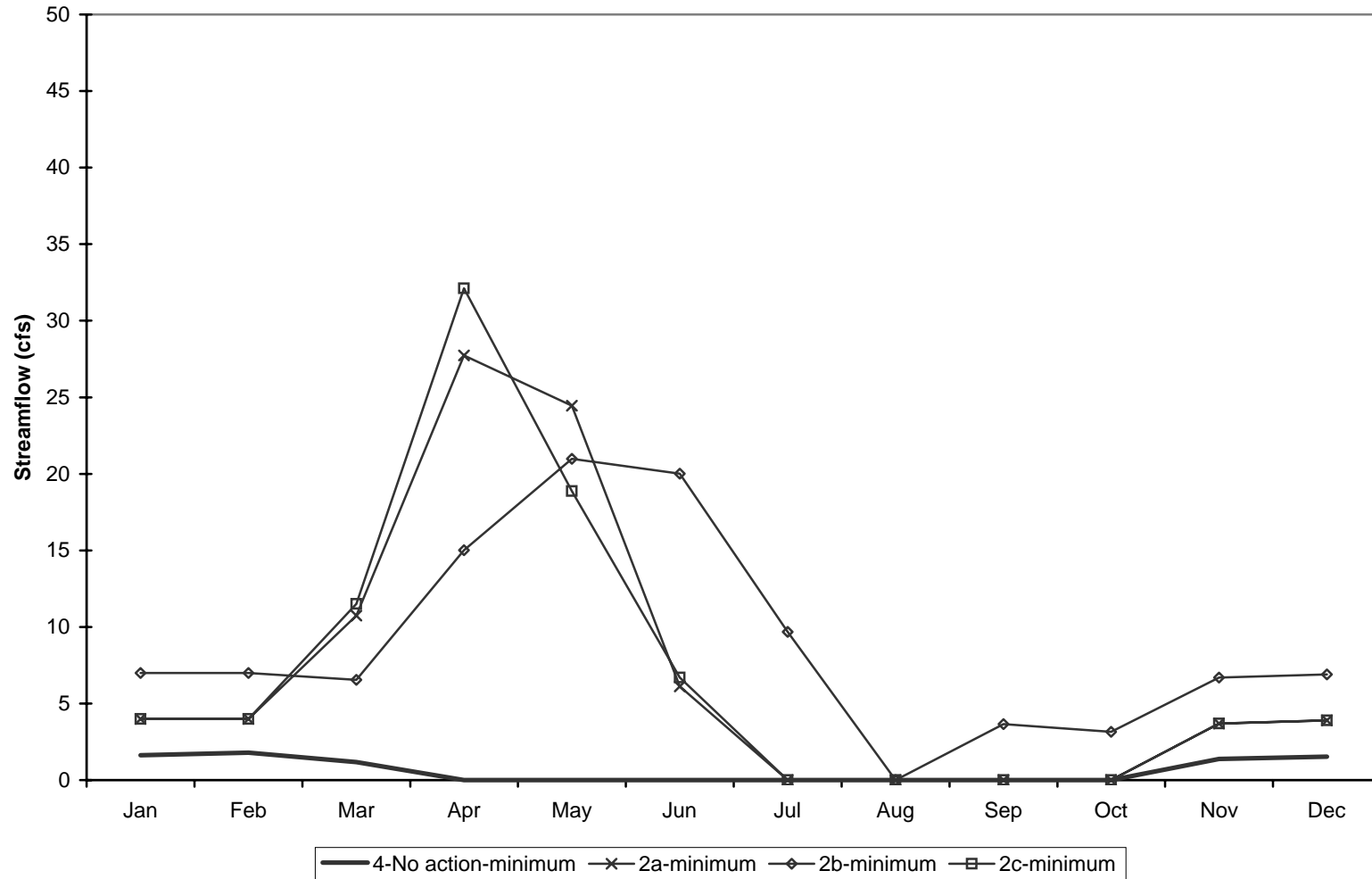
Simulated Minimum Streamflow, 1904-2002 - Below Weir Salmon Creek No Action vs Upgrade Shellrock Pumping Plant Alternative
