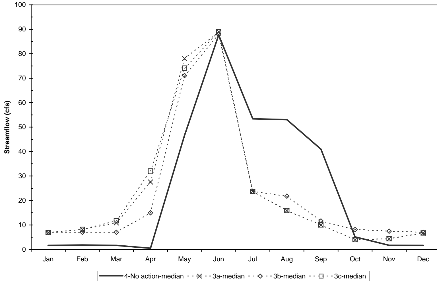
Simulated Median Streamflow, 1904-2002 - Middle Reach Salmon Creek No Action vs. Old Water Right Purchase Alternative
