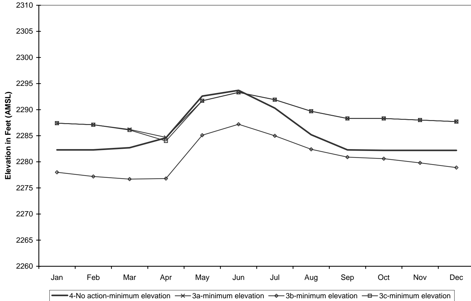
Simulated Minimum Lake Elevation, 1904-2002 - Salmon Lake No Action vs OID Water Right Purchase Alternative
