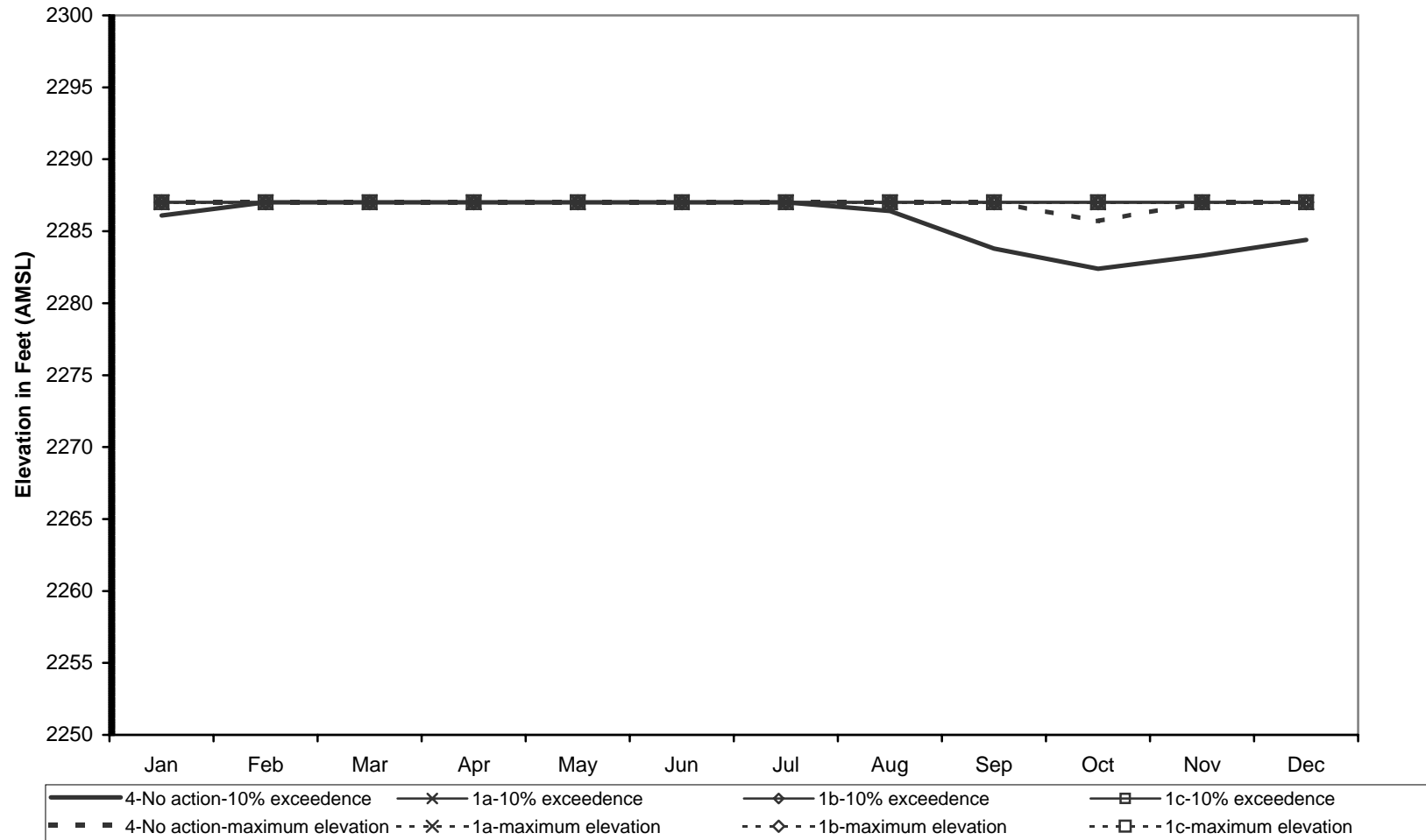
Simulated Maximum Lake Elevation, 1904-2002 - Conconully Reservoir No Action vs Okanogan River Water Exchange Alternative
