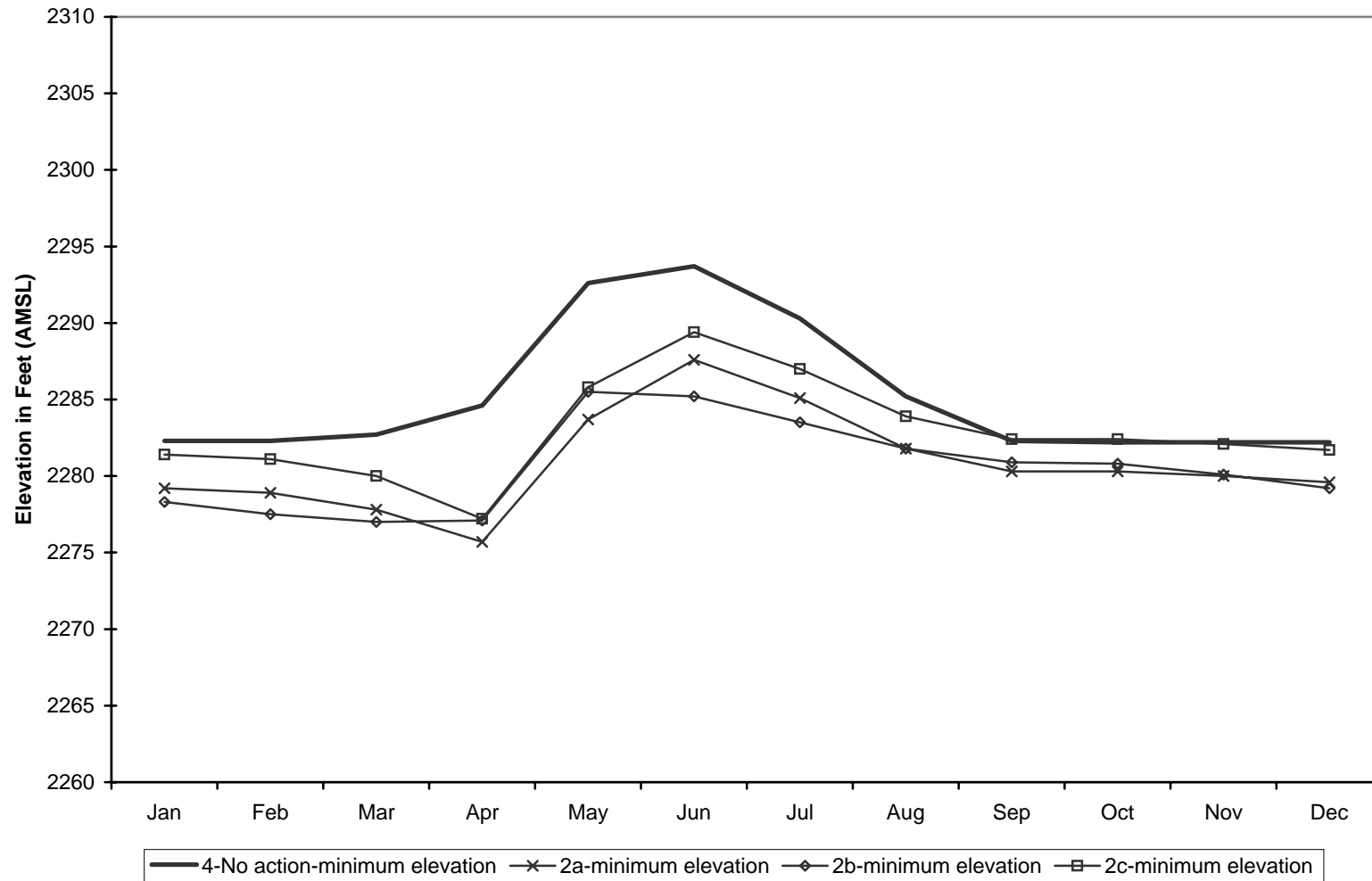
Simulated Minimum Lake Elevation, 1904-2002 - Salmon Lake No Action vs Upgrade Shellrock Pumping Plant Alternative
