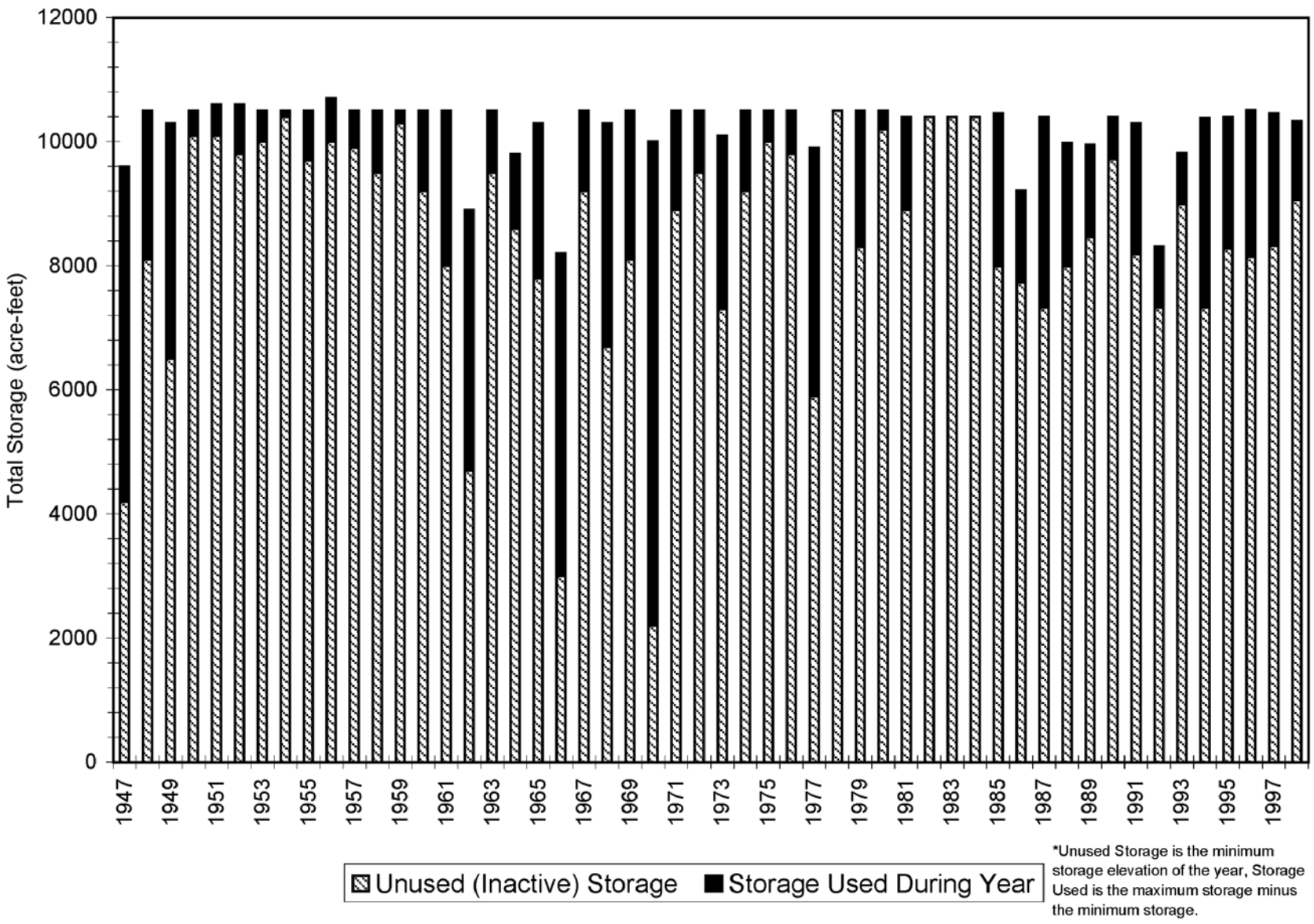
Figure 3-12. Measured Storage Utilization in Salmon Lake Reservoir.
