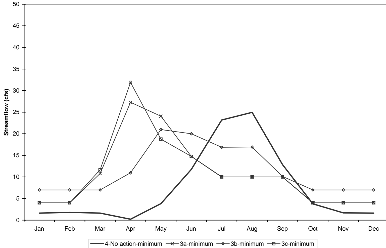
Simulated Minimum Streamflow, 1904-2002 - Middle Reach Salmon Creek No Action vs Old Water Right Purchase Alternative
