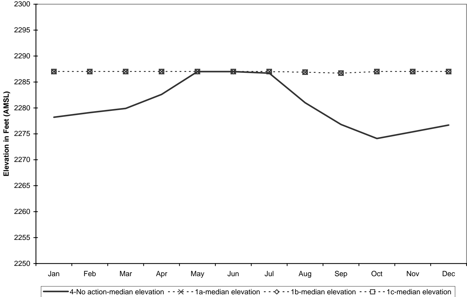
Simulated Median Lake Elevation, 1904-2002 - Conconully Reservoir No Action vs Okanogan River Water Exchange Alternative
