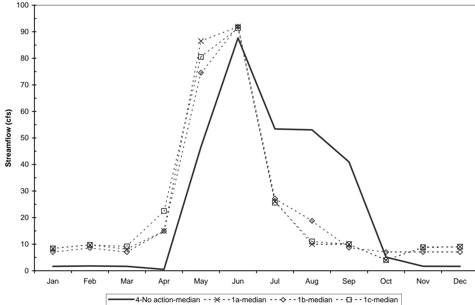
Simulated Median Streamflow, 1904-2002 - Middle Reach Salmon Creek No Action vs Okanogan River Water Exchange Alternative
