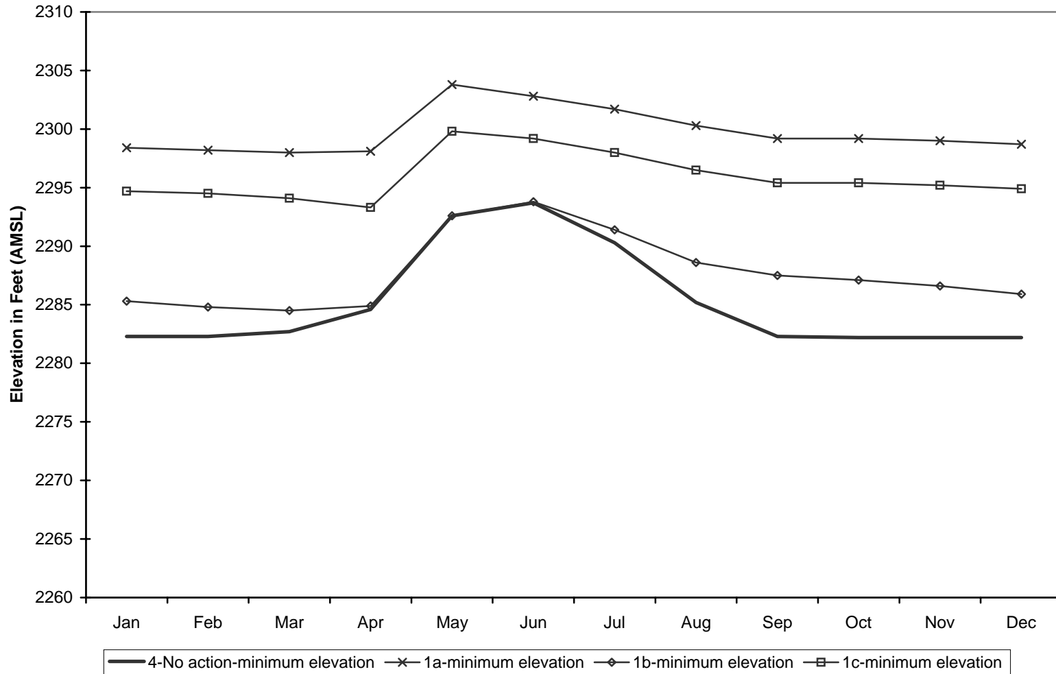
Simulated Minimum Lake Elevation, 1904-2002 - Salmon Lake No Action vs Okanogan River Water Exchange
