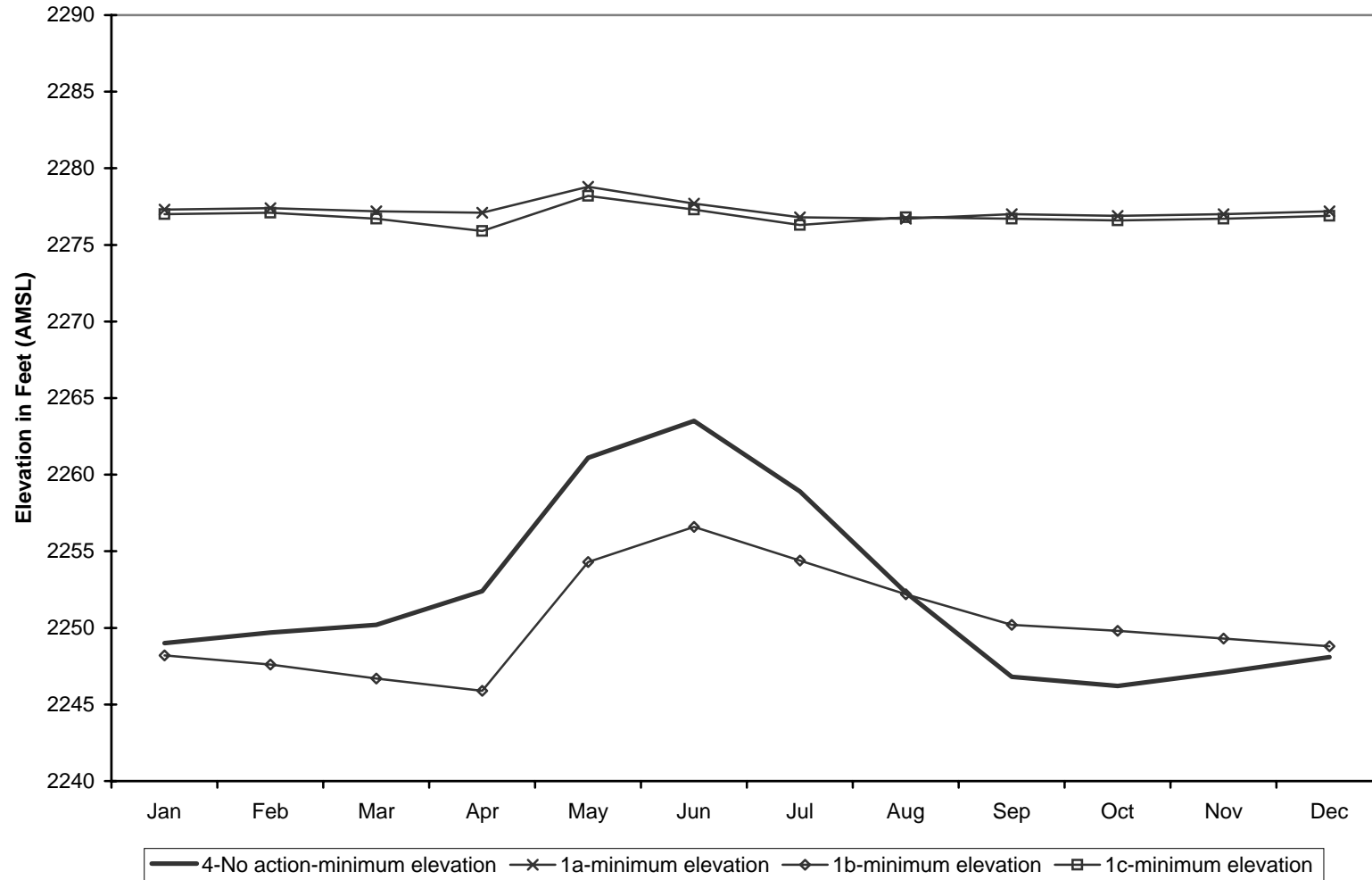
Simulated Minimum Lake Elevation, 1904-2002 - Conconully Reservoir No Action vs Okanogan River Water Exchange Alternative
