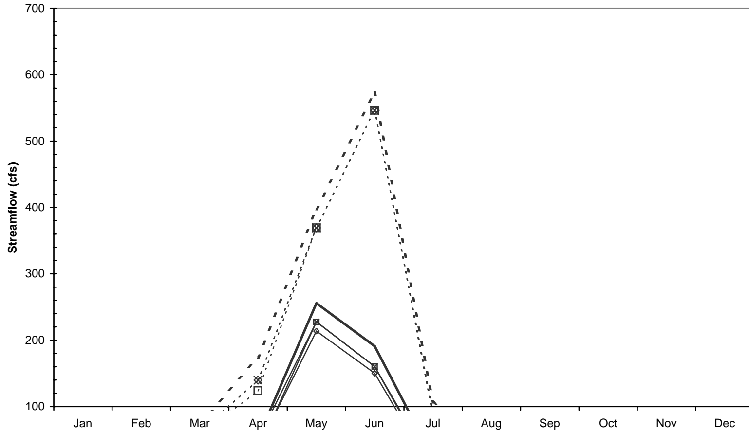
Simulated High-Flow, Low-Frequency Streamflow, 1904-2002 - Conconully Reservoir Spill No Action vs Okanogan River Water Exchange Alternative
