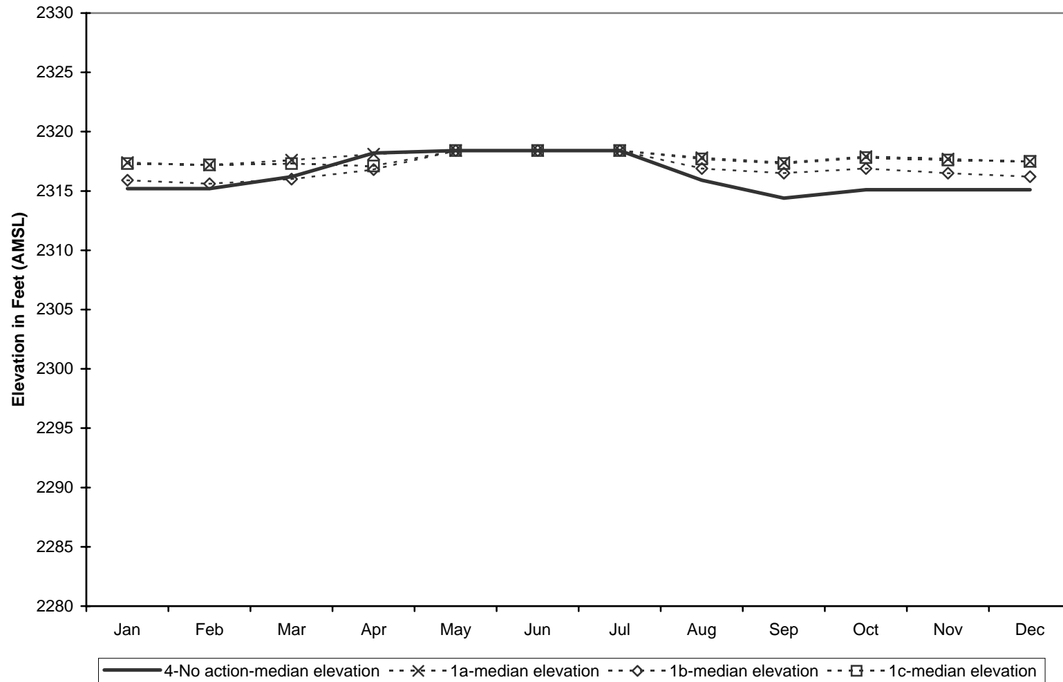
Simulated Median Lake Elevation, 1904-2002 - Salmon Lake No Action vs Okanogan River Water Exchange Alternative
