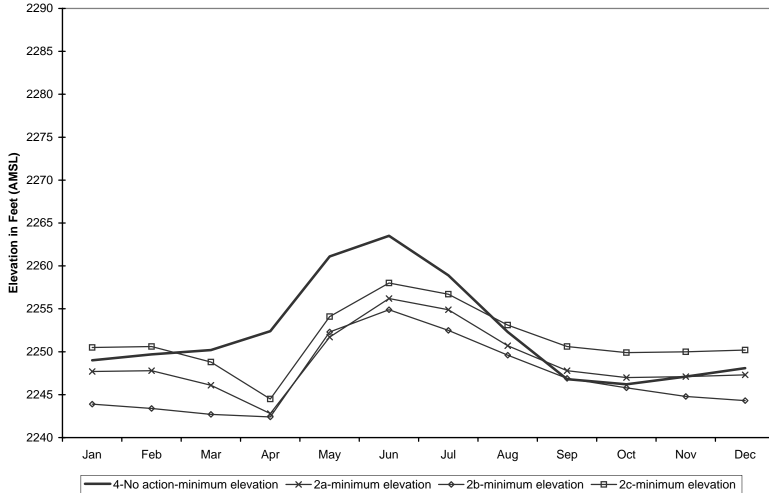
Simulated Minimum Lake Elevation, 1904-2002 - Conconully Reservoir No Action vs Upgrade Shellrock Pumping Plant Alternative
