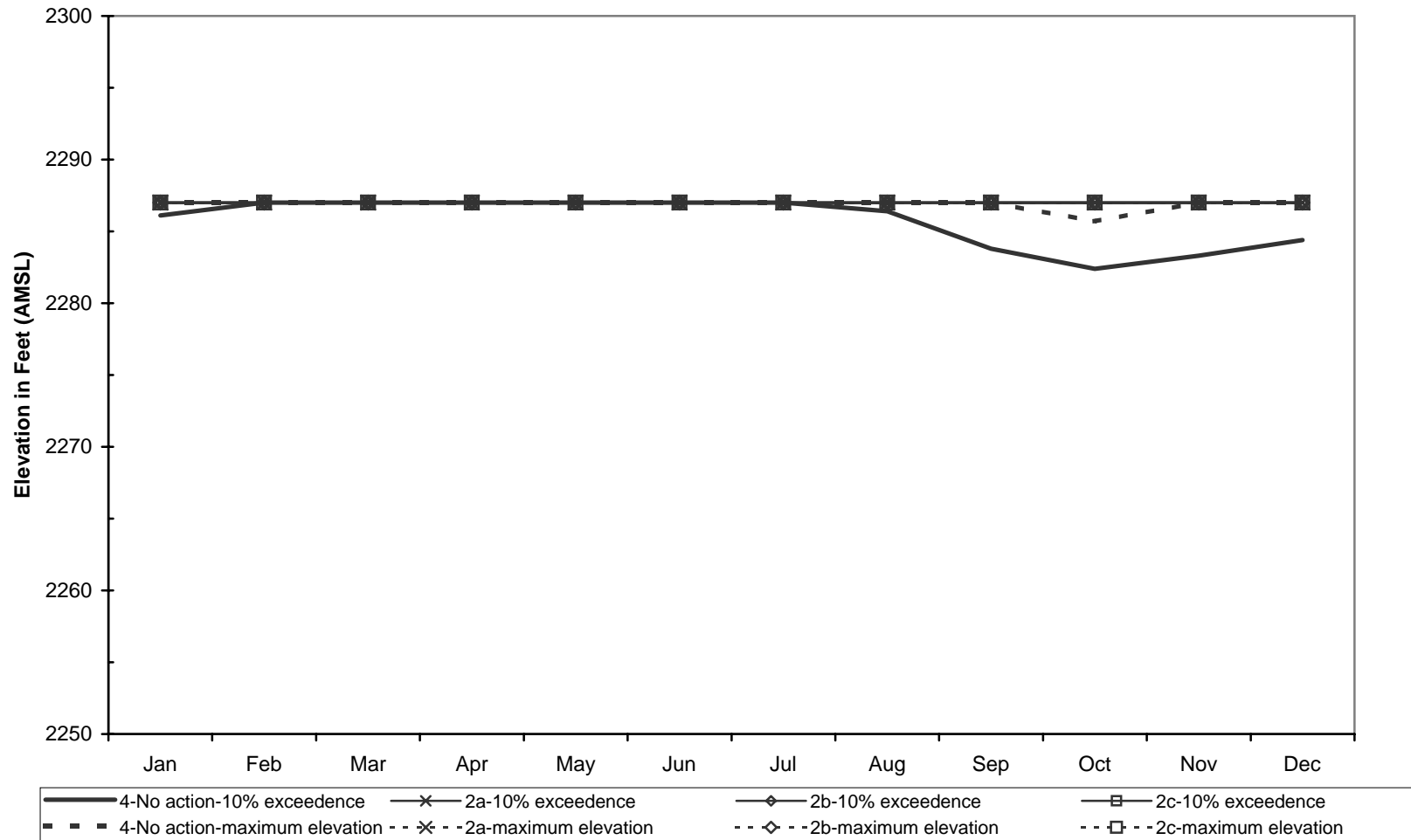
Simulated Maximum Lake Elevation, 1904-2002 - Conconully Reservoir No Action vs Upgrade Shellrock Pumping Plant Alternative
