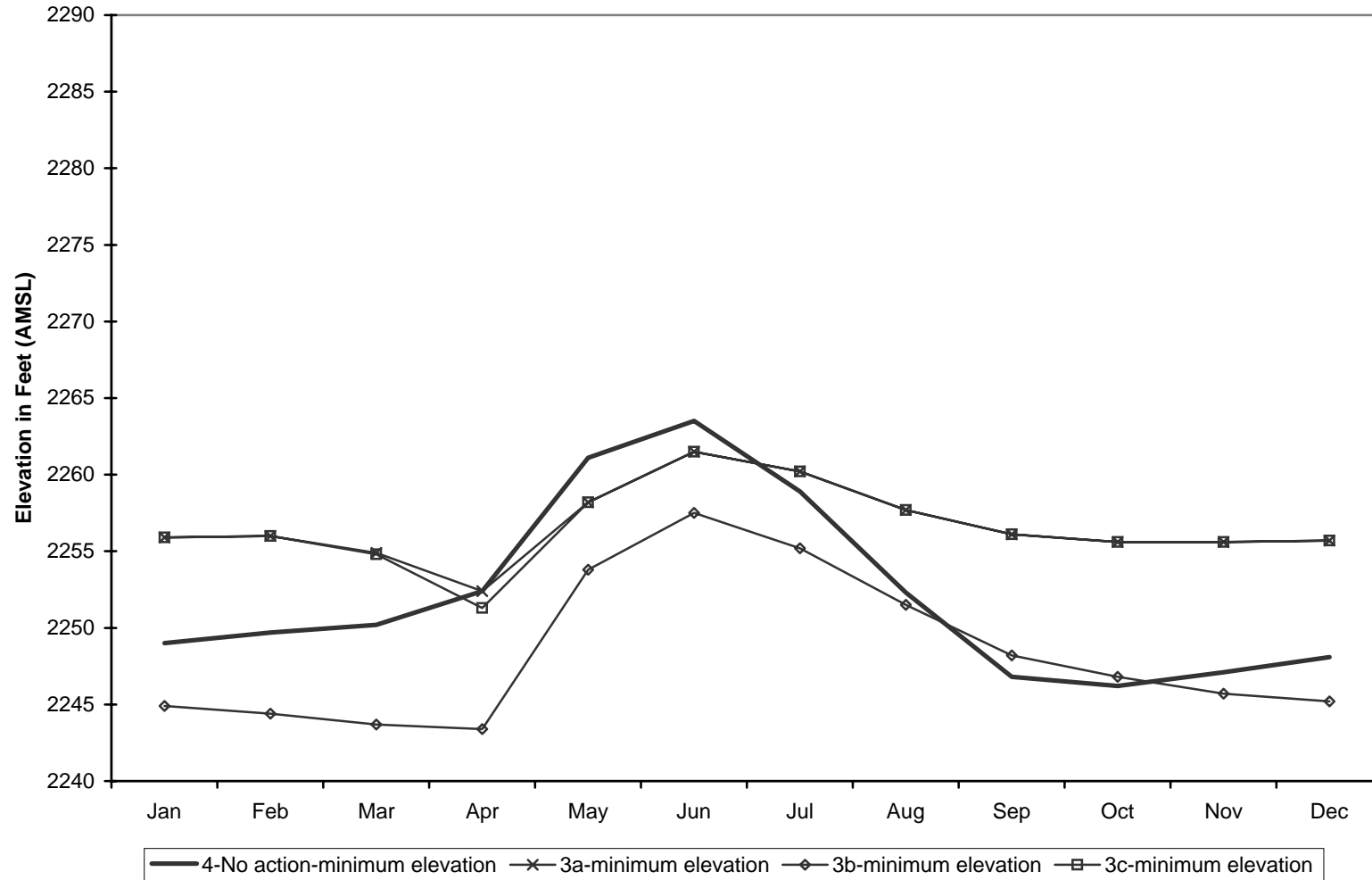
Simulated Minimum Lake Elevation, 1904-2002 - Conconully Reservoir No Action vs OID Water Right Purchase Alternative
