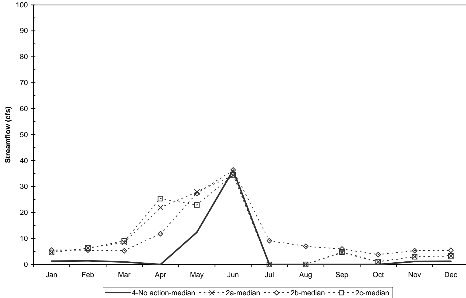
Simulated Median Streamflow, 1904-2002 - Lower Reach Salmon Creek No Action vs Upgrade Shellrock Pumping Plant Alternative
