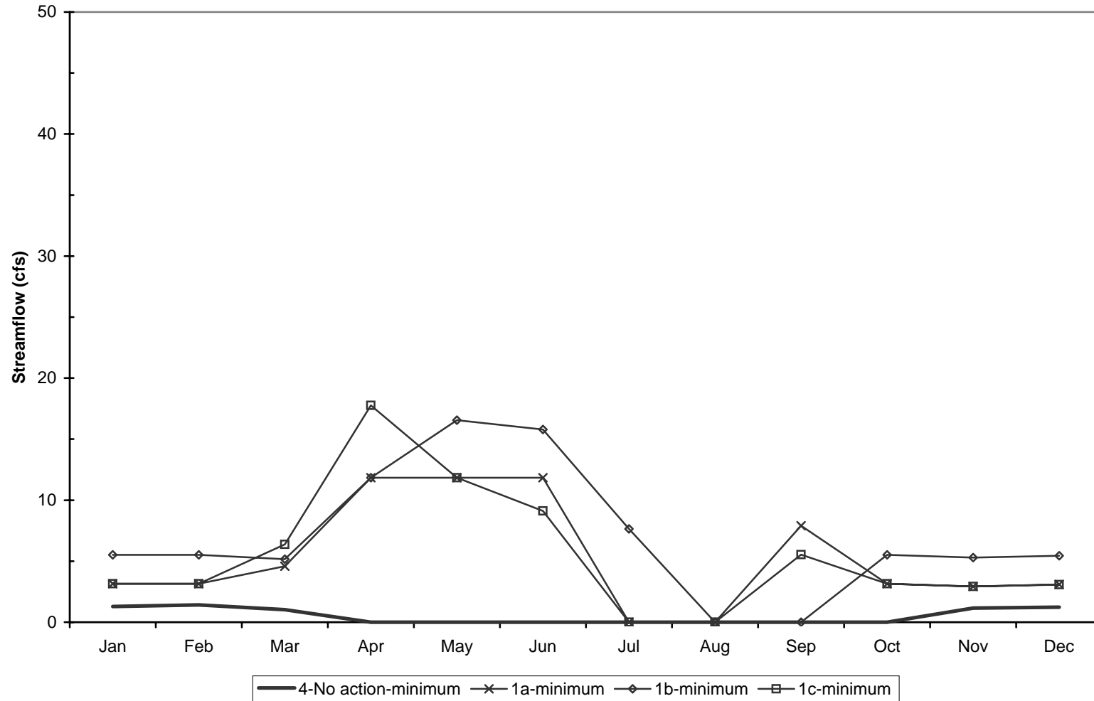
Simulated Minimum Streamflow, 1904-2002 - Lower Reach Salmon Creek No Action vs Okanogan River Water Exchange Alternative
