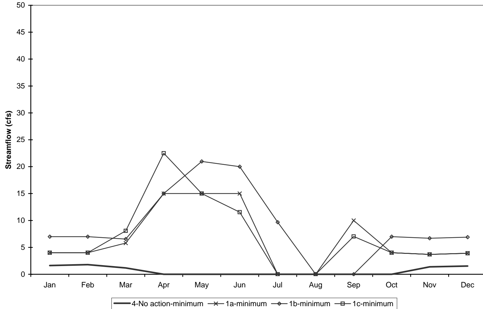
Simulated Minimum Streamflow, 1904-2002 - Below Weir Salmon Creek No Action vs Okanogan River Water Exchange Alternative
