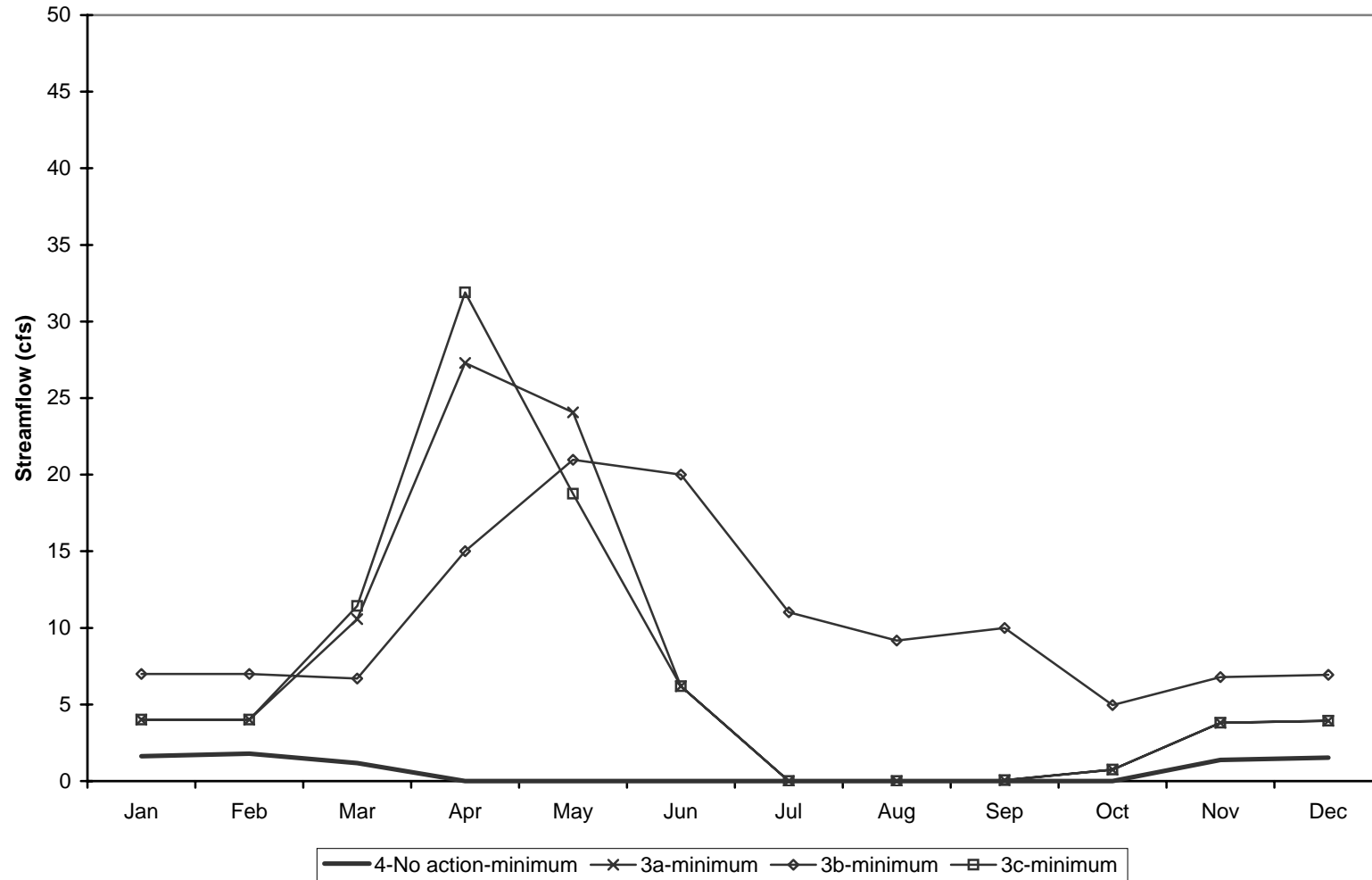
Simulated Minimum Streamflow, 1904-2002 - Below Weir Salmon Creek No Action vs OID Water Right Purchase Alternative
