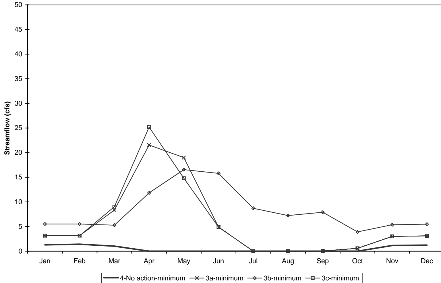
Simulated Minimum Streamflow, 1904-2002 - Lower Reach Salmon Creek No Action vs Old Water Rights Purchase Alternative
