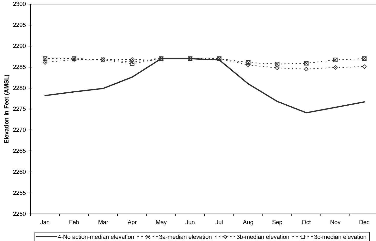
Simulated Median Lake Elevation, 1904-2002 - Conconully Reservoir No Action vs OID Water Right Purchase Alternative
