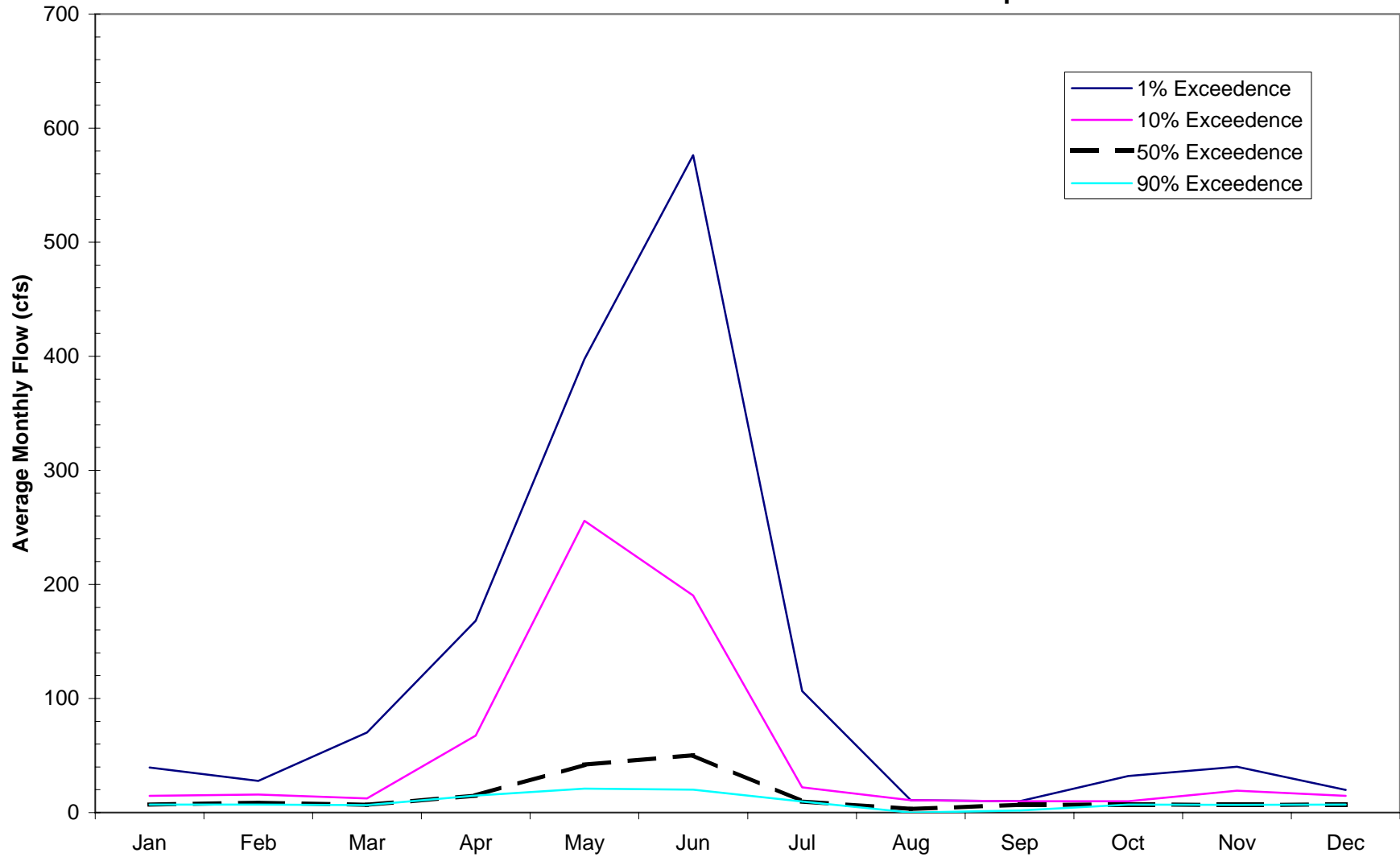
Alternative 1b -- Channel Rehabilitation, Steelhead and Chinook Flows on Salmon Creek Below Weir Exceedence Graph
