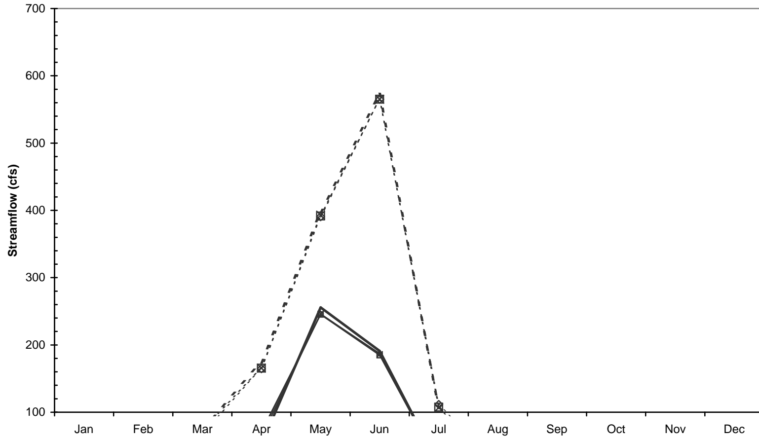
Simulated High-Flow, Low-Frequency Streamflow, 1904-2002 - Below Weir Salmon Creek No Action vs Upgrade Shellrock Pumping Plant Alternative
