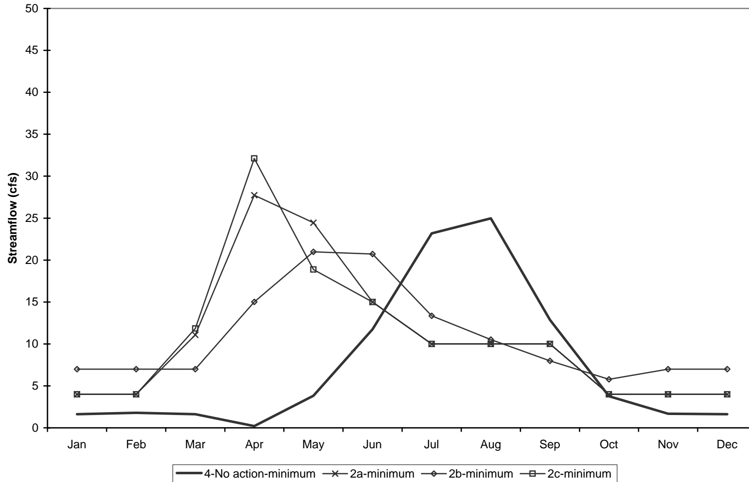
Simulated Minimum Streamflow, 1904-2002 - Middle Reach Salmon Creek No Action vs Upgrade Shellrock Pumping Plant Alternative
