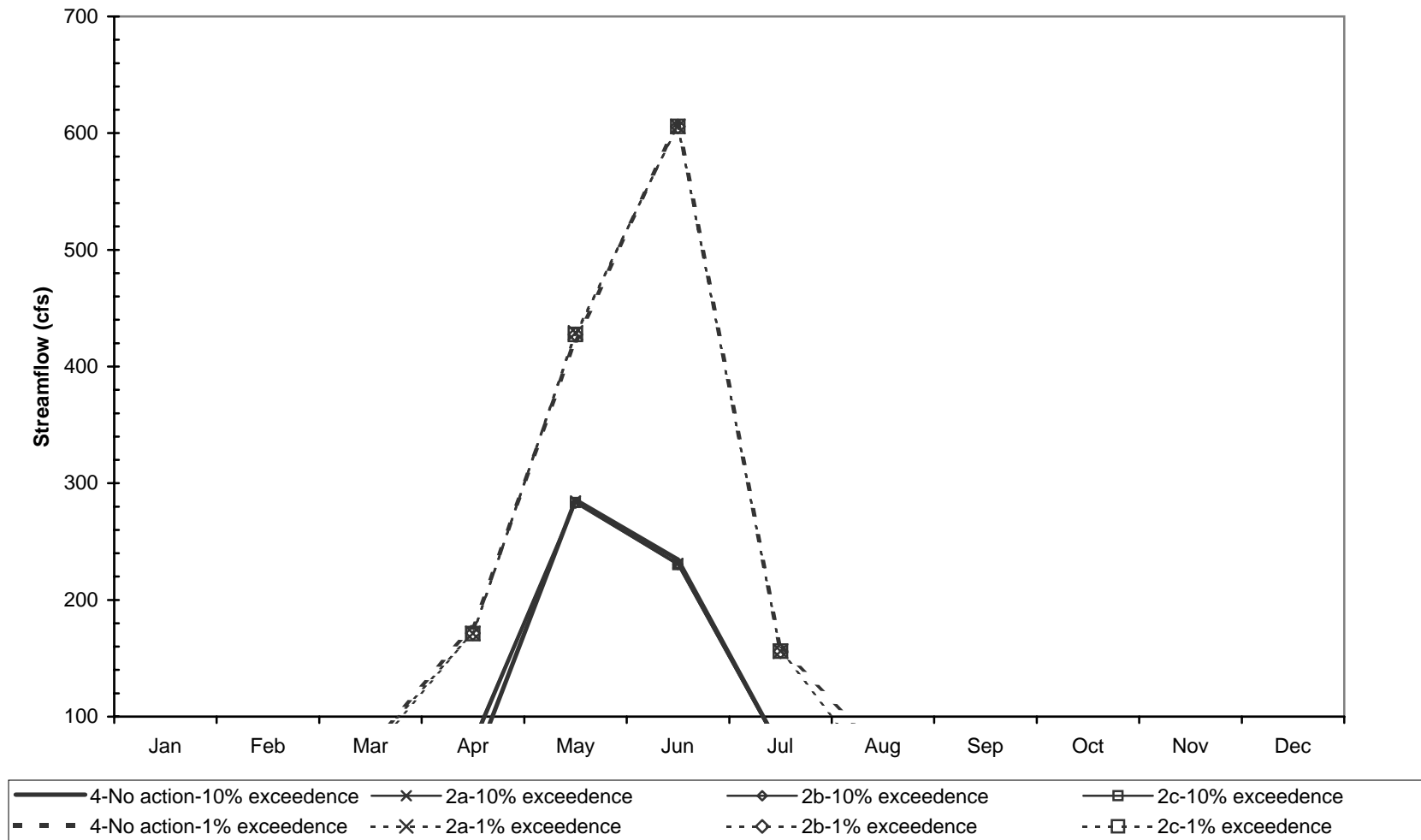
Simulated High-Flow, Low-Frequency Streamflow, 1904-2002 - Middle Reach Salmon Creek No Action vs Upgrade Shellrock Pumping Plant Alternative
