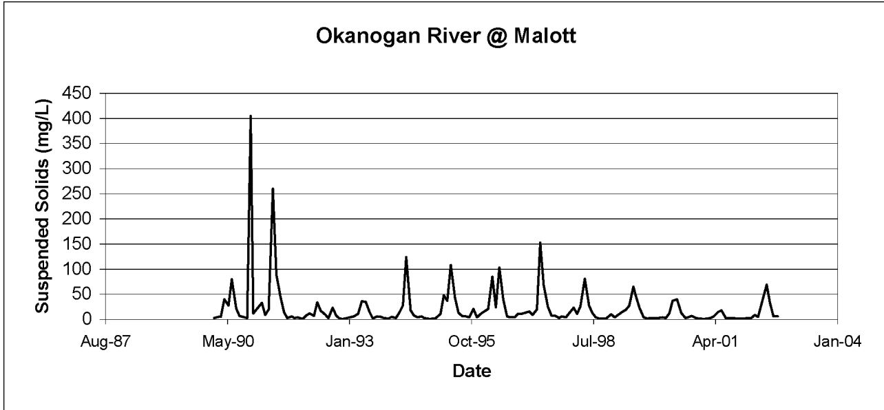
Figure 3-13. Okanogan River Suspended Solid Concentrations at Malott.
