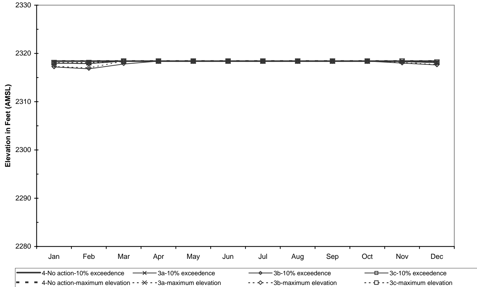
Simulated Maximum Lake Elevation, 1904-2002 - Salmon Lake No Action vs OID Water Right Purchase Alternative
