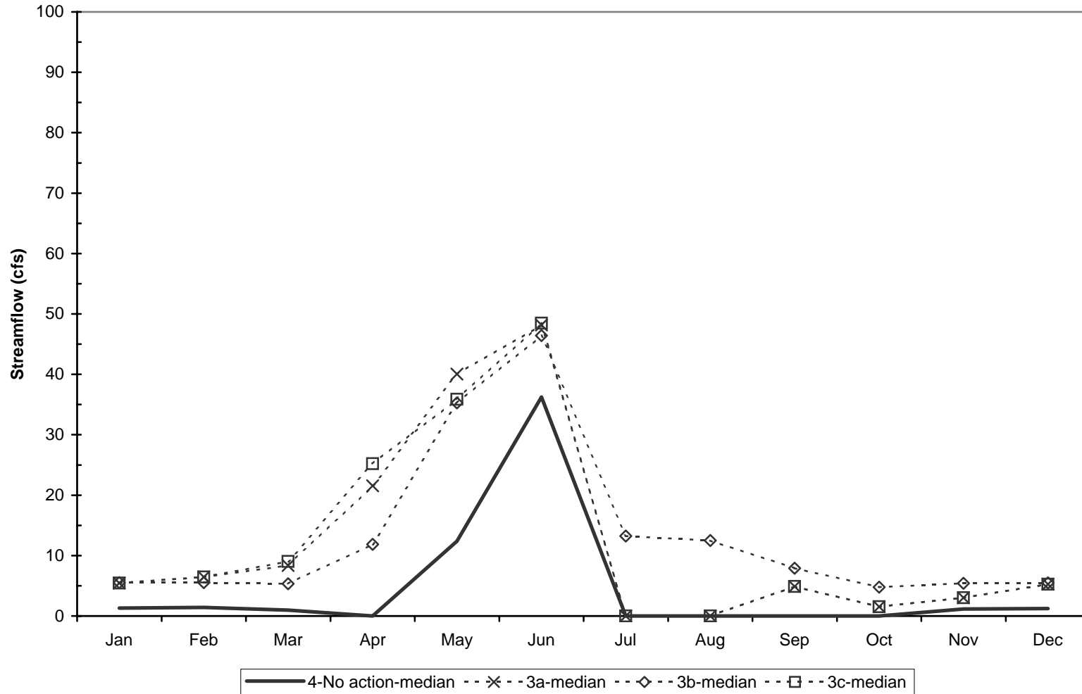
Simulated Median Streamflow, 1904-2002 - Lower Reach Salmon Creek No Action vs OID Water Right Purchase Alternative
