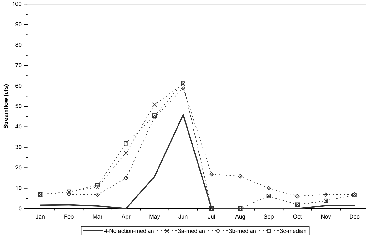
Simulated Median Streamflow, 1904-2002 - Below Weir Salmon Creek No Action vs. Old Water Right Purchase Alternative
