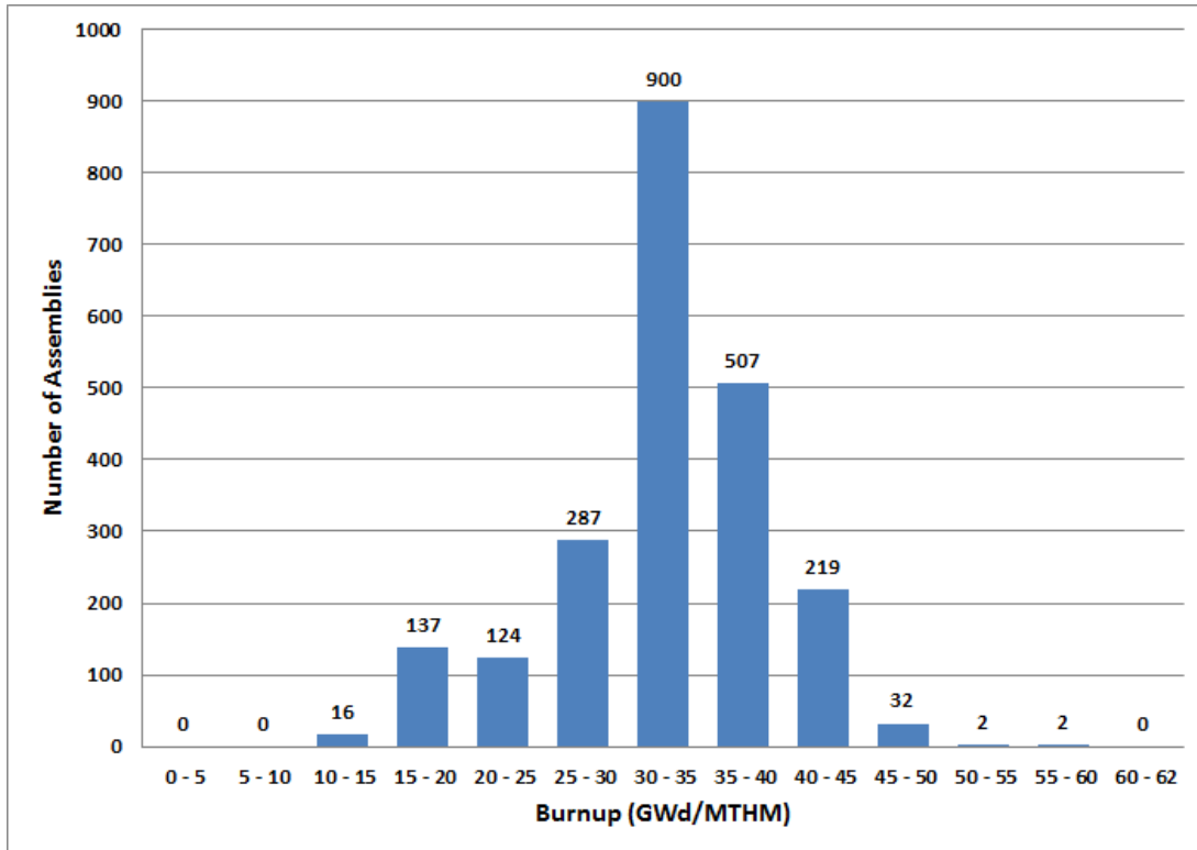
Figure 2-134. Zion Number of Assemblies versus Burnup (EIA 2013)
