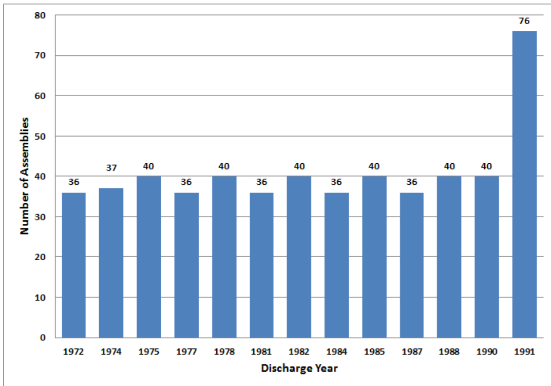
Figure 2-19. Yankee Rowe Number of Assemblies versus Discharge Year (EIA 2013)
