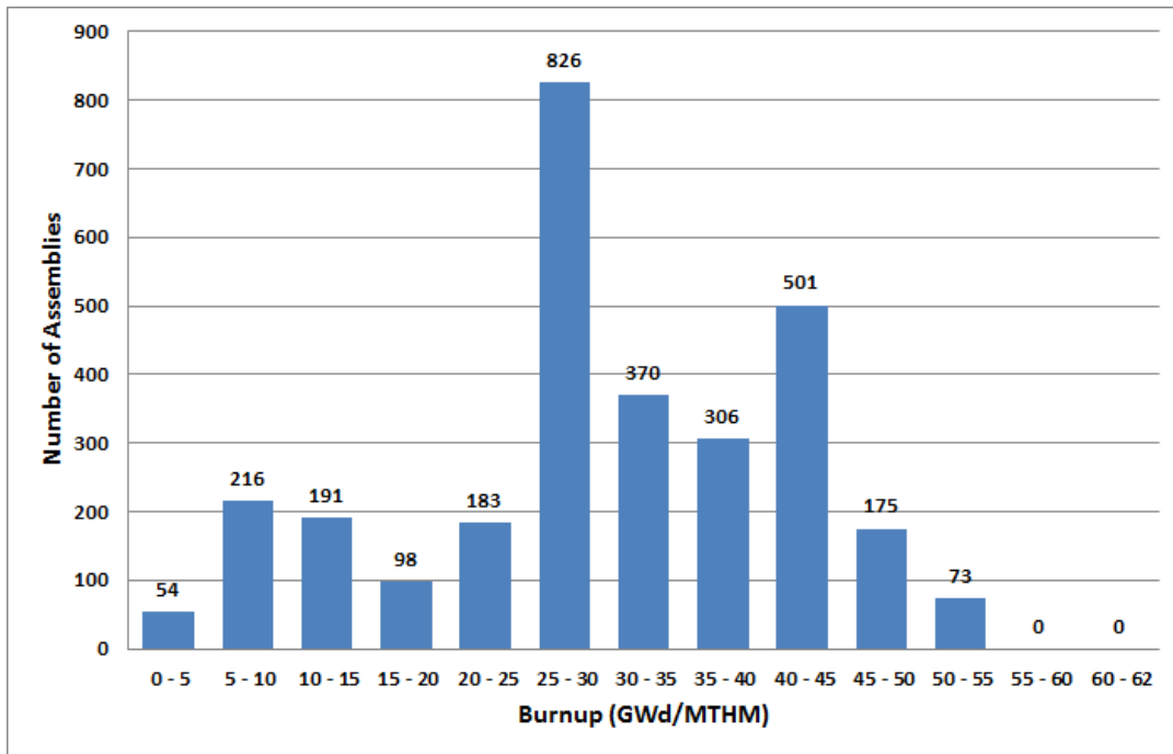
Figure 2-300. Vermont Yankee Number of Uncanistered Assemblies versus Burnup
