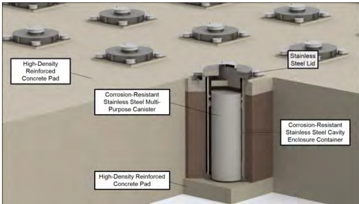
Figure 2-258. Cutaway View of the HI-STORM UMAX Dry Storage System
