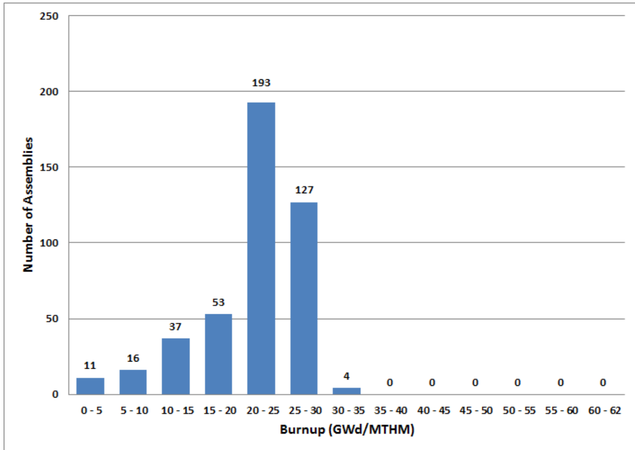
Figure 2-61. Big Rock Point Number of Assemblies versus Burnup (EIA 2013)
