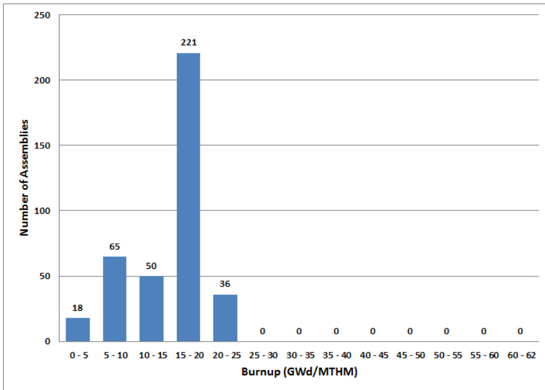
Figure 2-45. Humboldt Bay Number of Assemblies versus Burnup (EIA 2013)
