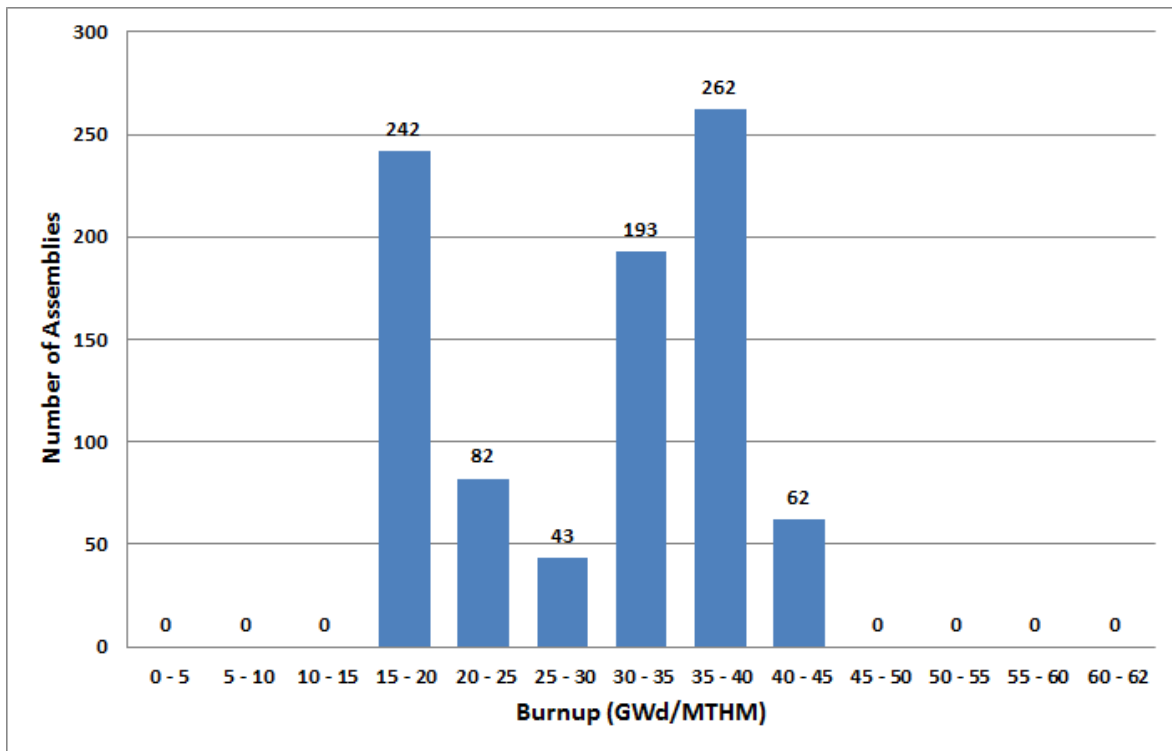
Figure 2-298. Vermont Yankee Number of Canistered Assemblies versus Burnup
