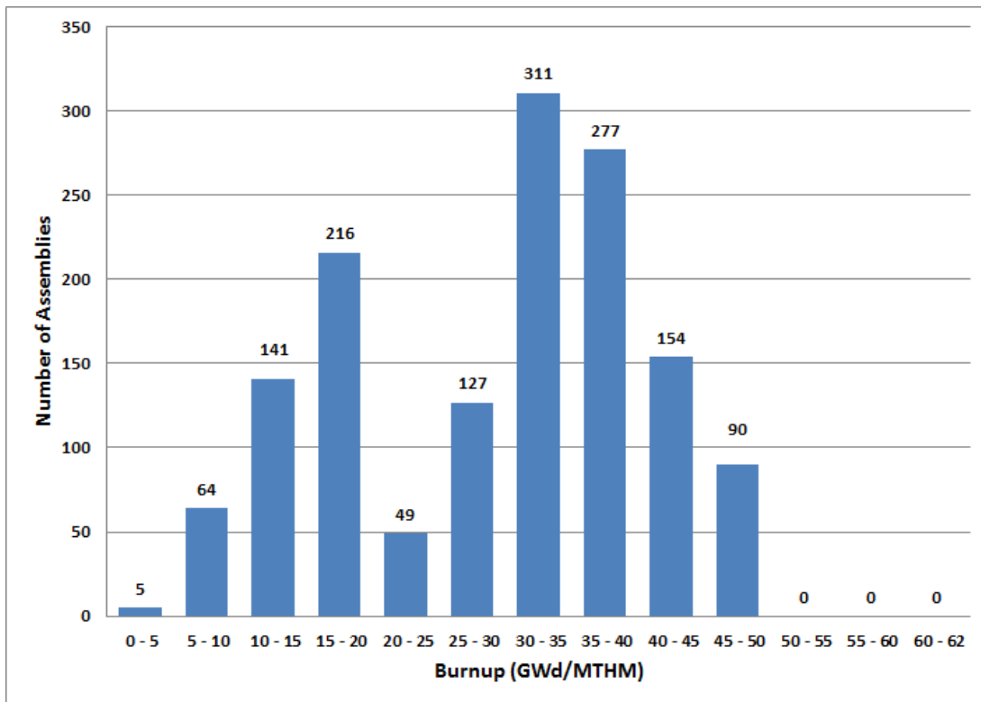
Figure 2-6. Maine Yankee Number of Assemblies versus Burnup (EIA 2013)
