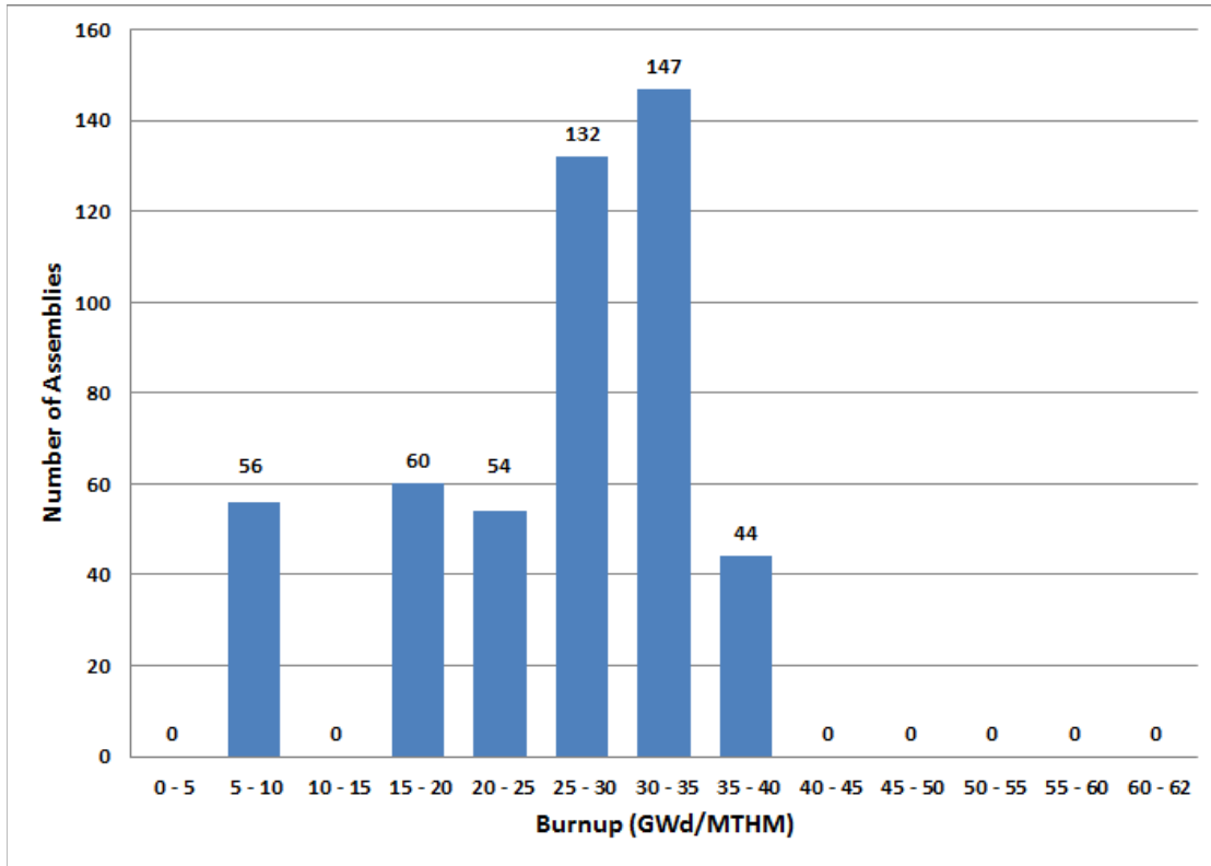
Figure 2-87. Rancho Seco Number of Assemblies versus Burnup (EIA 2013)
