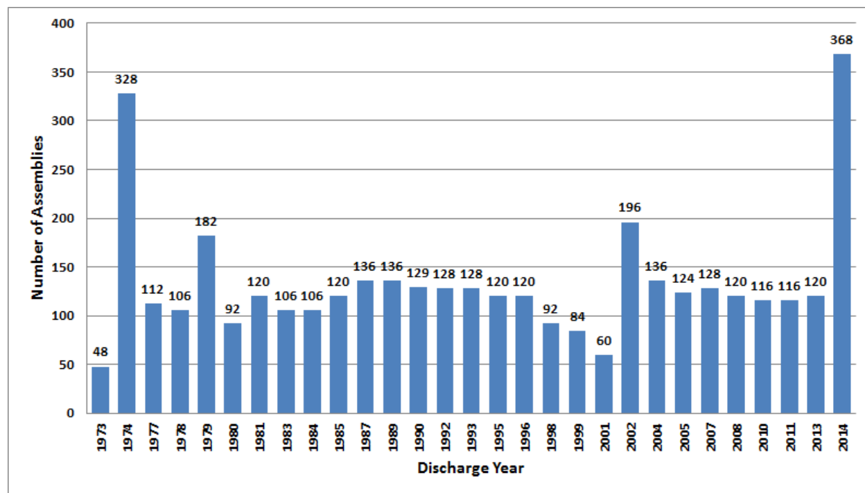
Figure 2-295. Vermont Yankee Number of Assemblies versus Discharge Year
