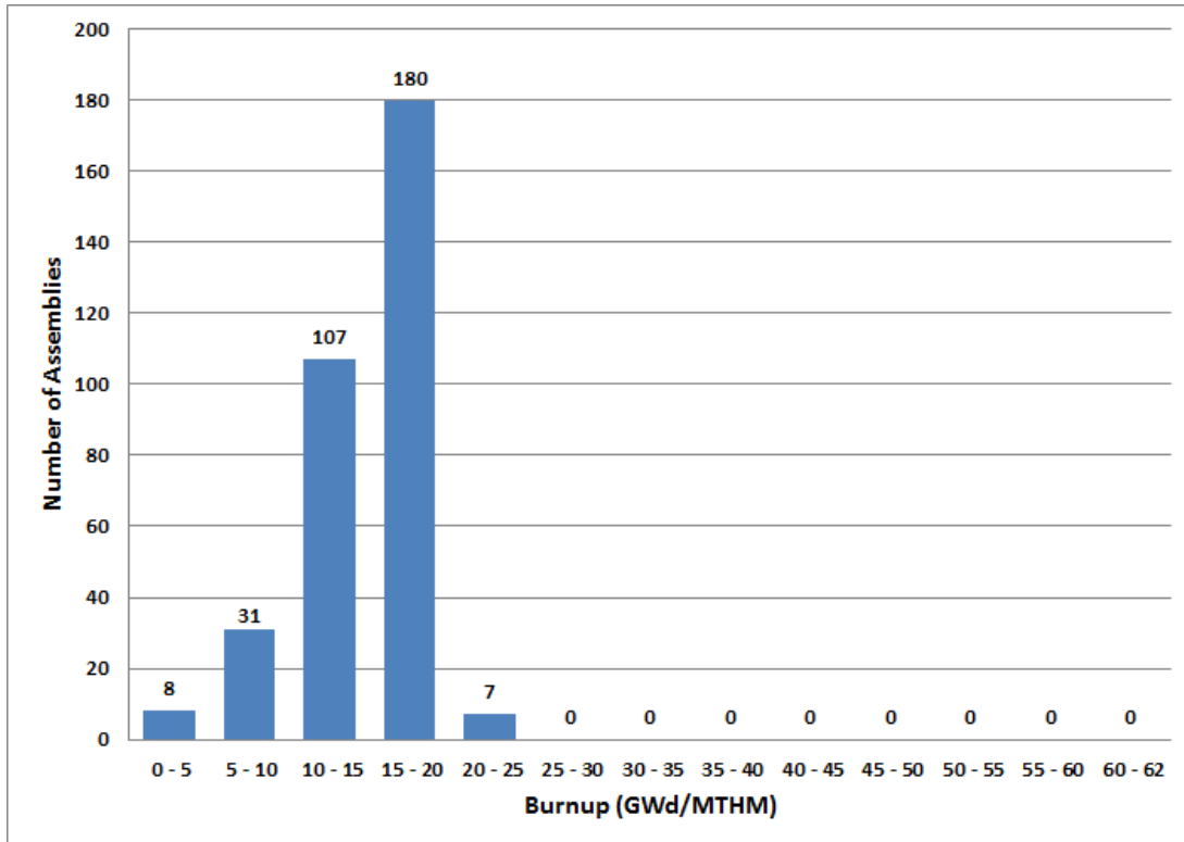
Figure 2-118. La Crosse Number of Assemblies versus Burnup (EIA 2013)
