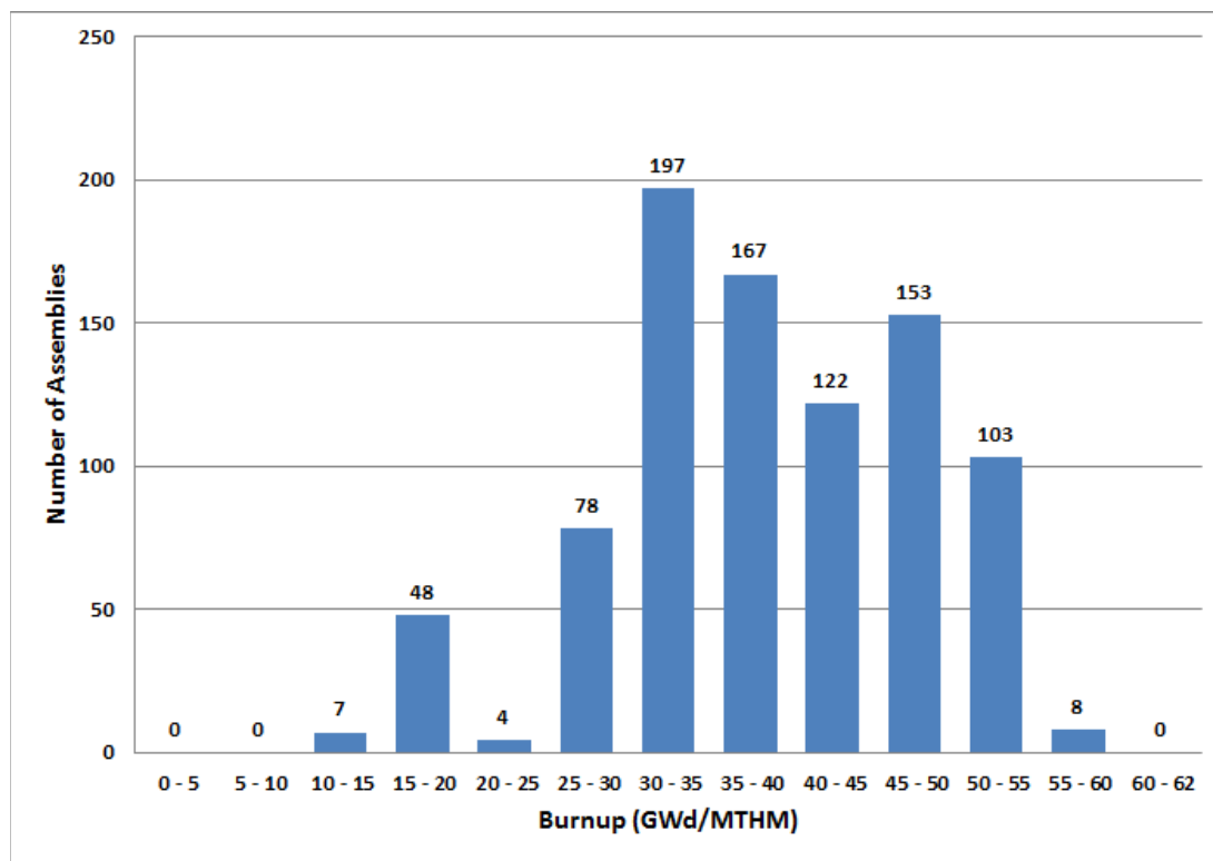
Figure 2-200. Kewaunee Number of Uncanistered Assemblies versus Burnup (EIA 2013)
