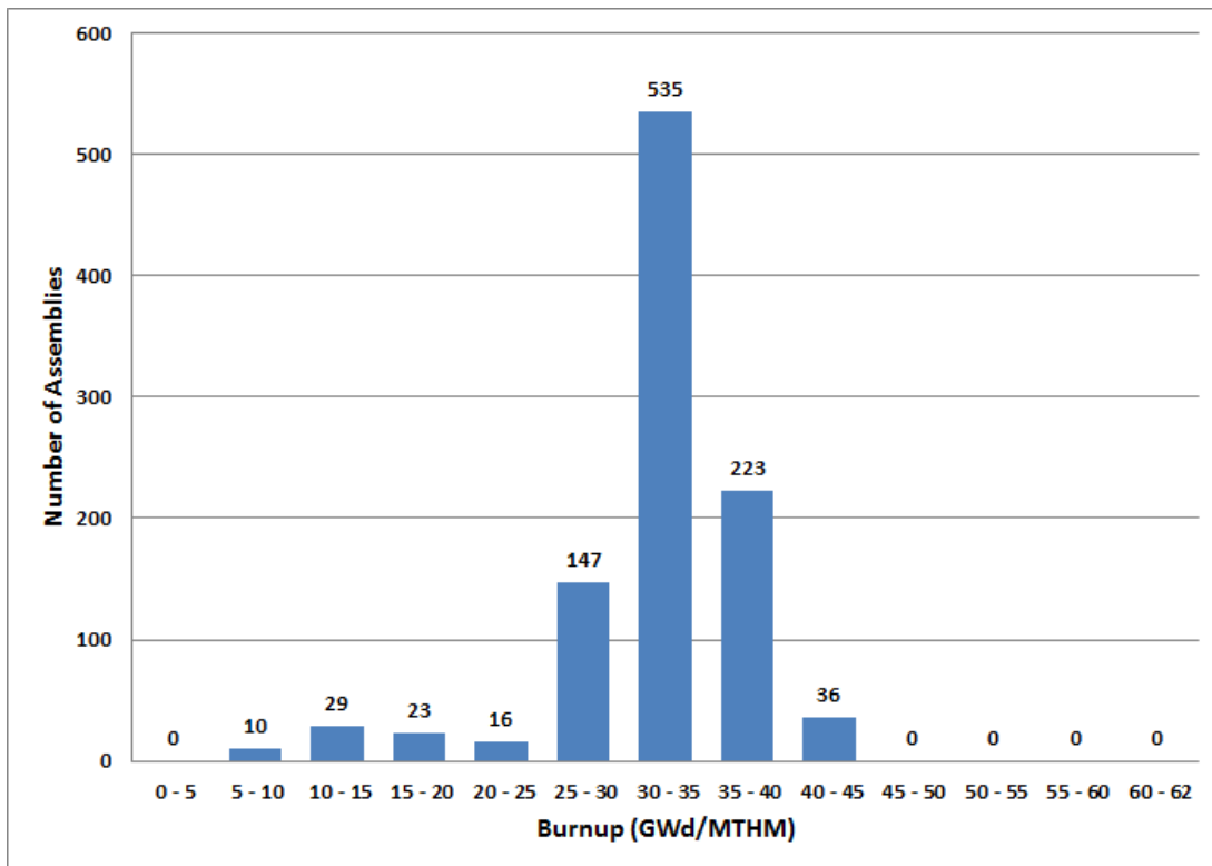
Figure 2-31. Connecticut Yankee Number of Assemblies versus Burnup (EIA 2013)
