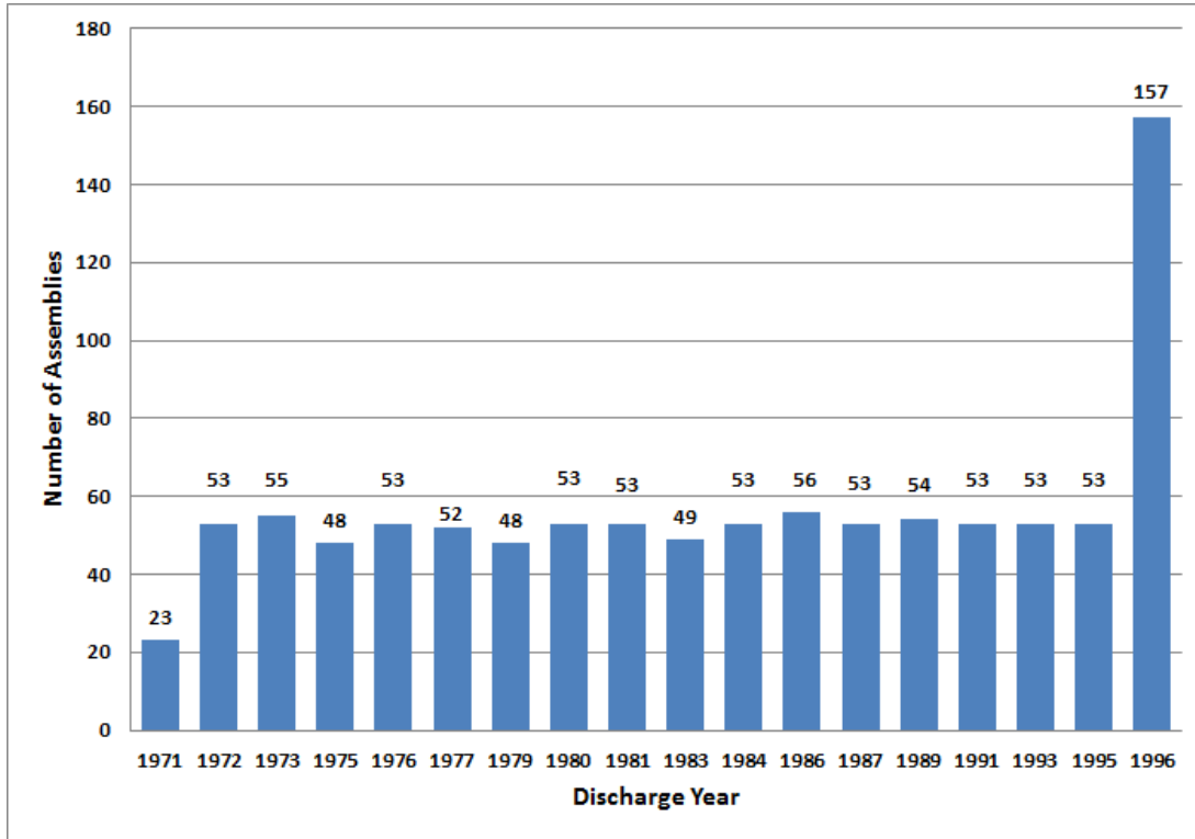
Figure 2-30. Connecticut Yankee Number of Assemblies versus Discharge Year (EIA 2013)
