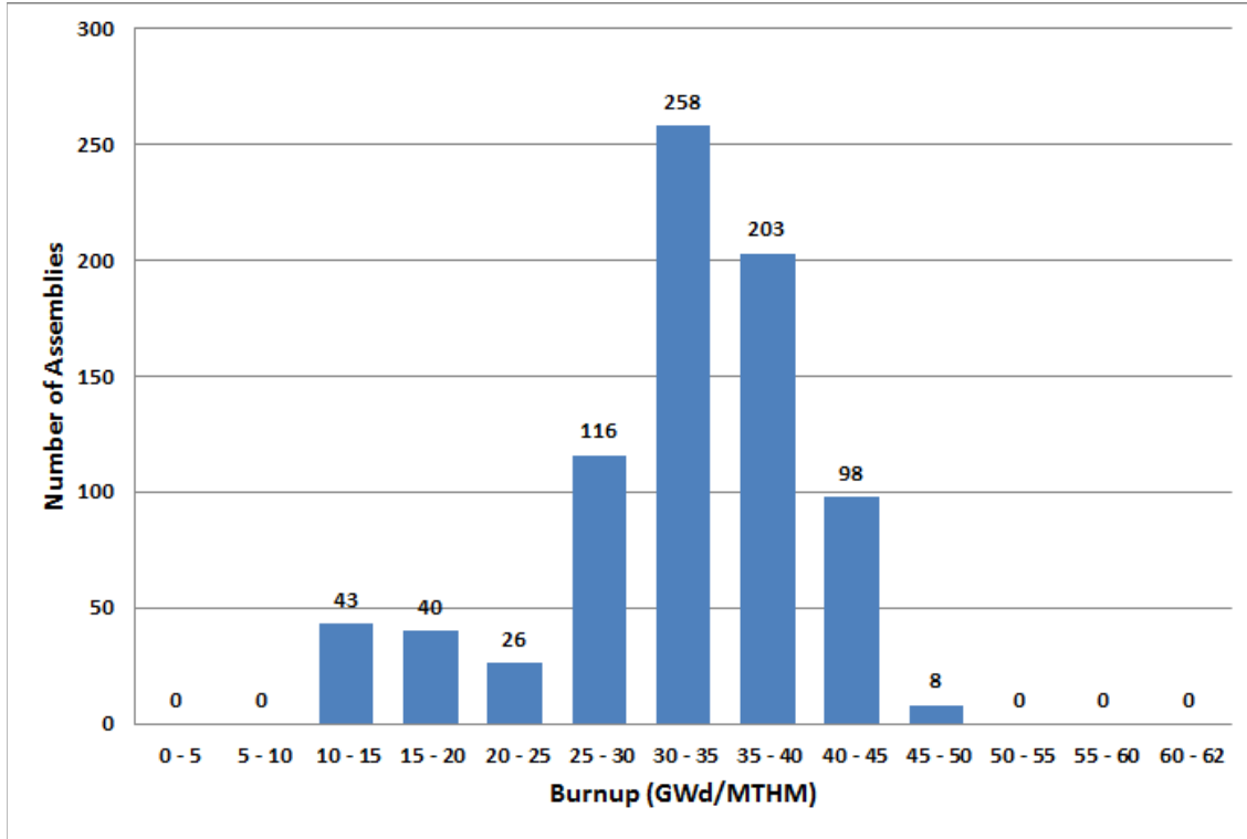
Figure 2-268. San Onofre-2 and -3 Number of Canistered Assemblies versus Burnup (EIA 2013)
