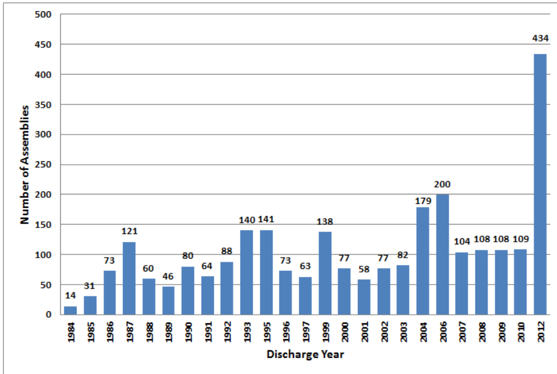
Figure 2-269. San Onofre-2 and -3 Number of Uncanistered Assemblies versus Discharge Year (EIA 2013)
