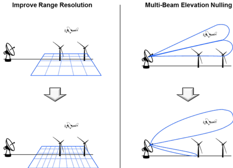
Figure 3. Examples of potential approaches to improve the performance of existing radars against wind turbines
