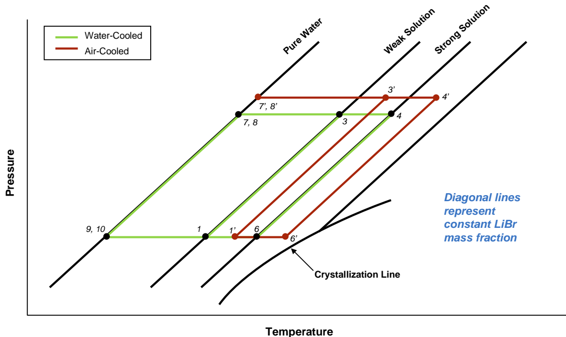
See Figure 1 for definition of state points. Adapted from Figure 20, ASHRAE Fundamentals Handbook [1].
