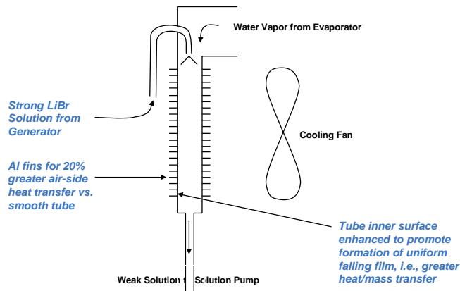
Figure 7: Vertical Falling-Film Absorber
