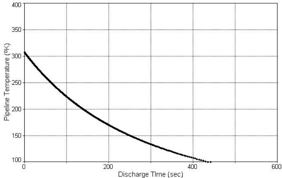
Temperature in CO 2 Pipeline Discharging To Atmosphere vs Time Pipeline: 10.31 inch ID; 5 mile segment; 308 °K; 850 kg/m 3 ; choked flow (without allowing for phase change)
