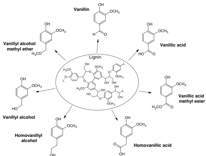
Figure A.2 - Potential Structures Available from Guaiacyl Units, Group 2
